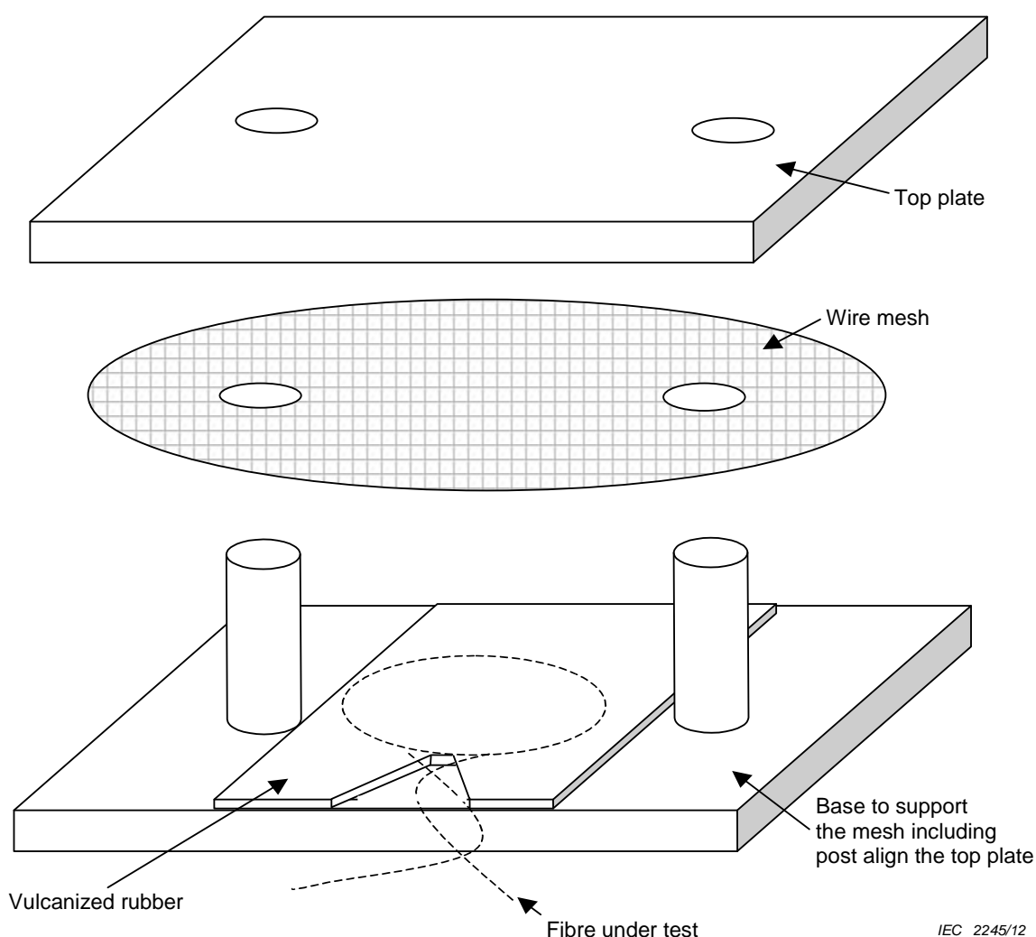
Figure 5 – Microbend-inducing equipment
