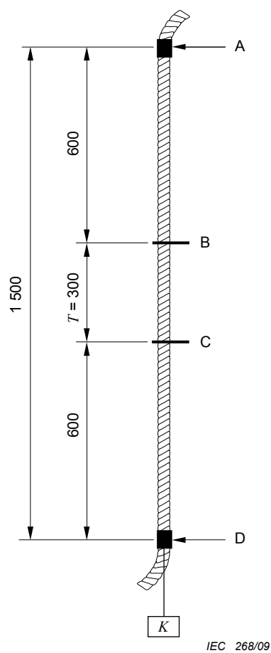
Figure 2a – Electrode arrangement for test before water conditioning
