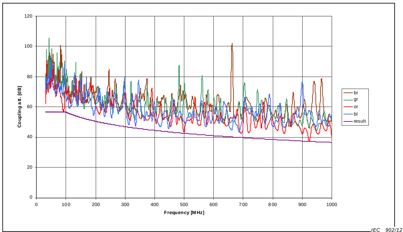
Figure 6 – Typical measurement of a screened balanced channel – Coupling attenuation, A is 57 dB
