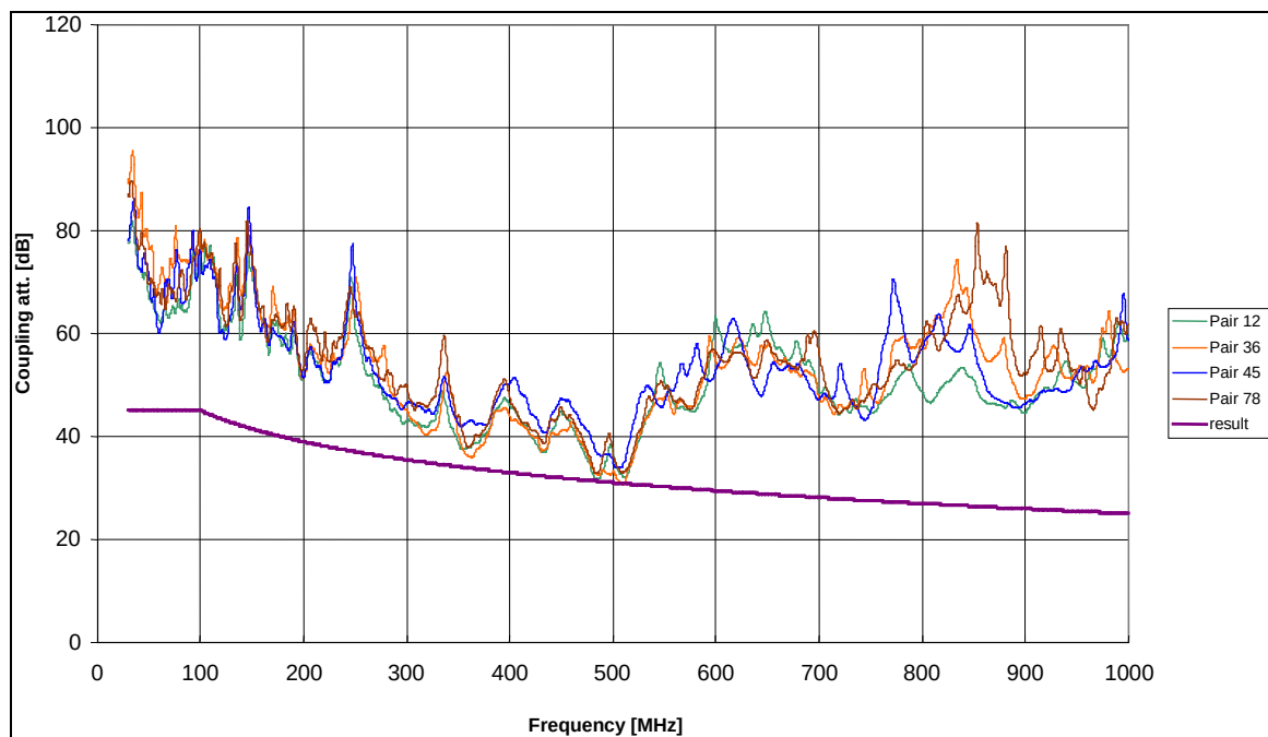
Figure 7 – Double wall outlet, right port (without connected screen) – Coupling attenuation, A is 44,8 dB
