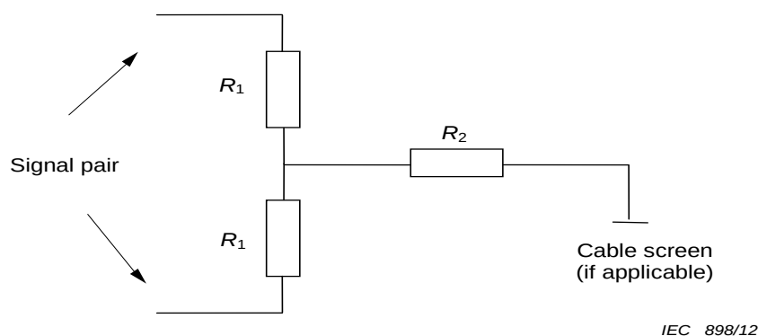
Figure 2 – Termination of link or channel or applied extension cable
