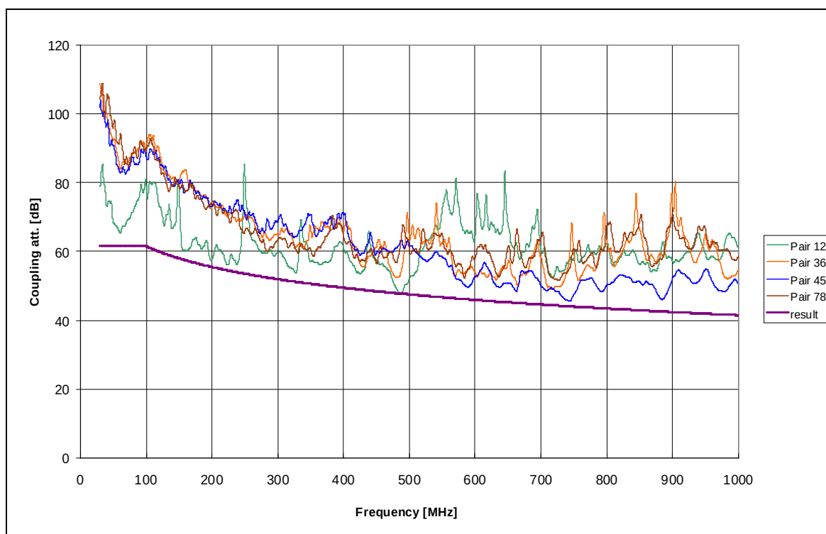
Figure 8 – Double wall outlet, left port (with connected screen) – Coupling attenuation, A is 61,5 dB
