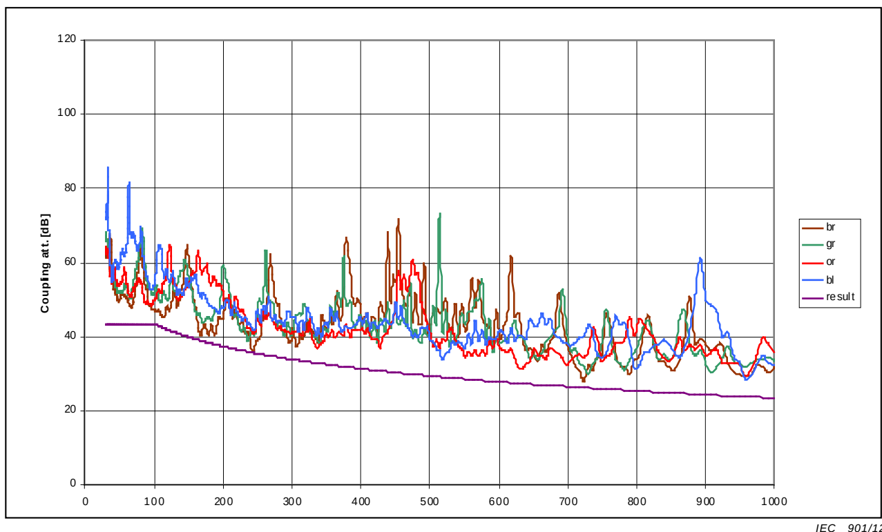
Figure 5 – Typical measurement of an unscreened channel – Coupling attenuation, A is 43 dB
