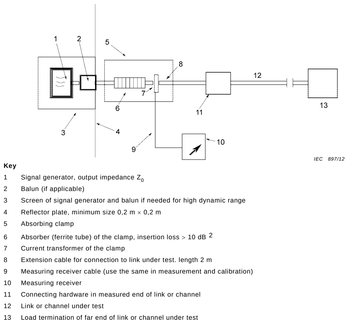
Figure 1 – Measurement of surface wave at one end of a link or channel
