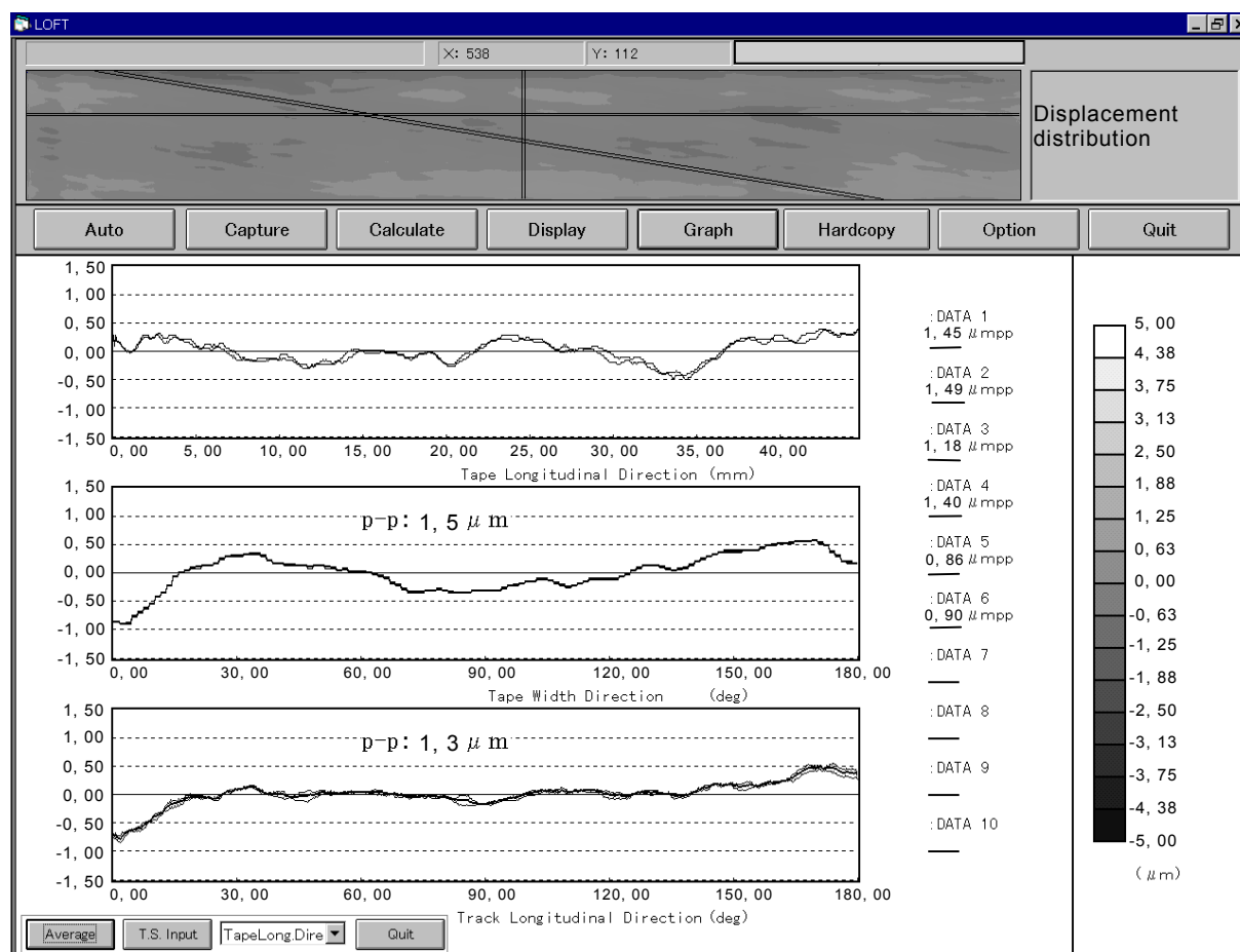
Figure 12 – Example of calculation results
