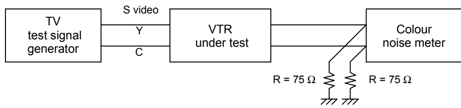
Figure 25 – Block diagram for S video input
