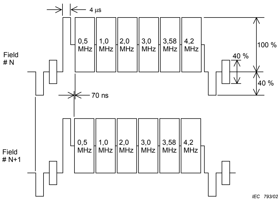
Figure 29 – Test signal for 3D chrominance signal separation
