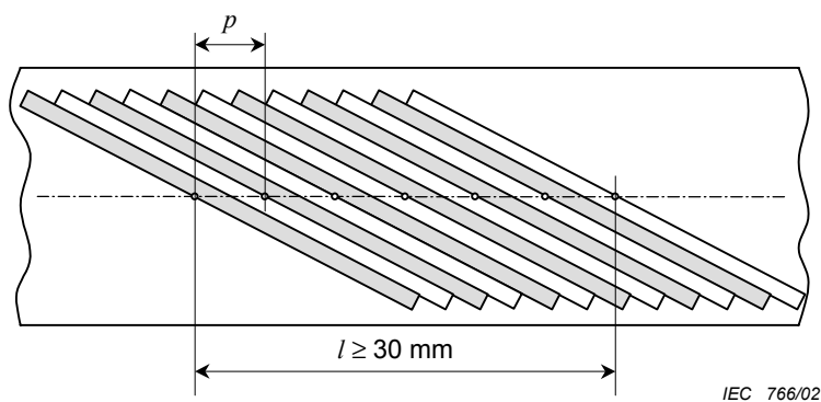
Figure 2 – Measuring method for track interval
