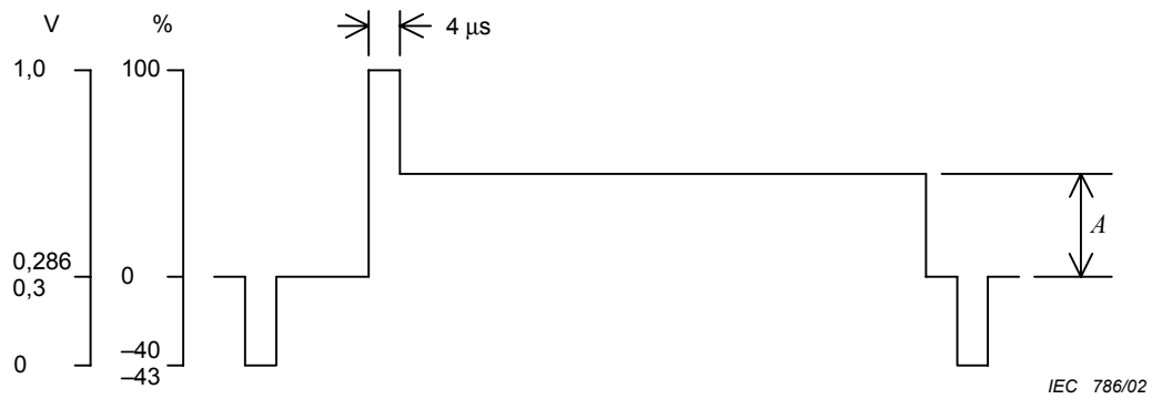
Figure 21 – Composite video test signal for luminance signal-to-noise ratio
