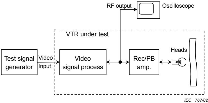
Figure 3 – Measuring block diagram for RF envelope flatness
