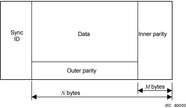
Figure A.1 – Structure of data-synchronization blocks
