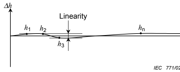
Figure 7 – Measuring method for linearity
