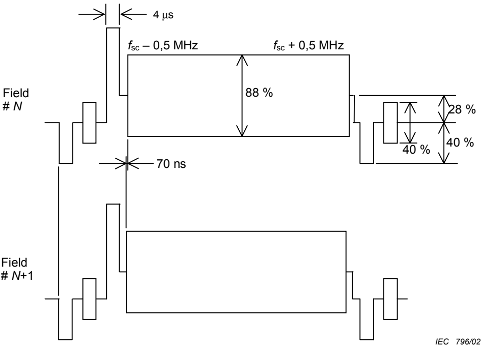
Figure 32 – Test signal for 3D luminance signal separation
