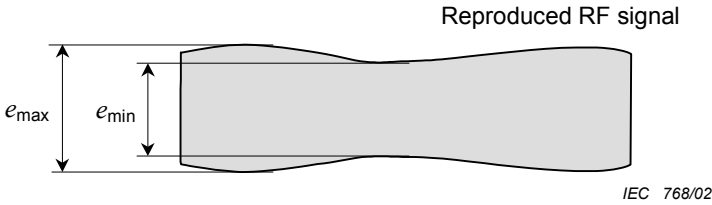
Figure 4 – Measuring method for RF envelope flatness
