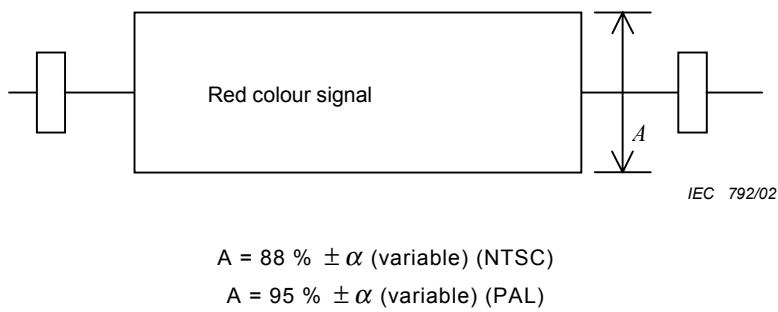
Figure 28 – S chrominance test signal for chrominance signal-to-noise ratio
