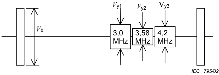
Figure 31 – Measuring method for 3D chrominance signal separation
