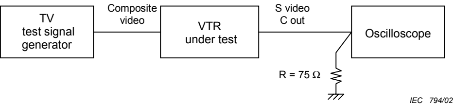
Figure 30 – Measuring block diagram for chrominance signal separation
