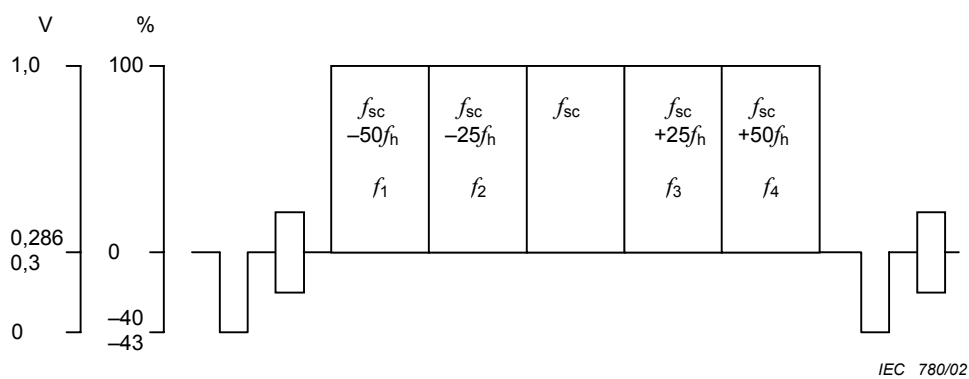
Figure 16 – Test signal for chrominance amplitude frequency response
