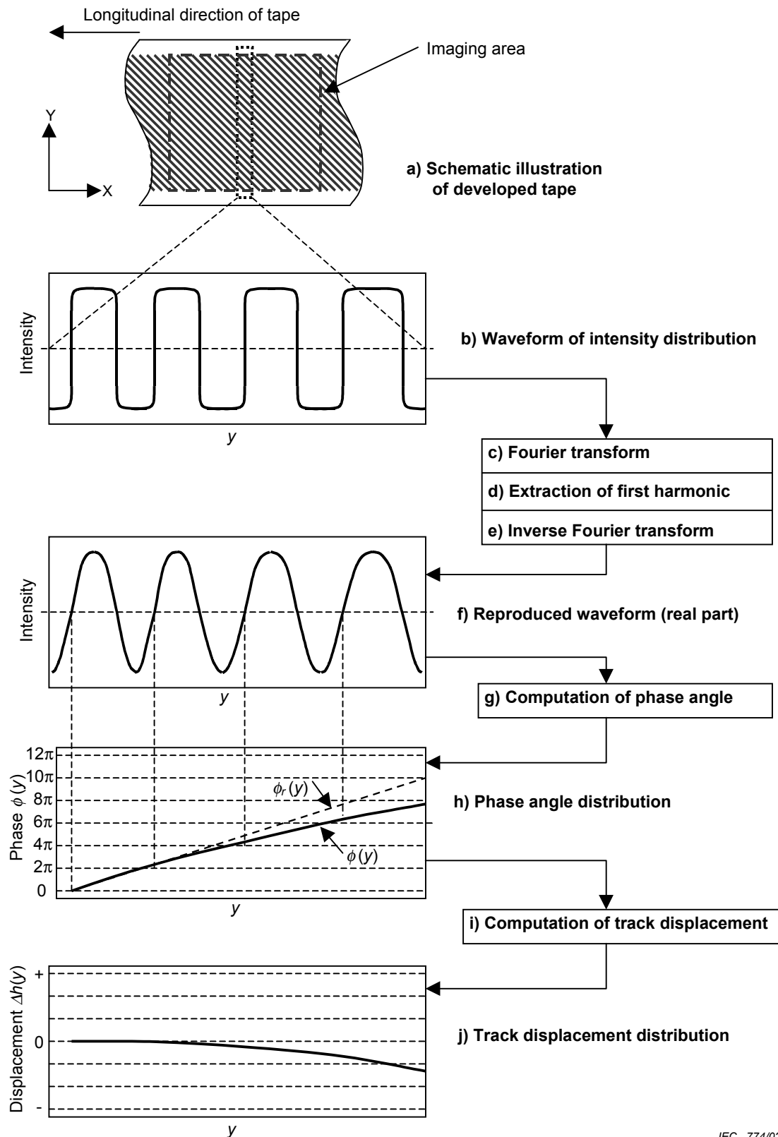
Figure 10 – Schematic diagram of the image processing technique
