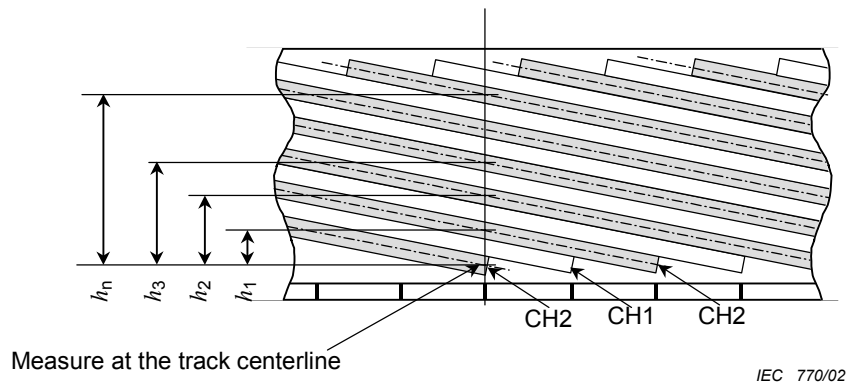
Figure 6 – Cross-tape track height for D-VHS format
