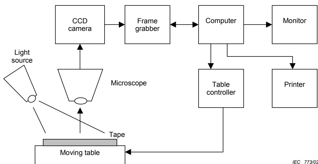
Figure 9 – Block diagram of the measurement system
