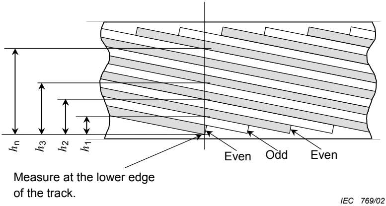
Figure 5 – Cross-tape track height for DV format
