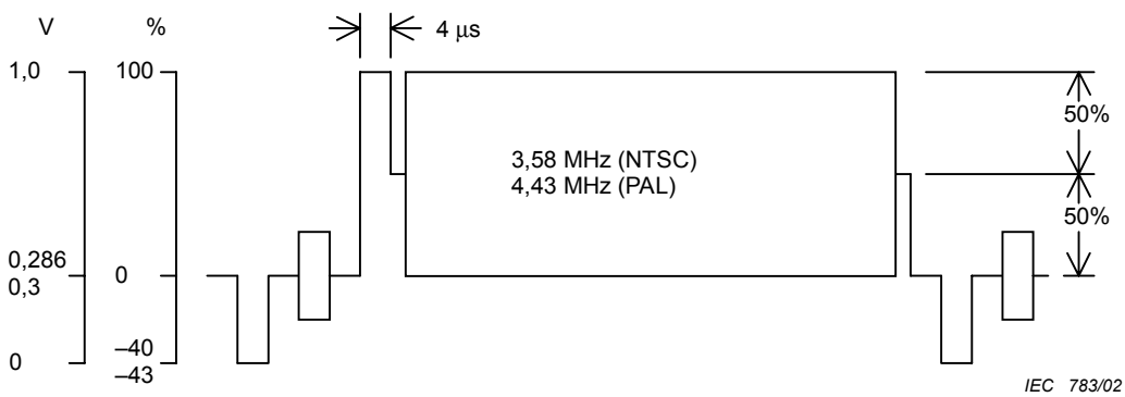
Figure 19 – Test signal for chrominance waveform distortion
