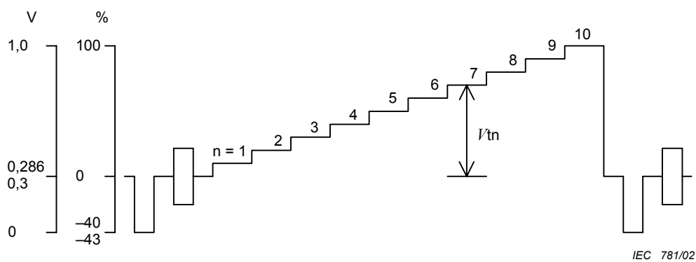
Figure 17 – Test signal for luminance non-linear distortion
