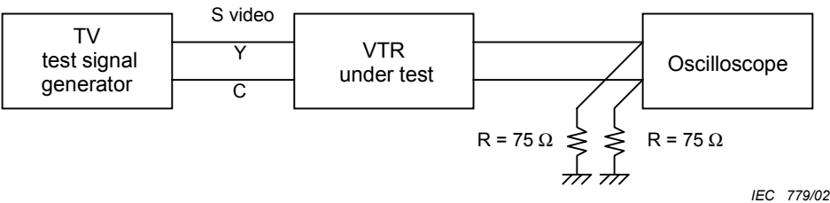
Figure 15 – Measuring block diagram for S video signal
