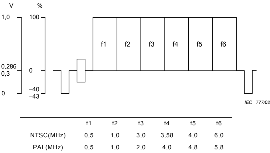
Figure 13 – Test signal for luminance amplitude frequency response
