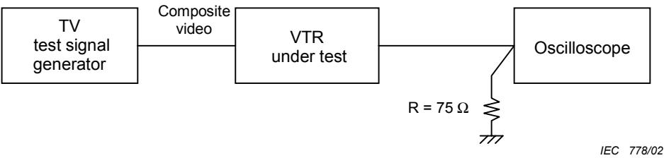
Figure 14 – Measuring block diagram for composite video signal
