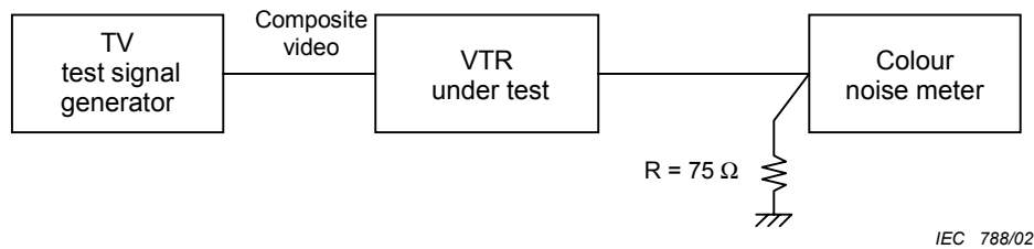
Figure 24 – Block diagram for composite video input
