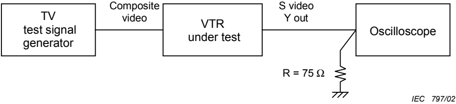
Figure 33 – Measuring block diagram for luminance signal separation
