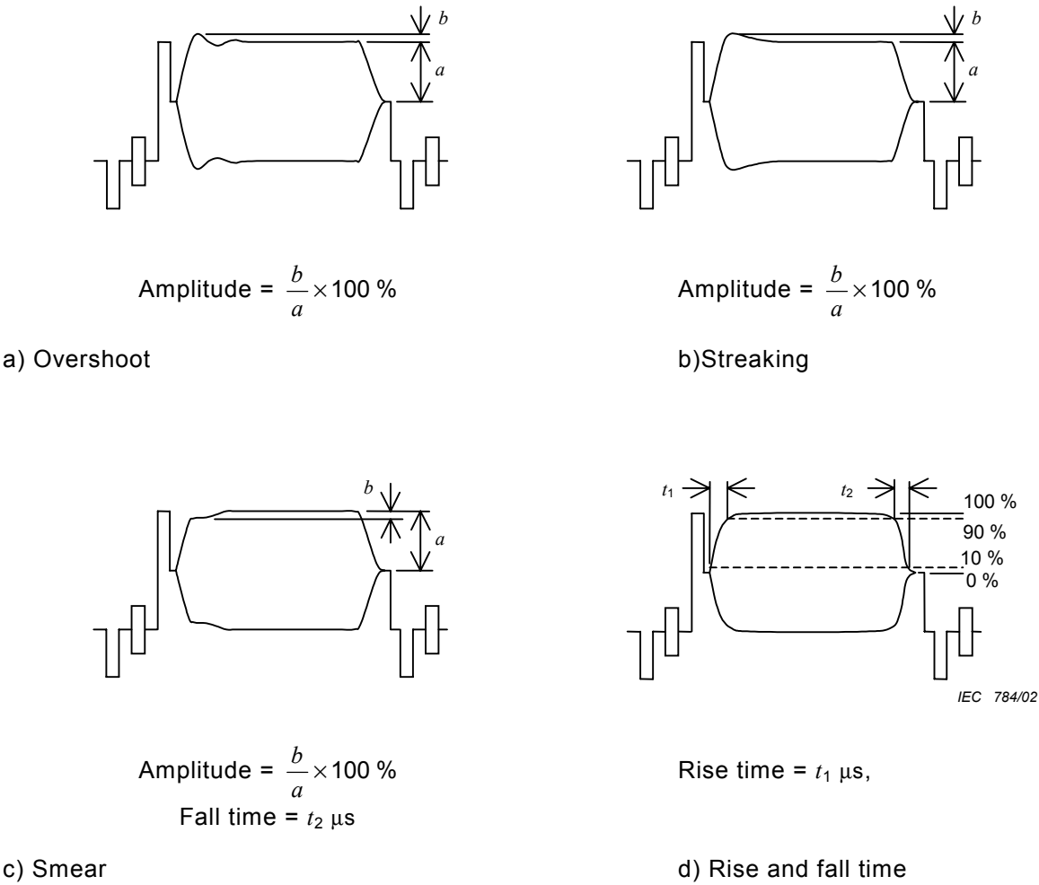
Figure 20 – Measuring method for chrominance waveform distortion
