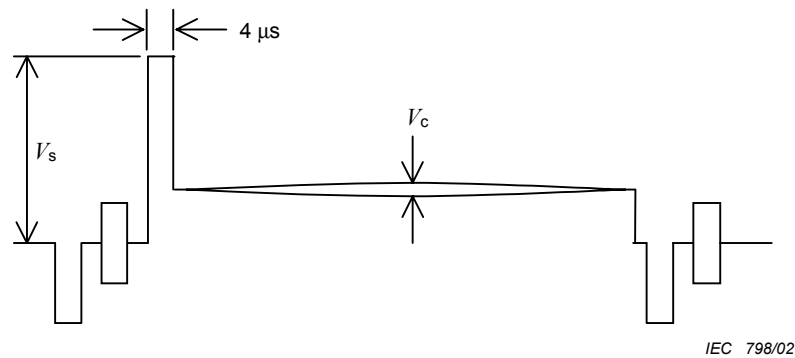
Figure 34 – Measuring method for 3D luminance signal separation
