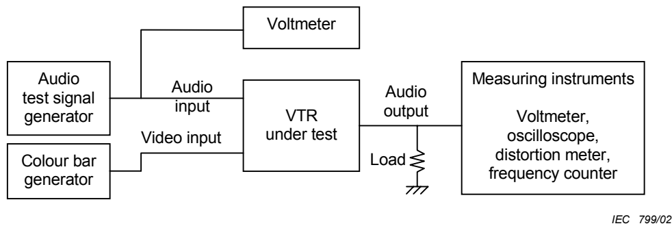
Figure 35 – Block diagram for audio characteristics
