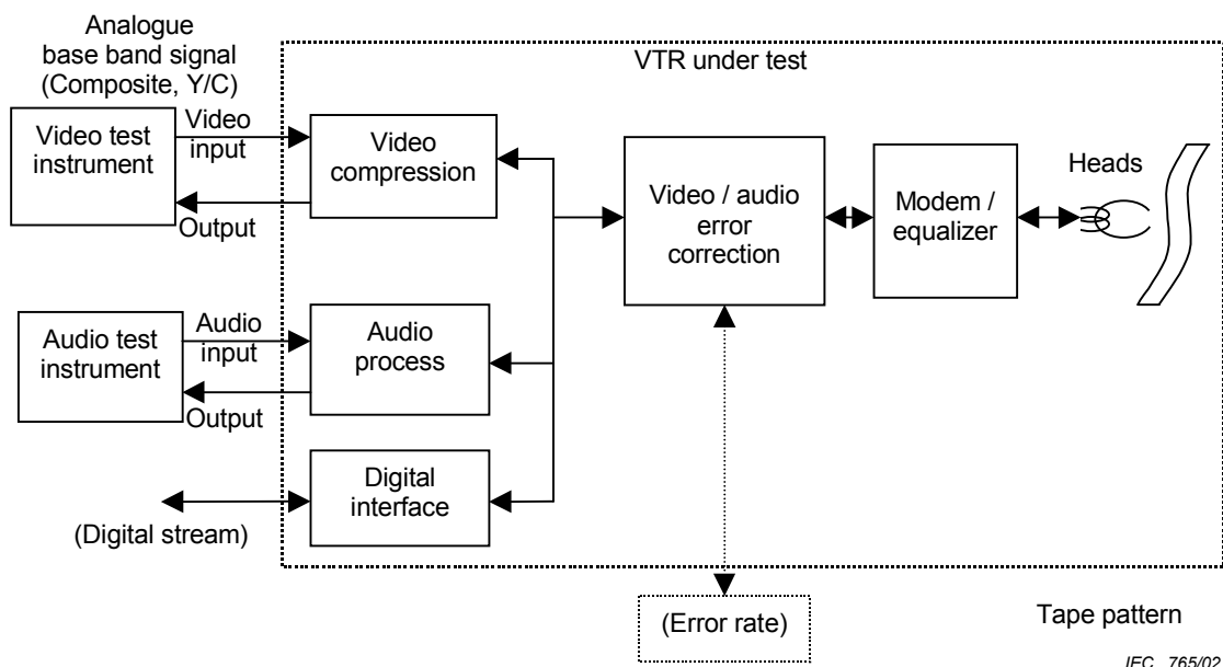
Figure 1 – Basic block diagram of measurement system
