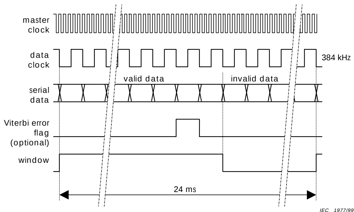
Figure A.1 – Logic signals of DAB 3 interface
