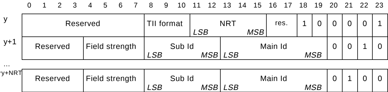
Figure 8 – Basic format for TII data (TII format = 010)
