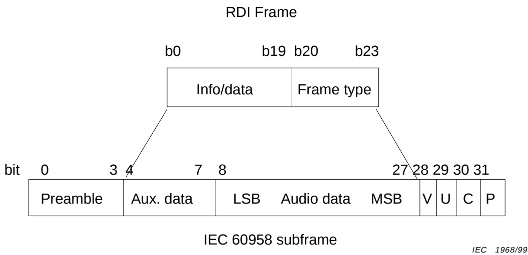
Figure 3 – Embedding RDI frames into IEC 60958 subframes
