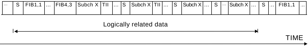
Figure 10 – Order of transmission on RDI (Examples)
