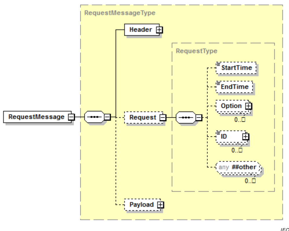
Figure 19 – RequestMessage structure
