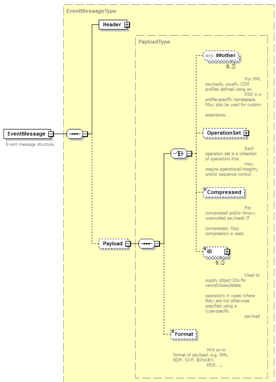
Figure 23 – EventMessage structure
