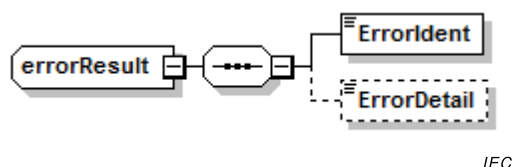
Figure 14 – errorResult substructure
