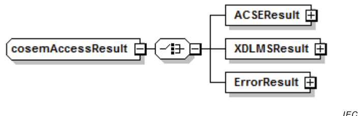
Figure 13 – cosemAccessResult substructure
