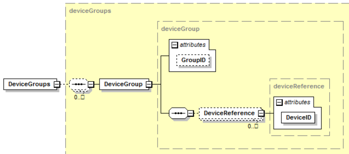
Figure 9 – DeviceGroups structure
