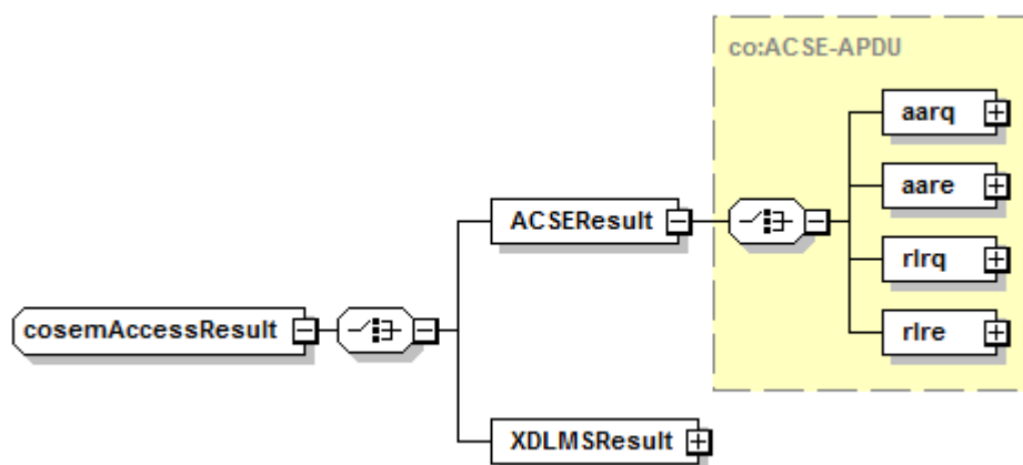
Figure 15 – ACSEResult substructure
