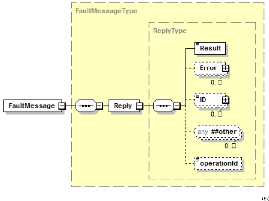
Figure 25 – FaultMessage structure
