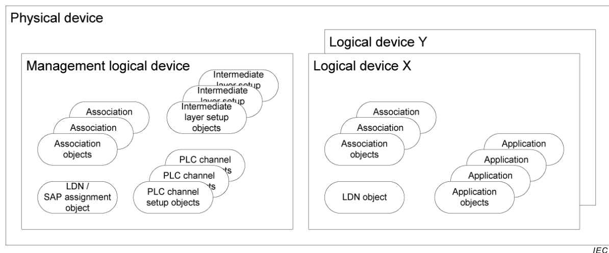
Figure 16 – Object model of DLMS/COSEM servers
