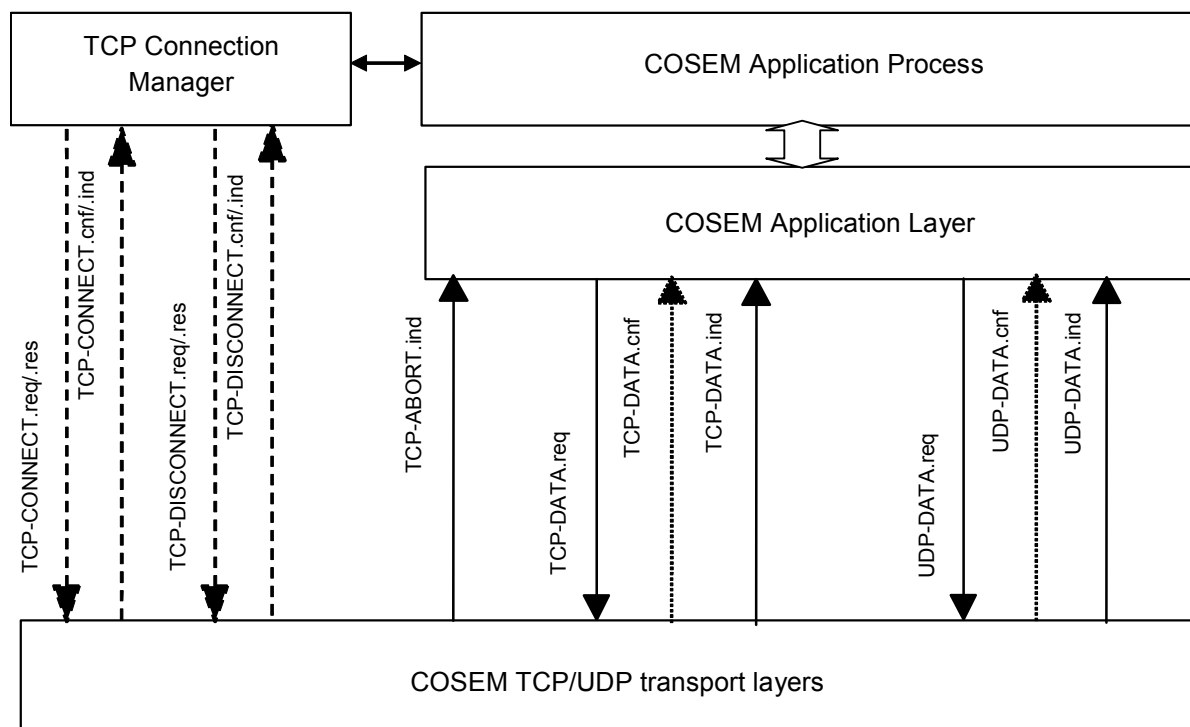
Figure B.10 – Summary of TCP/UDP layer services on the client and server side
