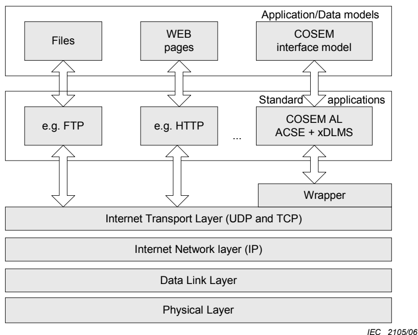
Figure B.7 – COSEM as a standard Internet application protocol
