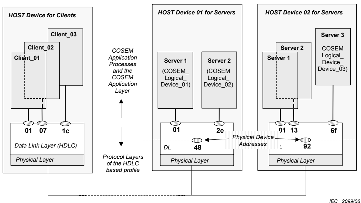
Figure B.1 – Identification/addressing scheme in the 3-layer, connection-oriented, HDLC based communication profile
