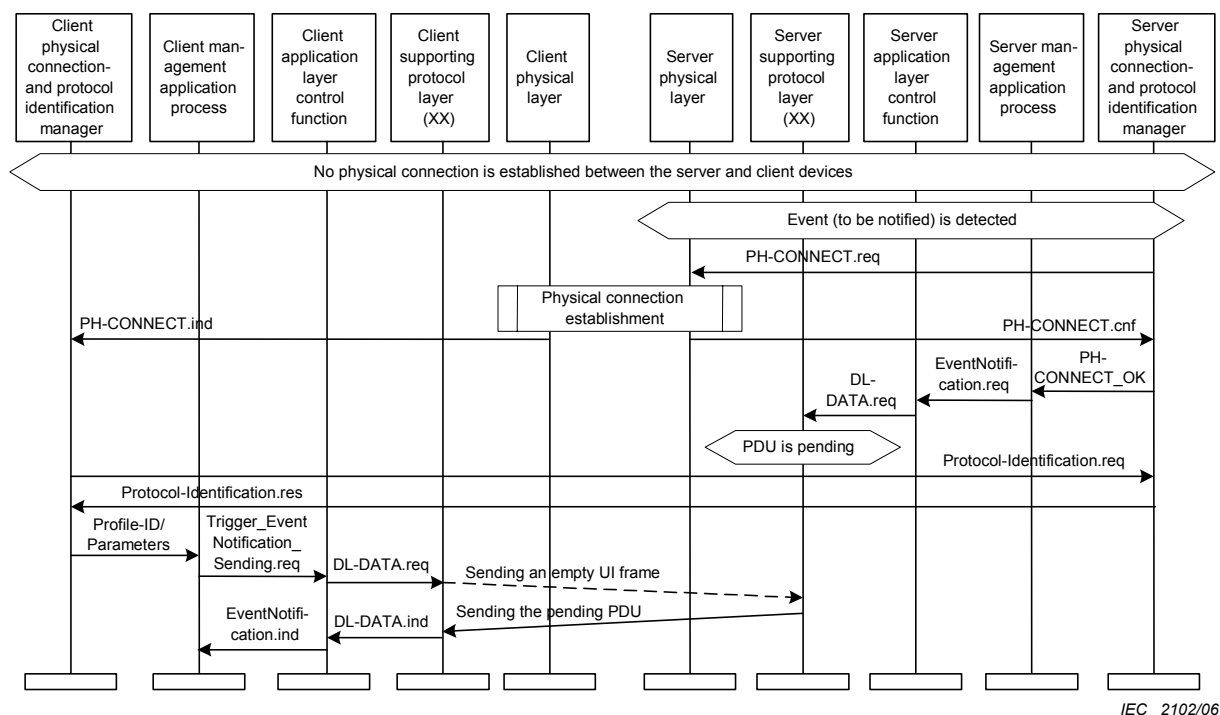
Figure B.4 – Example: EventNotificaton triggered by the client
