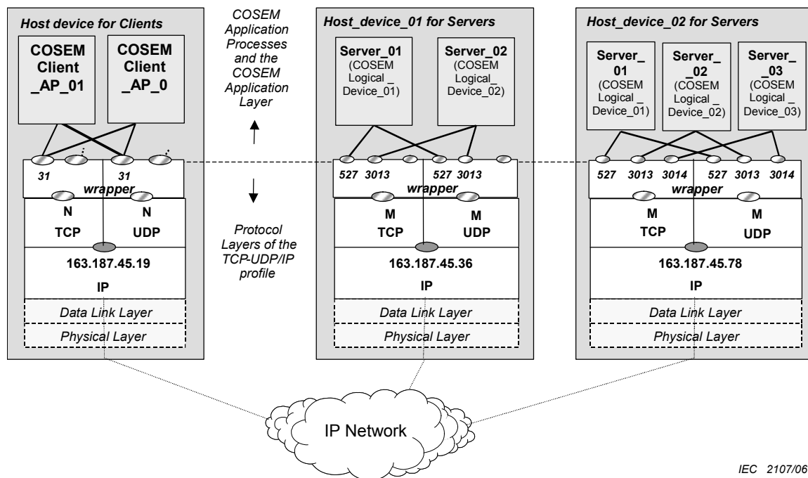
Figure B.9 – Identification/addressing scheme in the TCP-UDP/IP based profile(s)
