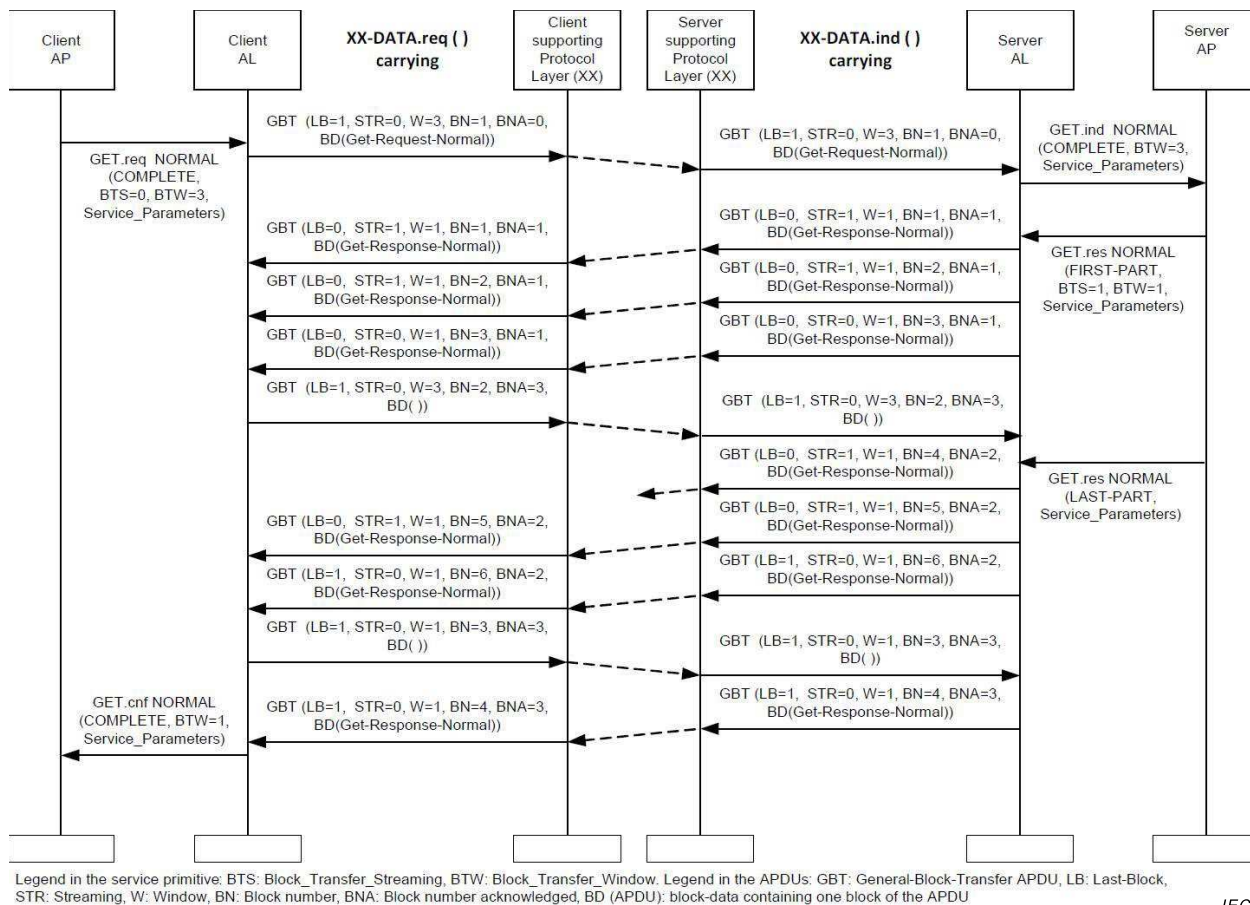
Figure 32 – GET service with partial invocations, GBT and streaming, recovery of 4 th block sent in the 2 nd stream
