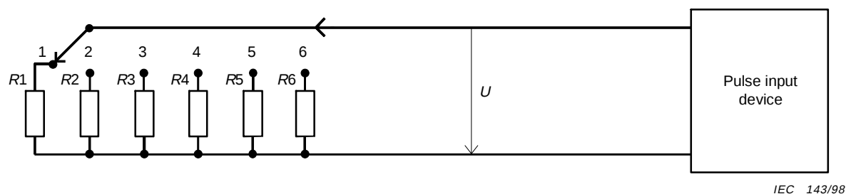
Figure E.3 – Pulse input device test set-up
