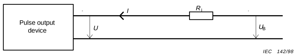
Figure E.2 – Pulse output device test set-up
