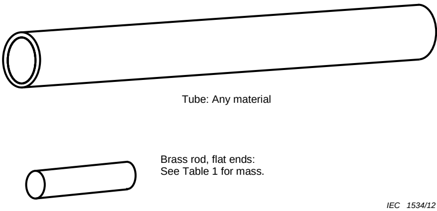
Figure 2 – Impact device
