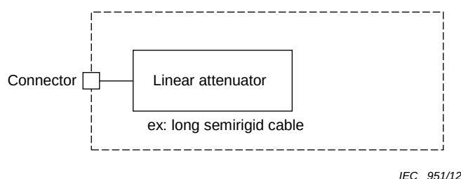
Figure A.1 – Long cable termination
