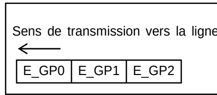
Figure 23 – Bloc “Groupe”
