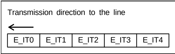
Figure 24 – Item block
