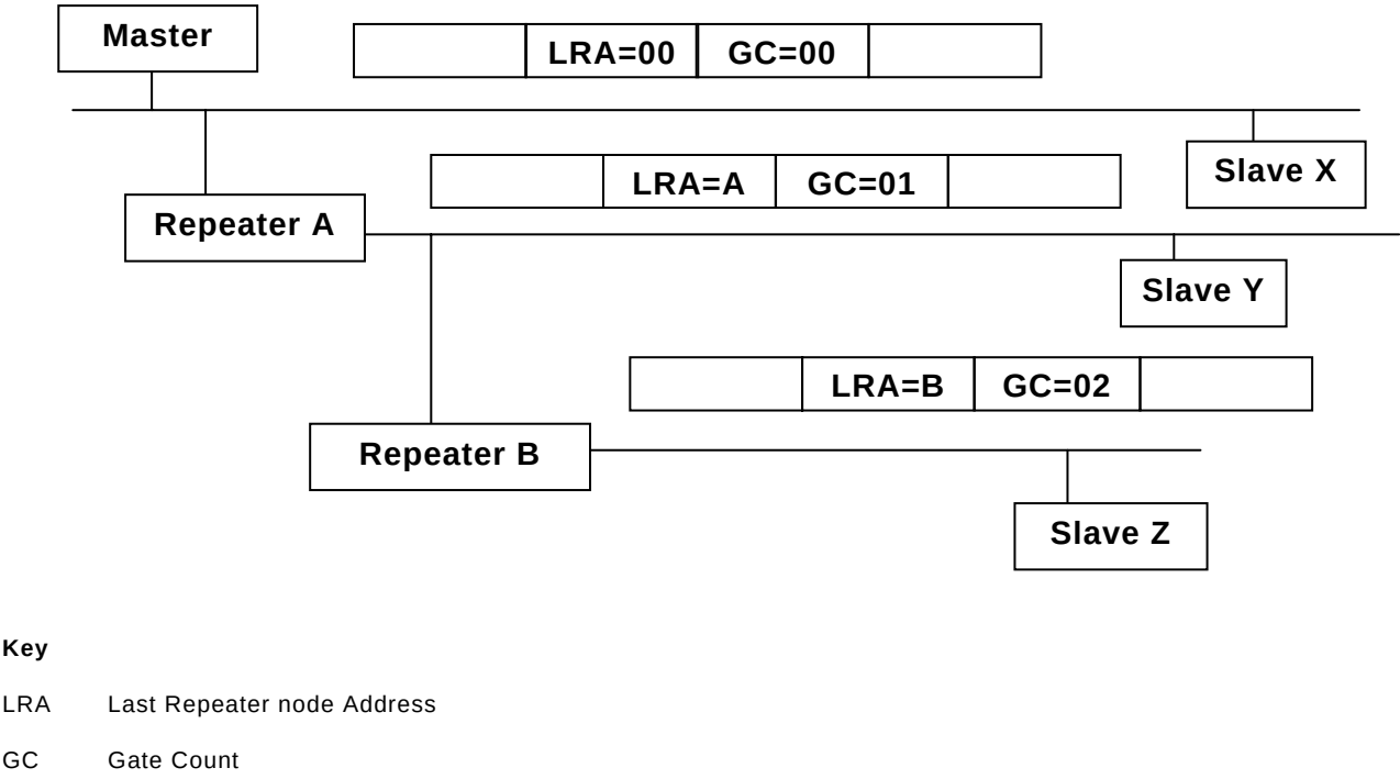
Figure 52 – BEACON changed by repeaters
