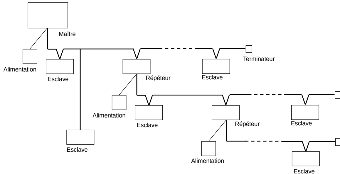
Figure 2 – Composants CompoNet
