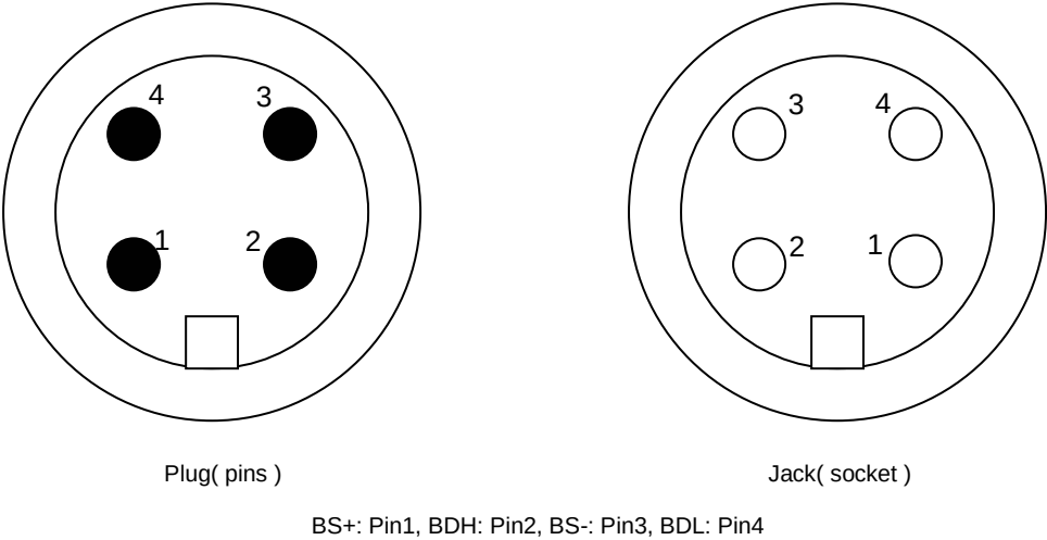
Figure 115 – M12 connector pinout
