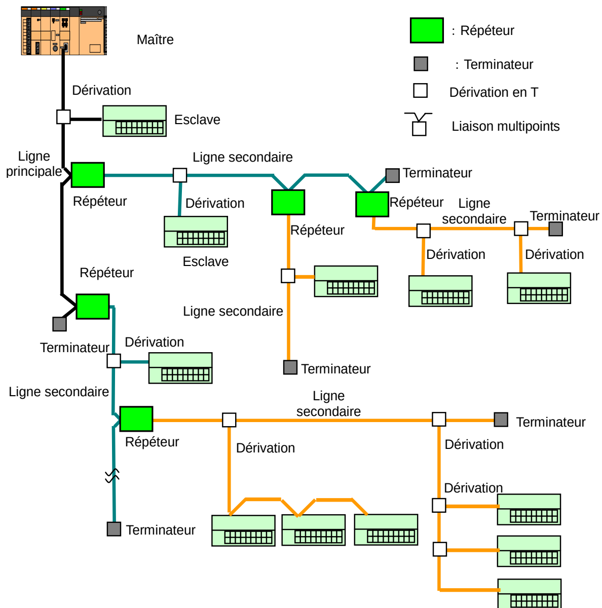
Figure 83 – Topologie des supports
