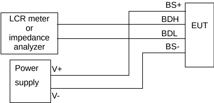
Figure 122 – Input impedance
