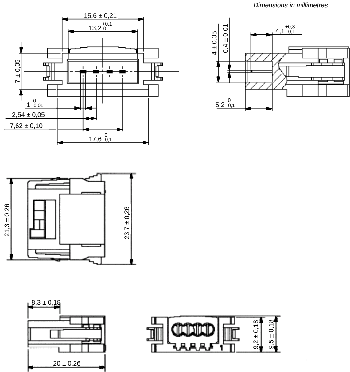
Figure 109 – Flat connector I plug
