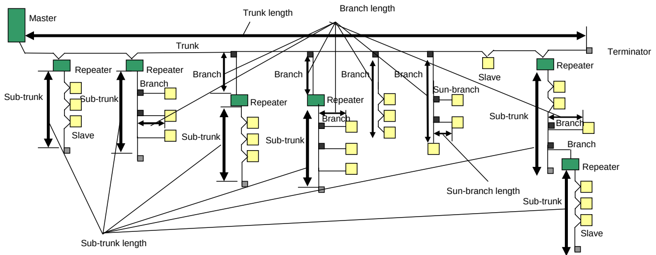
Figure 86 – Cable length limitation Illustration
