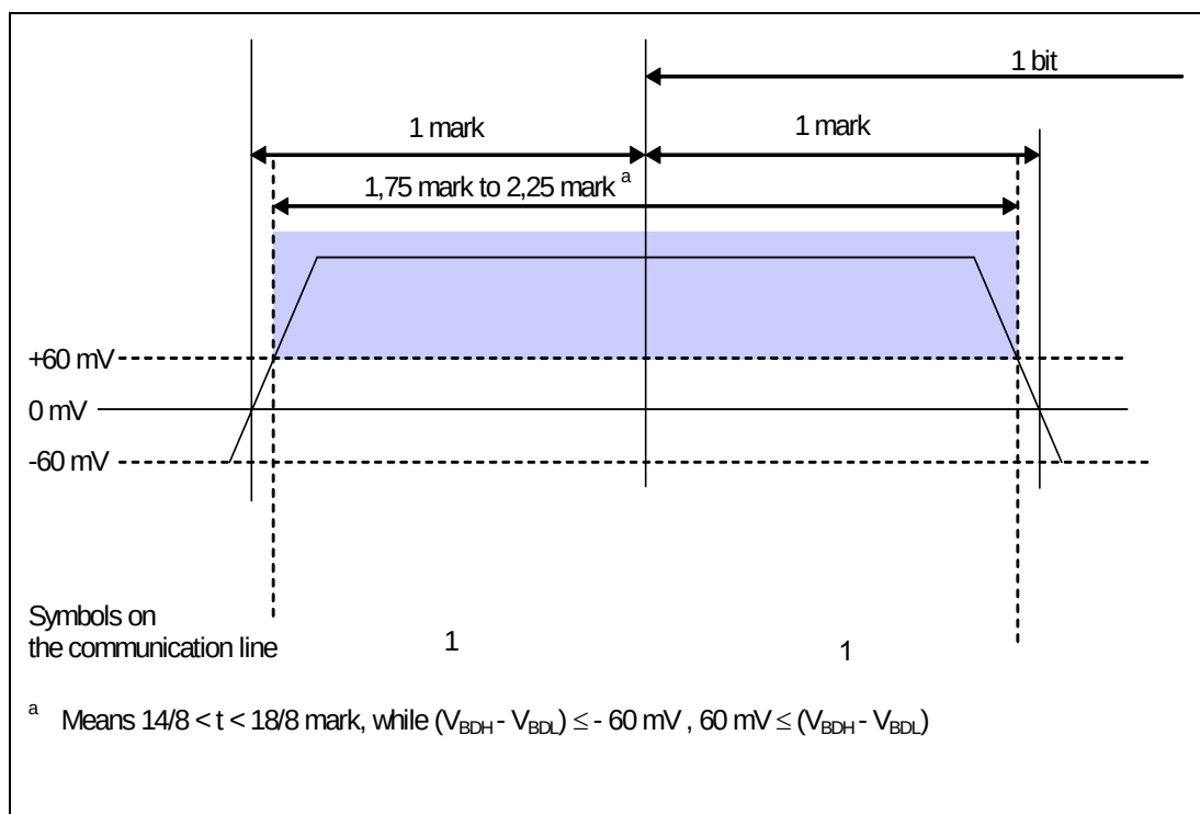
Figure 67 – Receive mask 2
