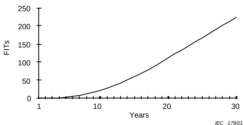
Figure 6 – Component reliability in service
