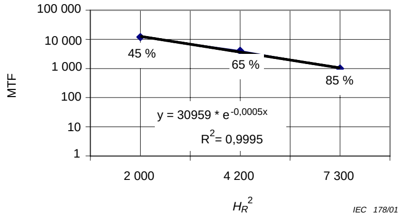
Figure 5 – Exponential curve fit for MTF versus H_R^2
