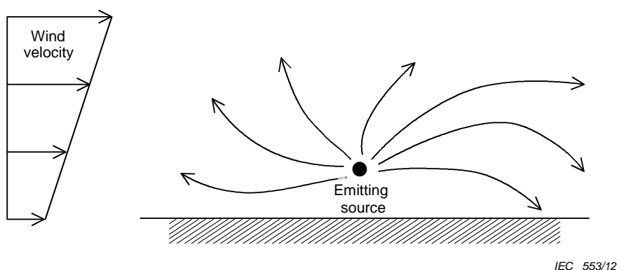
Figure 6 – Example of sound refraction with the shown wind gradient
