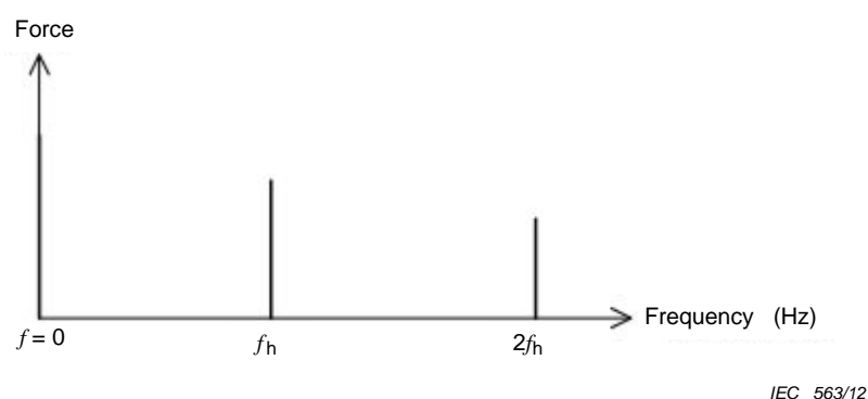
Figure 16 – Example of spectrum of forces acting on the reactor winding
