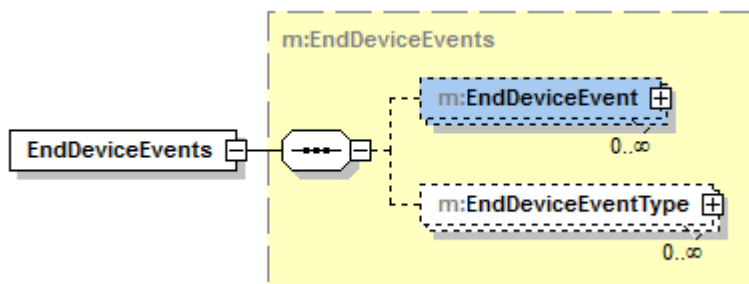
Figure 48 – EndDeviceEvents definition
