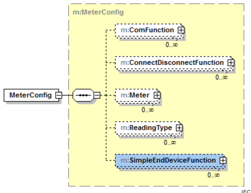
Figure 53 – MeterConfig definition
