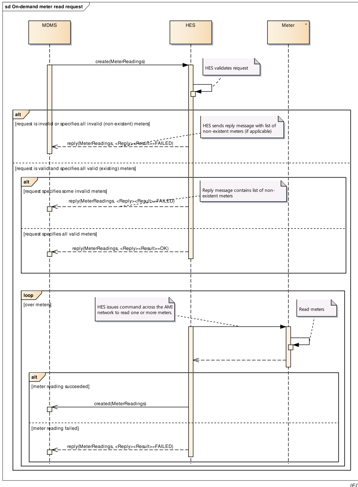
Figure 24 – Message exchange pattern for an on-demand meter read
