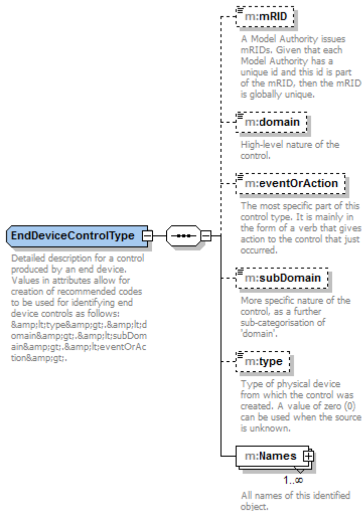
Figure 45 – EndDeviceControlType definition
