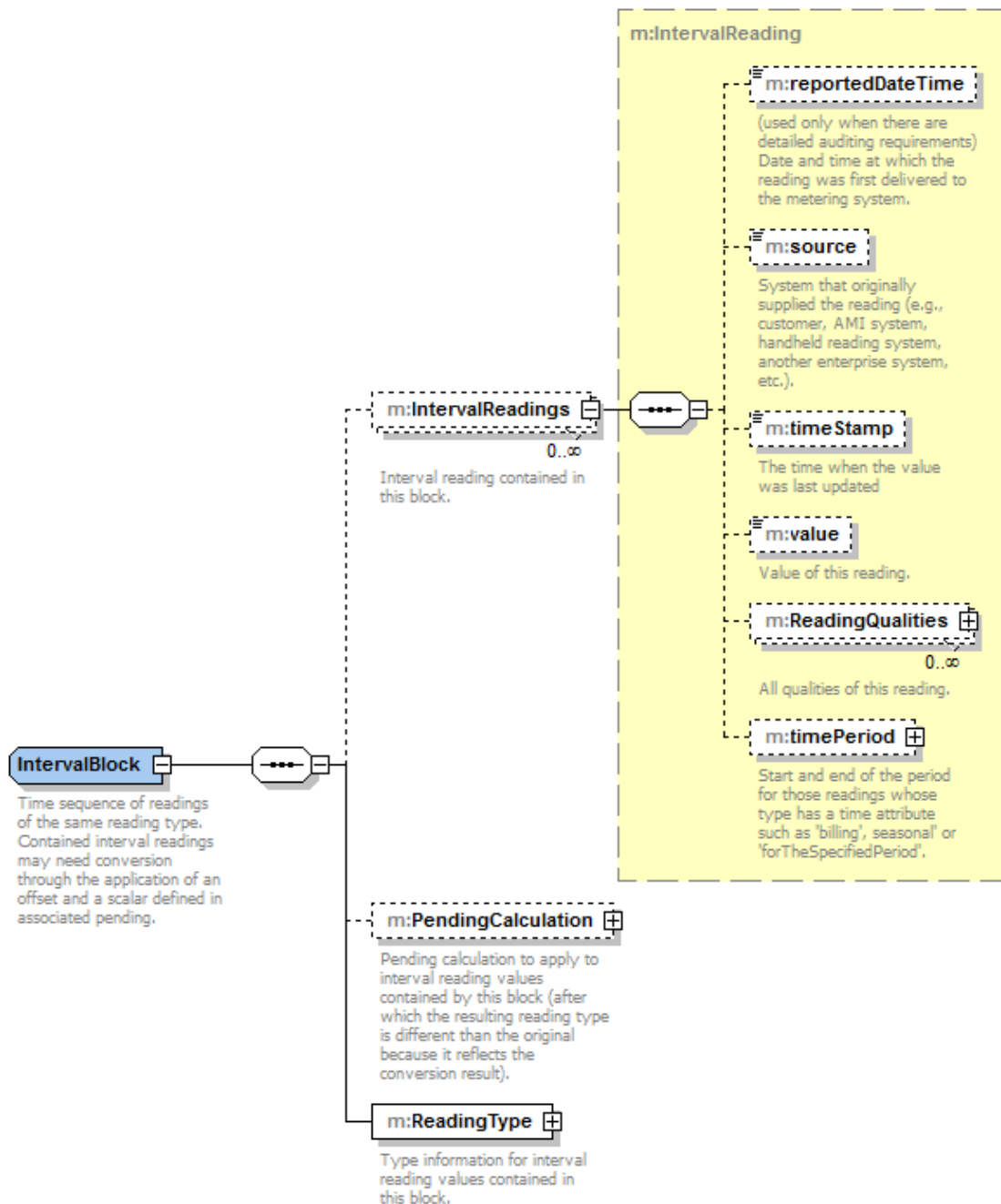
Figure 31 – <MeterReadings><IntervalBlock> definition
