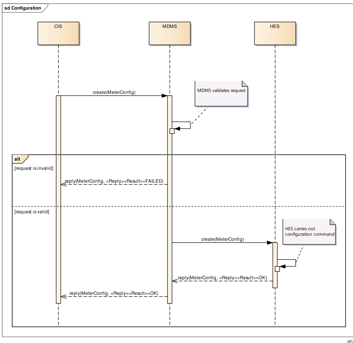
Figure 52 – Message exchange pattern for a create(MeterConfig) message
