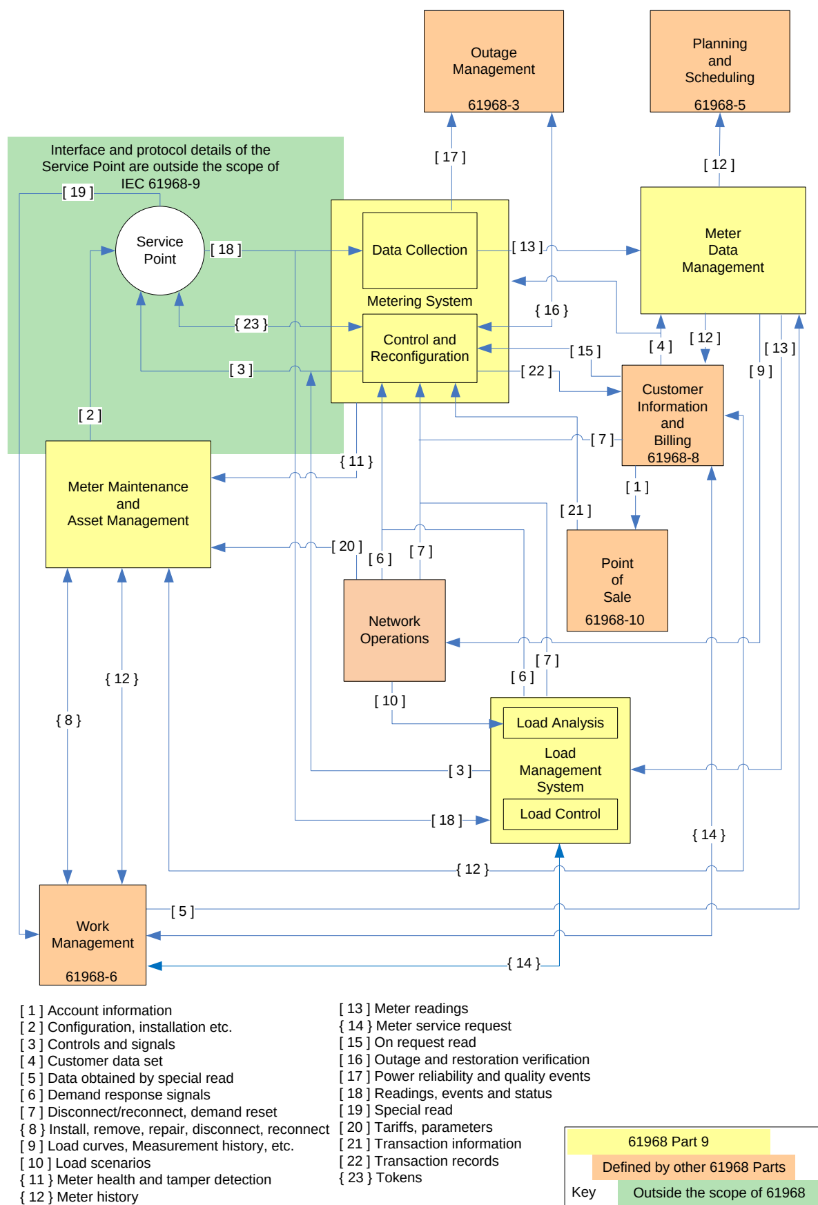
Figure 3 – IEC 6168-9 reference model
