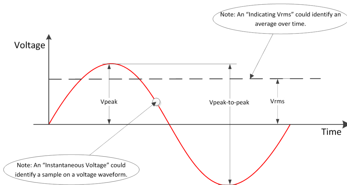
Figure C.3 – Voltage measurements
