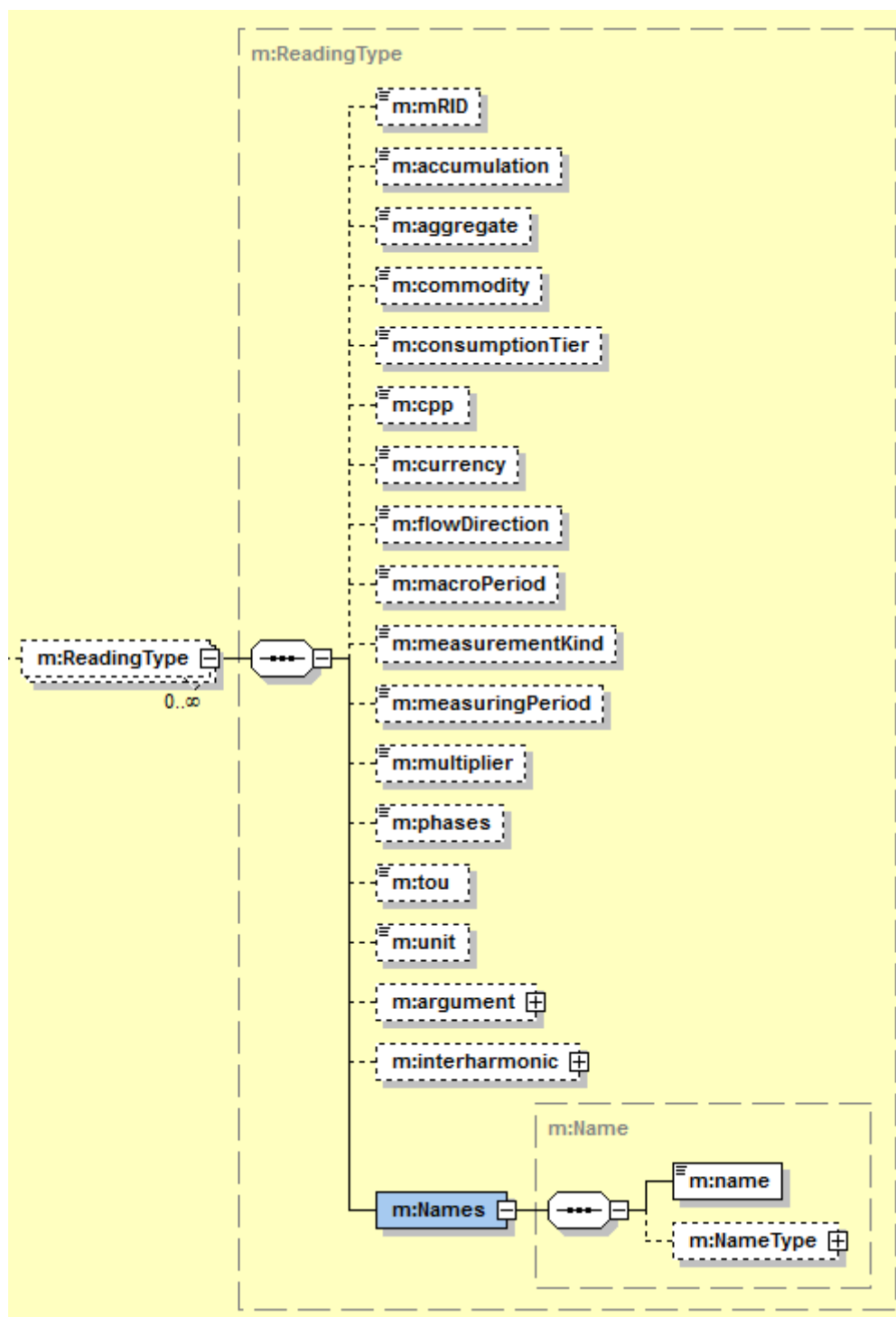
Figure 26 – Structure ReadingType
