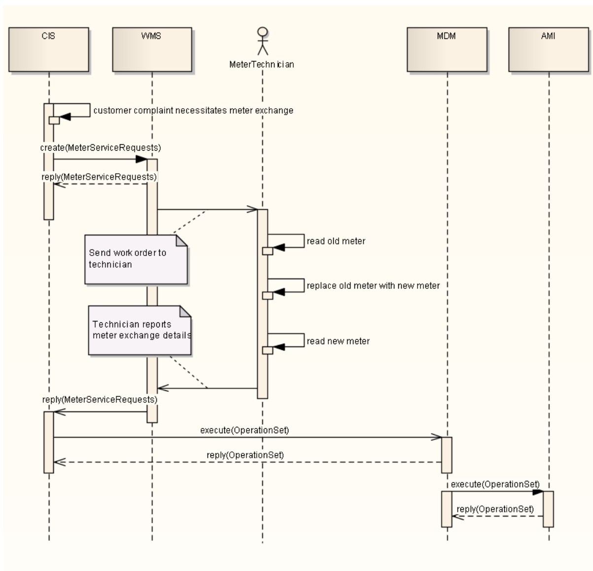
Figure 39 – Example message exchange due to CIS alarms
