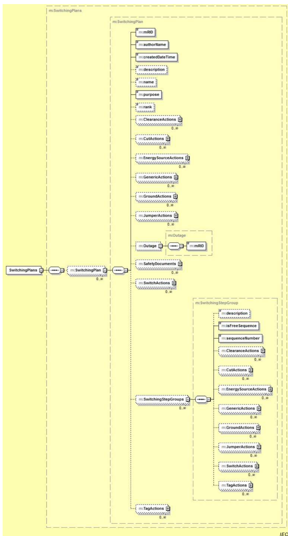
Figure 16 – Charge utile de message SwitchingPlans (Plans de commutation)
