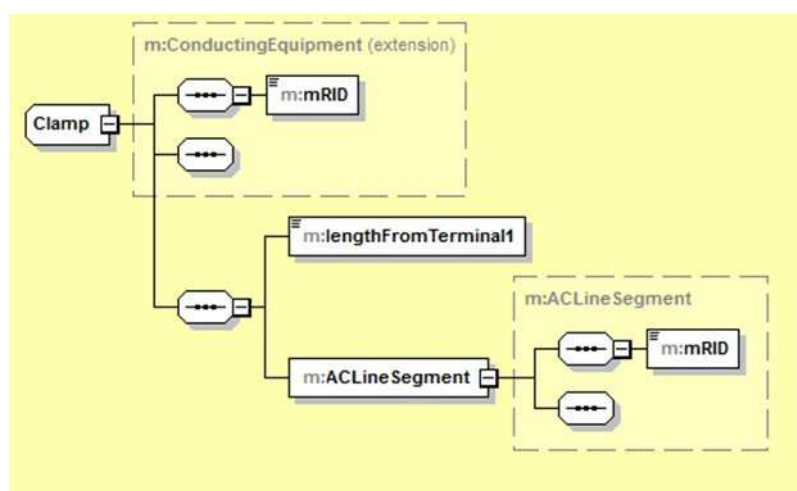
Figure 10 – TemporaryNetworkChanges message payload, Clamp detail
