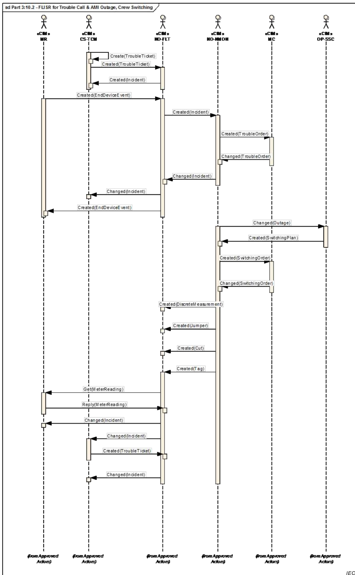
Figure A.2 – FLISR for trouble call and AMI outage, crew switching
