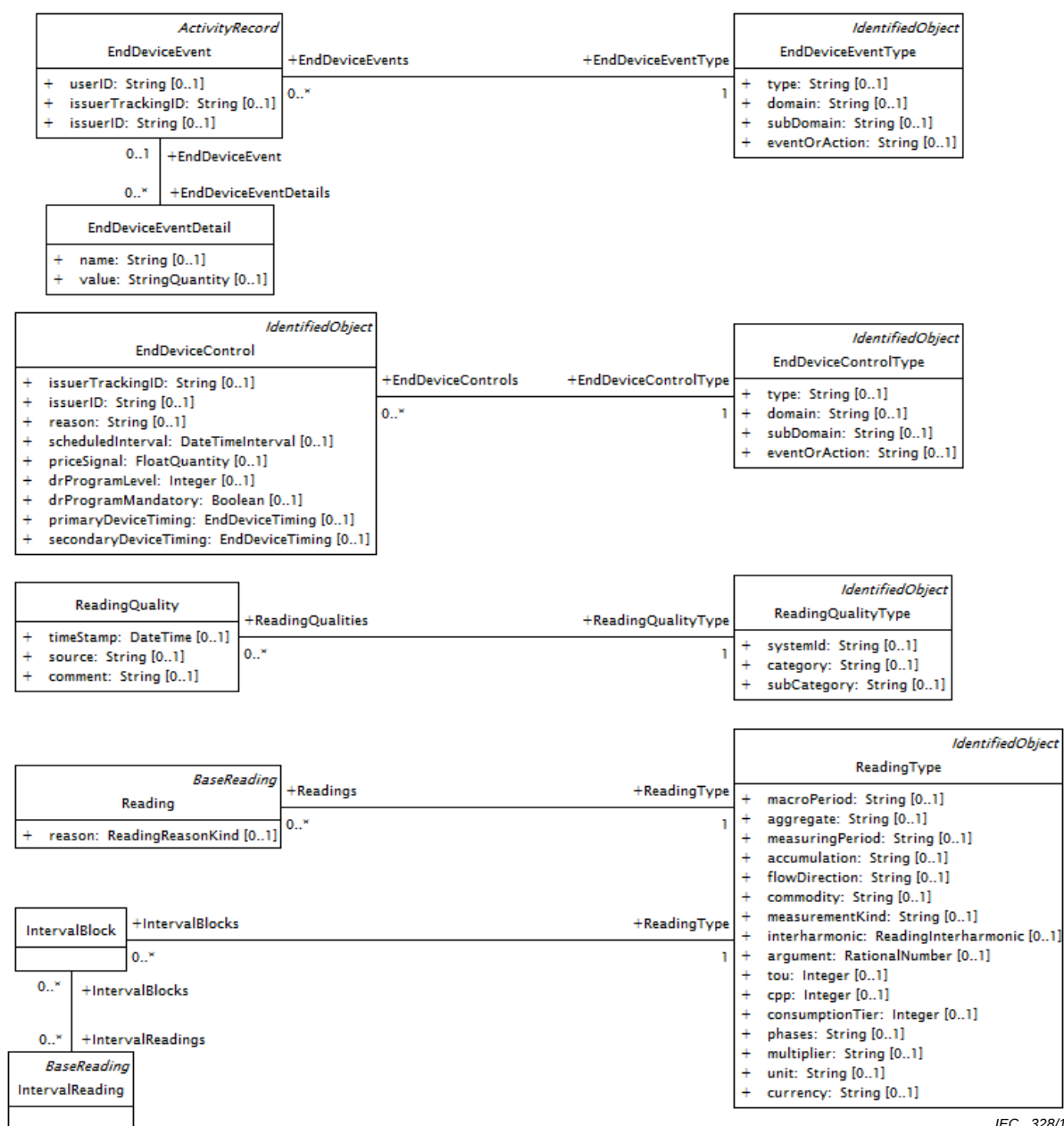
Figure 51 – Diagramme de classe Metering::MeteringTypes
