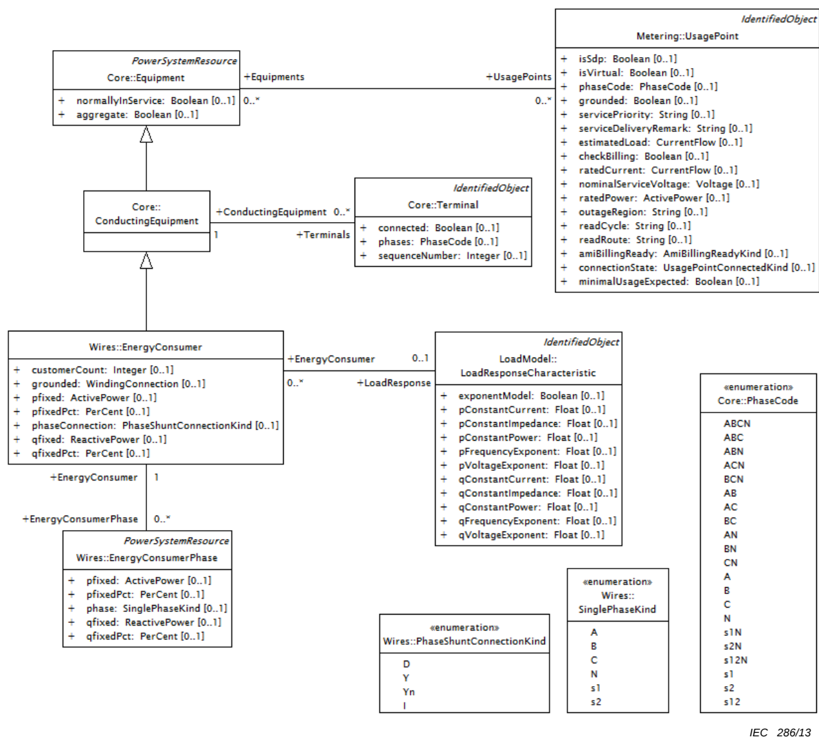
Figure 9 – DCIM load model
