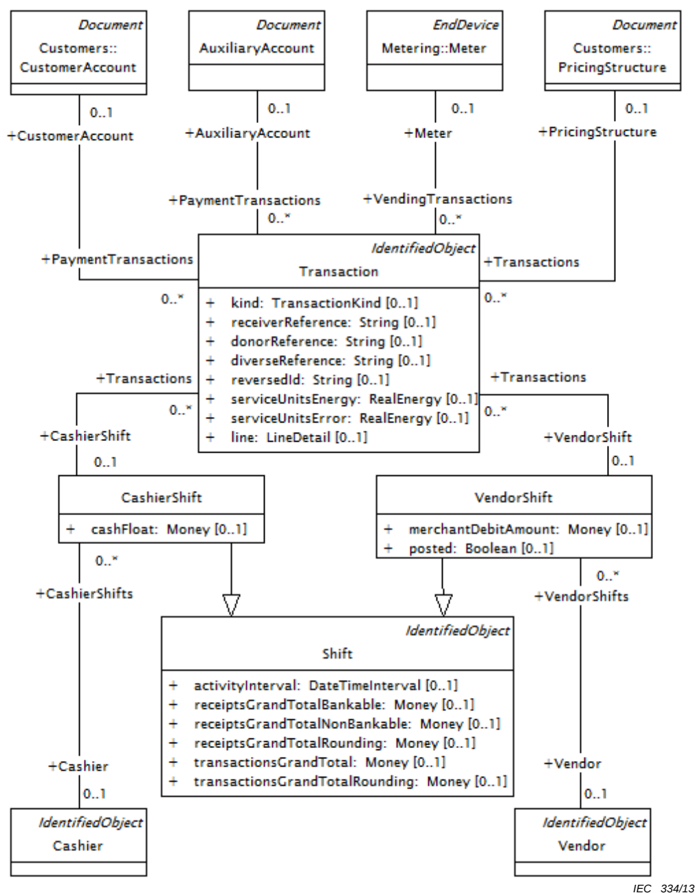
Figure 57 – Diagramme de classe PaymentMetering::Transacting
