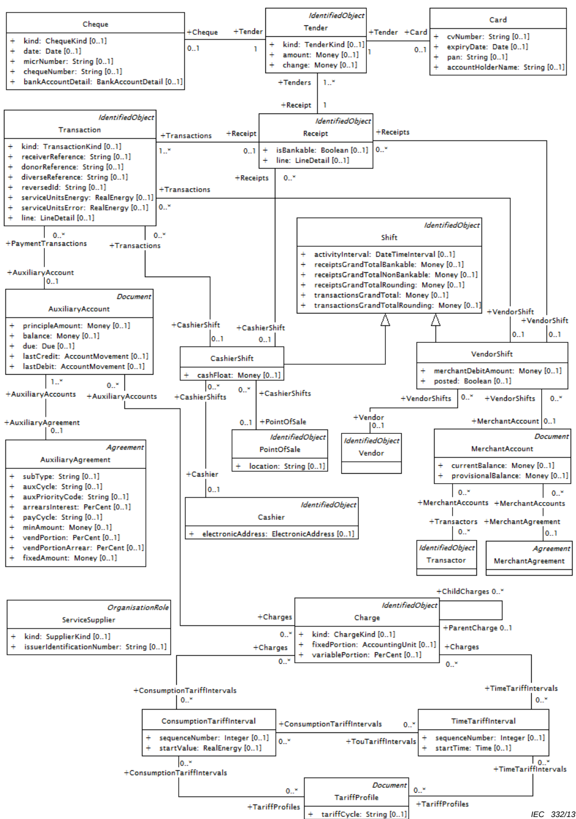
Figure 55 – Diagramme de classe PaymentMetering::PaymentMeteringOverview
