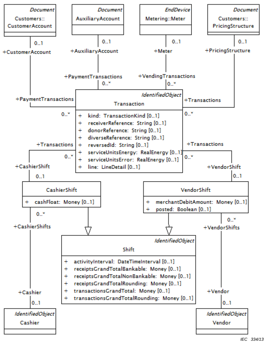
Figure 57 – Class diagram PaymentMetering::Transacting
