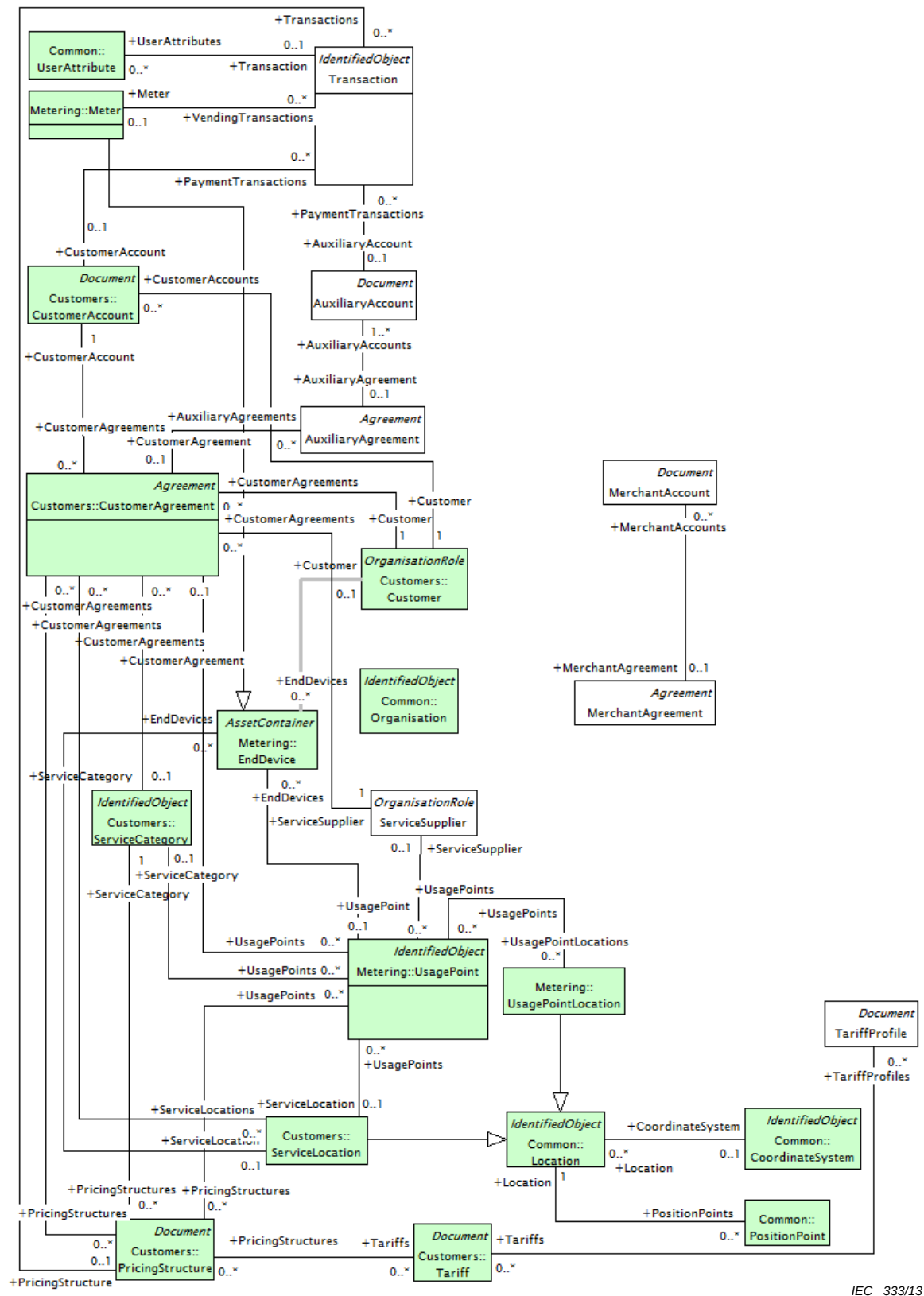
Figure 56 – Diagramme de classe PaymentMetering::PaymentMeteringRelationships
