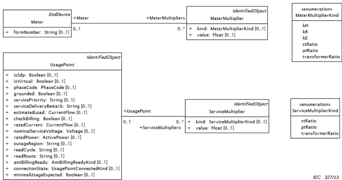
Figure 50 – Class diagram Metering::MeteringMultipliers
