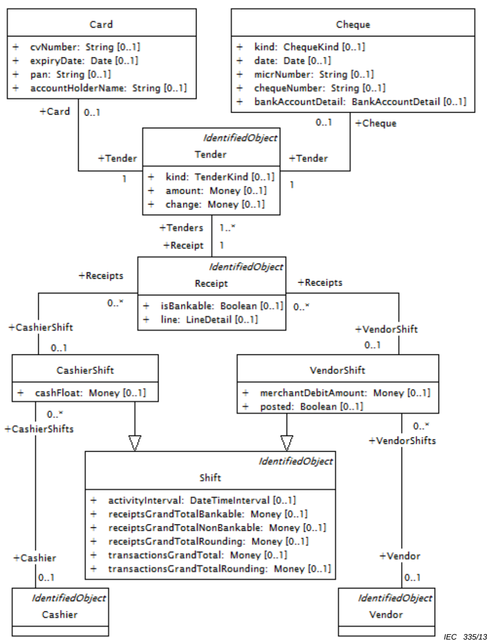
Figure 58 – Diagramme de classe PaymentMetering::Receipting
