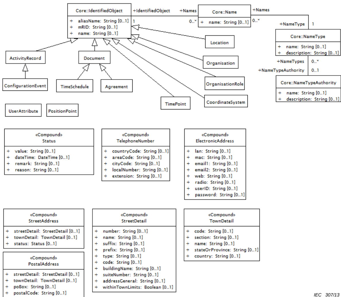
Figure 30 – Class diagram Common::CommonInheritance
