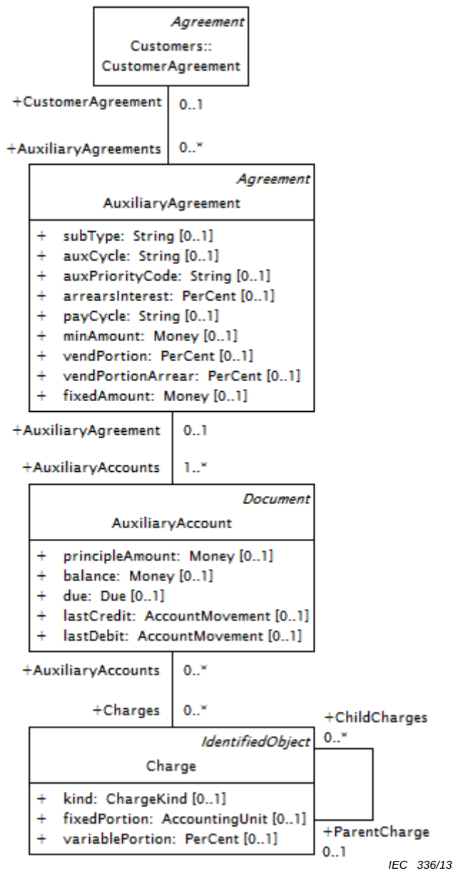
Figure 59 – Class diagram PaymentMetering::AuxiliaryAgreement
