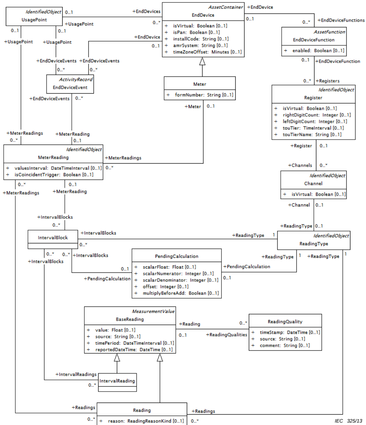
Figure 48 – Diagramme de classe Metering::MeteringMeterReadings
