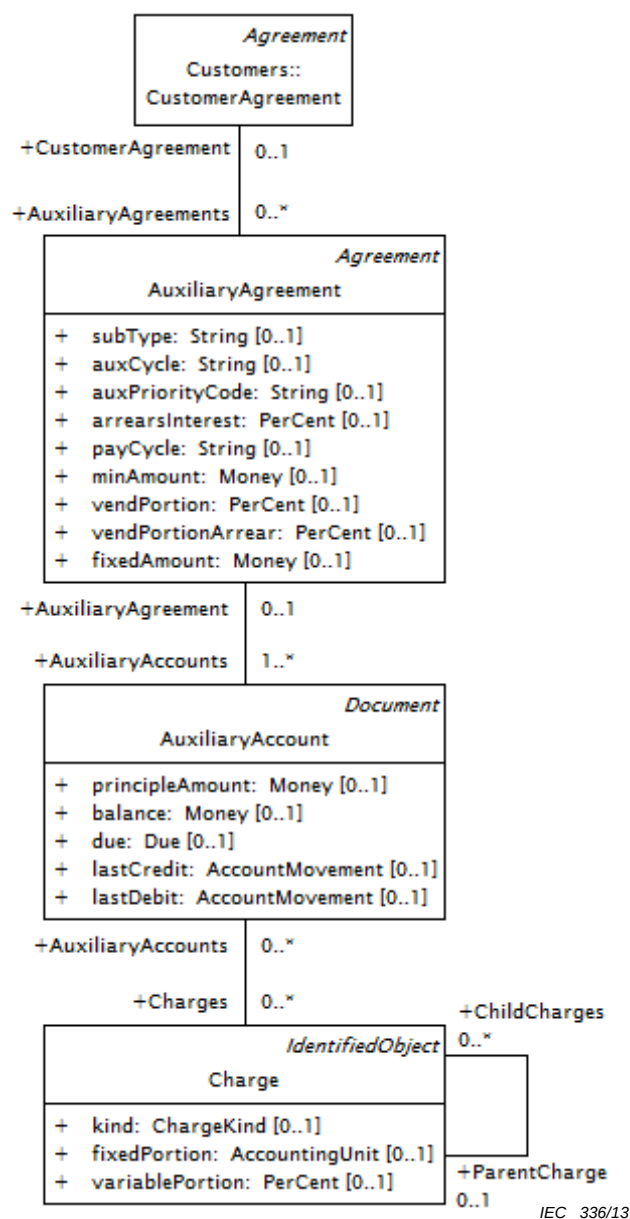
Figure 59 – Diagramme de classe PaymentMetering::AuxiliaryAgreement
