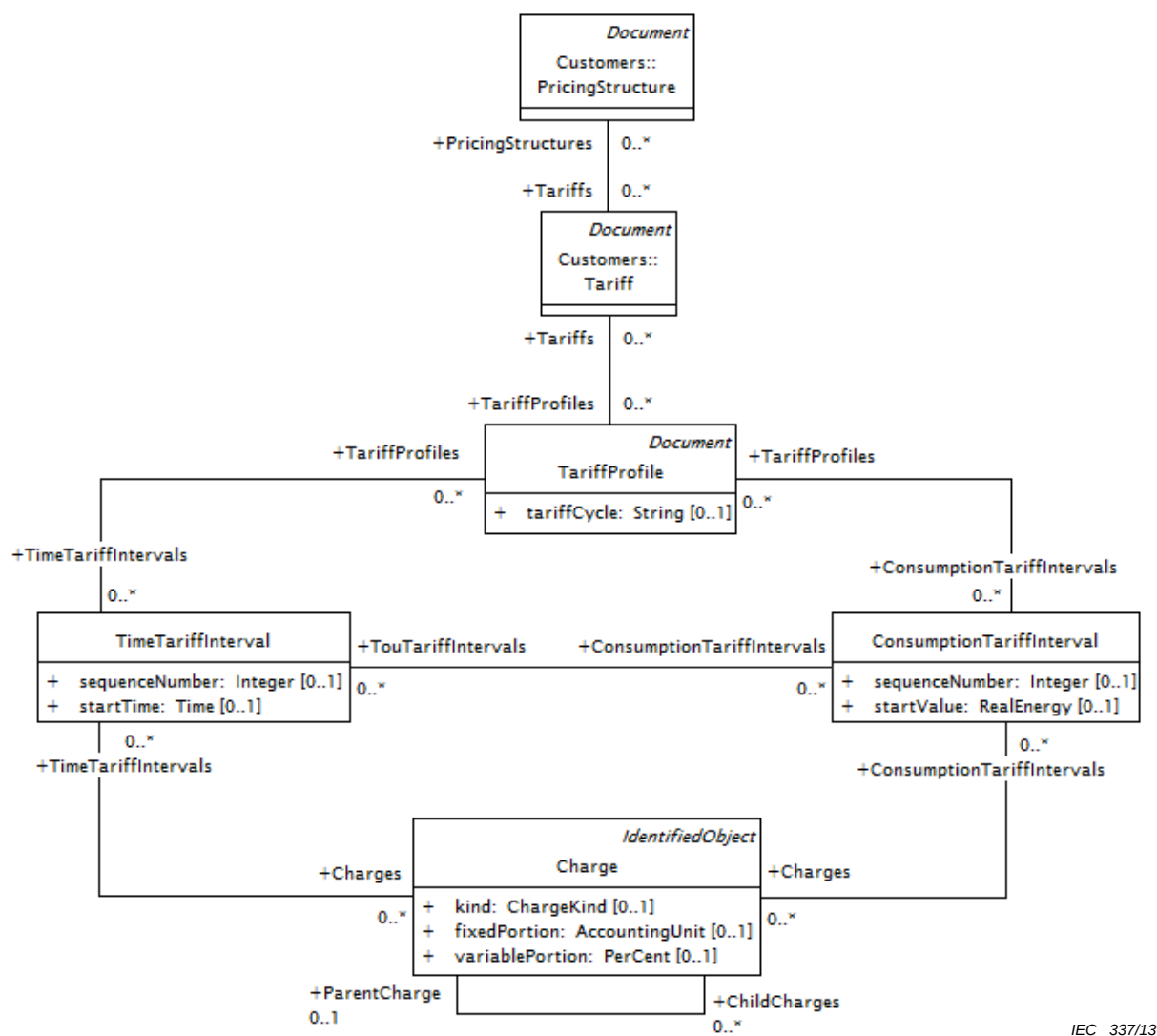
Figure 60 – Diagramme de classe PaymentMetering::TariffProfile
