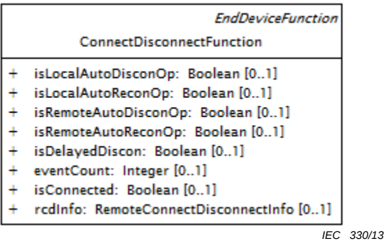
Figure 53 – Diagramme de classe LoadControl::LoadControlOverview
