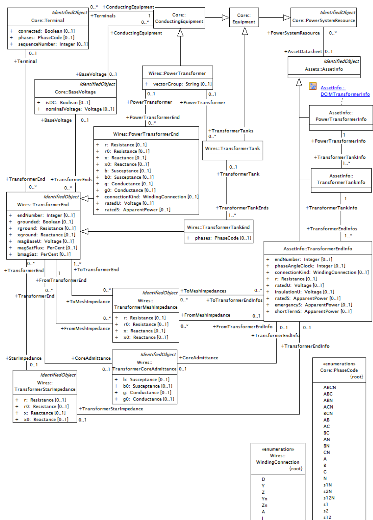
Figure 12 – DCIM transformer connectivity model
