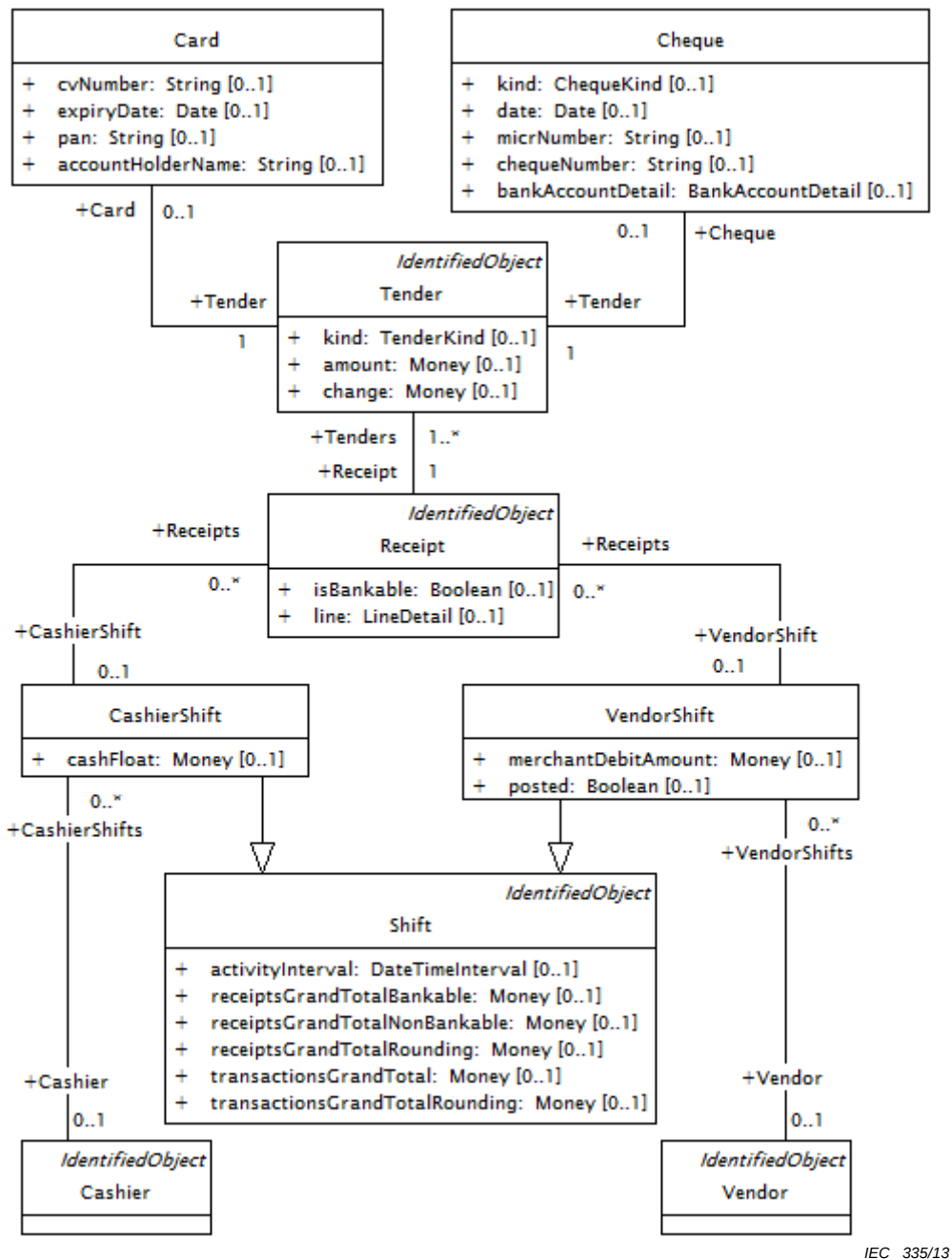
Figure 58 – Class diagram PaymentMetering::Receipting
