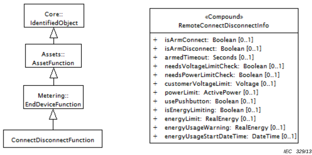
Figure 52 – Diagramme de classe LoadControl::LoadControlInheritance
