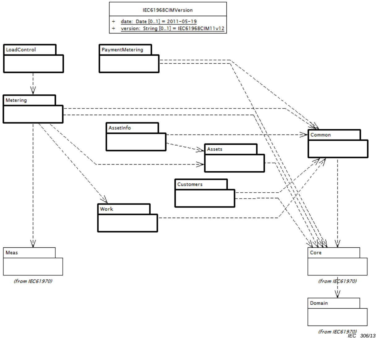
Figure 29 – Diagramme des paquetages IEC61968::IEC61968Dependencies
