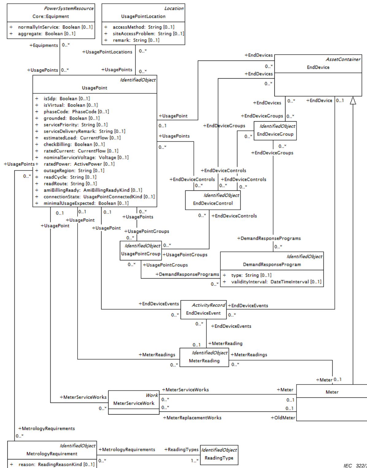
Figure 45 – Diagramme de classe Metering::MeteringUsagePoints
