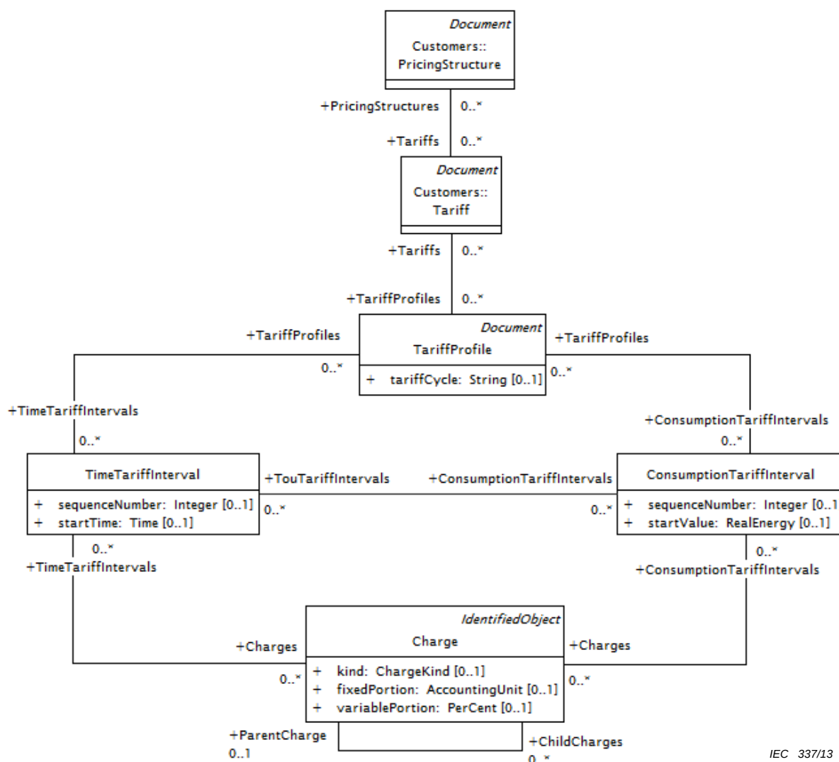
Figure 60 – Class diagram PaymentMetering::TariffProfile
