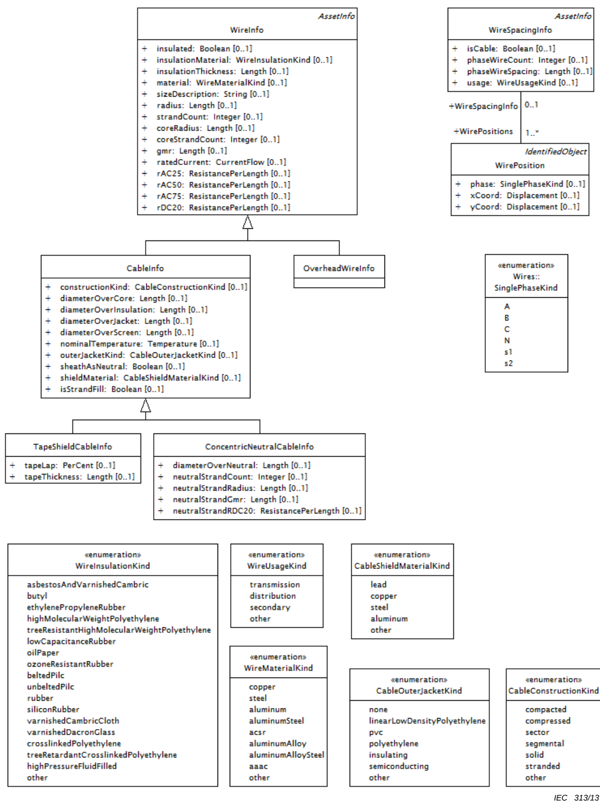
Figure 36 – Class diagram AssetInfo::DCIMWireInfo
