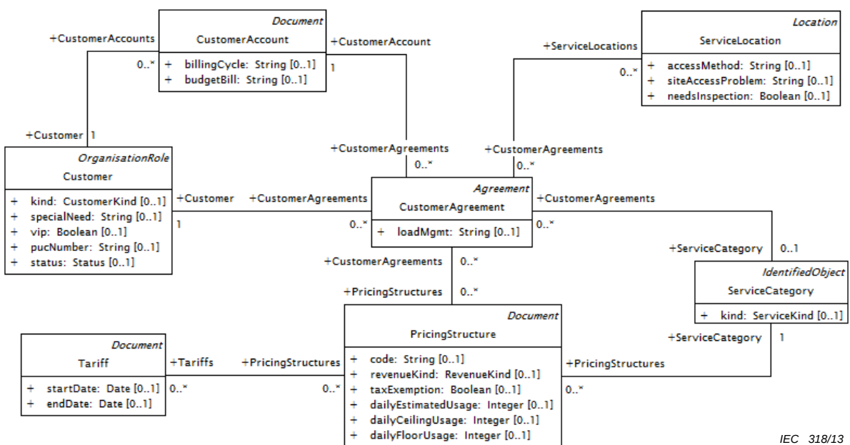
Figure 41 – Diagramme de classe Customers::CustomersOverview
