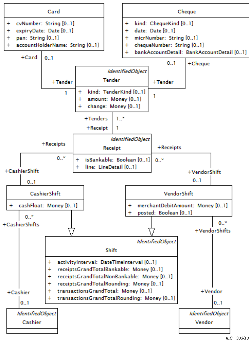
Figure 26 – DCIM receipting model
