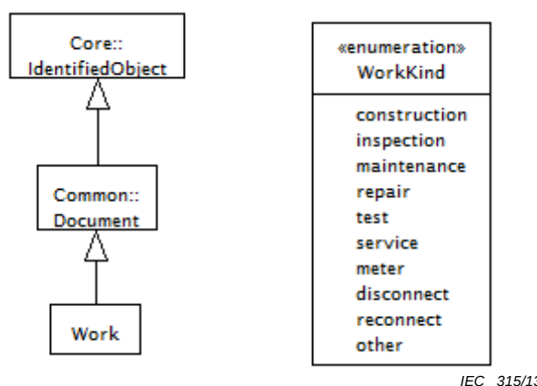
Figure 38 – Diagramme de classe Work::WorkInheritance
