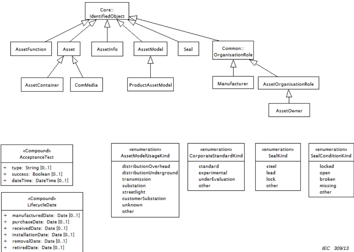
Figure 32 – Diagramme de classe Assets::AssetsInheritance
