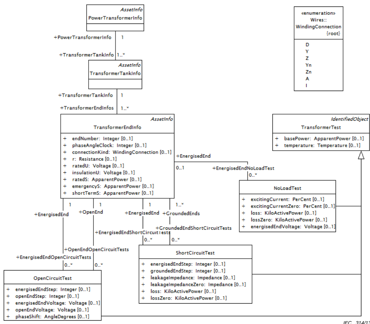
Figure 37 – Diagramme de classe AssetInfo::DCIMTransformerInfo
