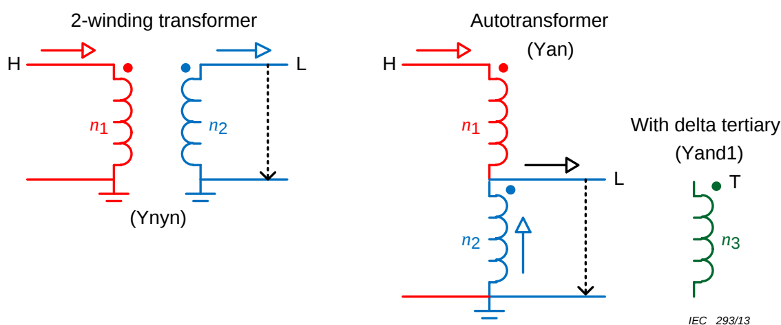
Figure 16 – Example of a two-winding transformer connected as an autotransformer
