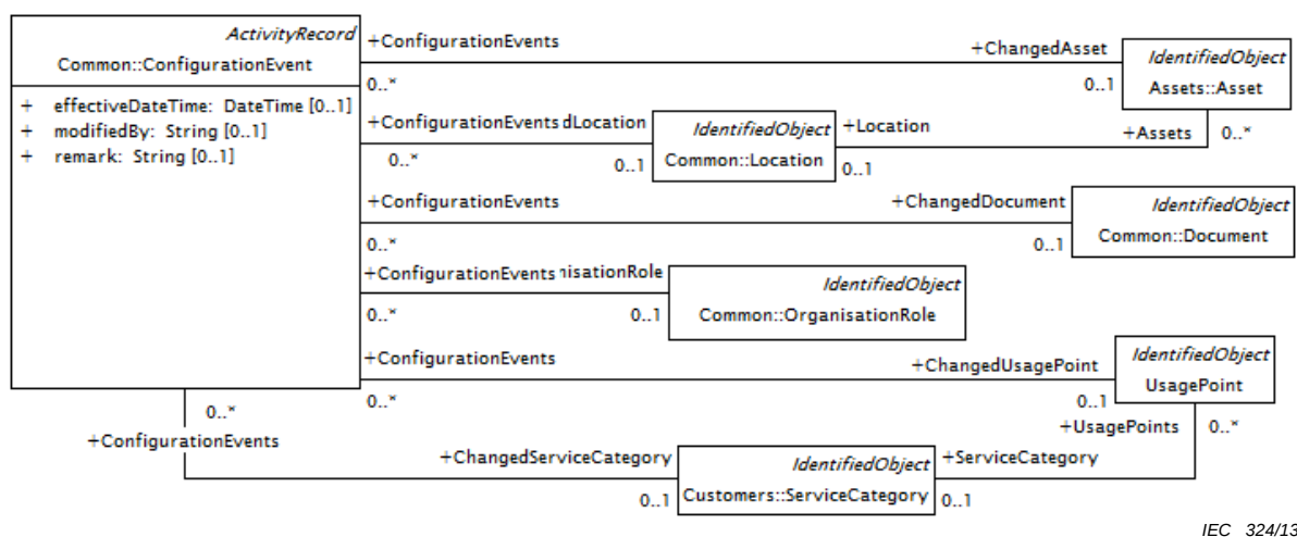
Figure 47 – Diagramme de classe Metering::MeteringConfigurationEvents
