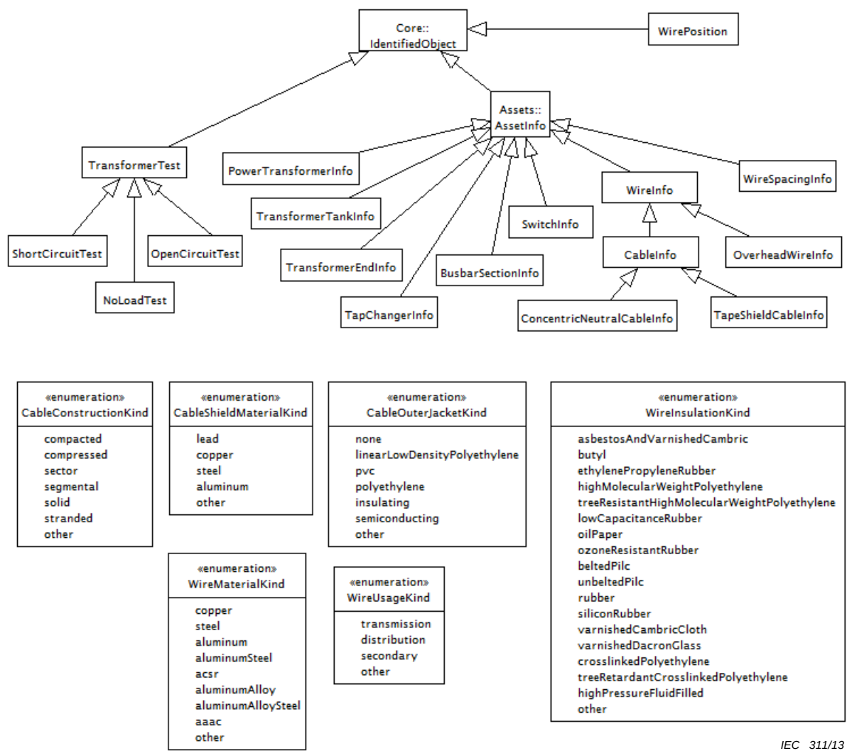
Figure 34 – Class diagram AssetInfo::AssetInfoInheritance
