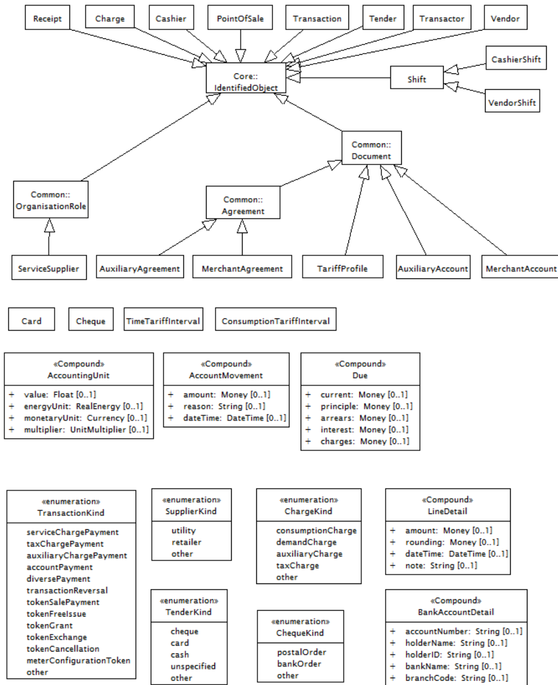
Figure 54 – Diagramme de classe PaymentMetering::PaymentMeteringInheritance
