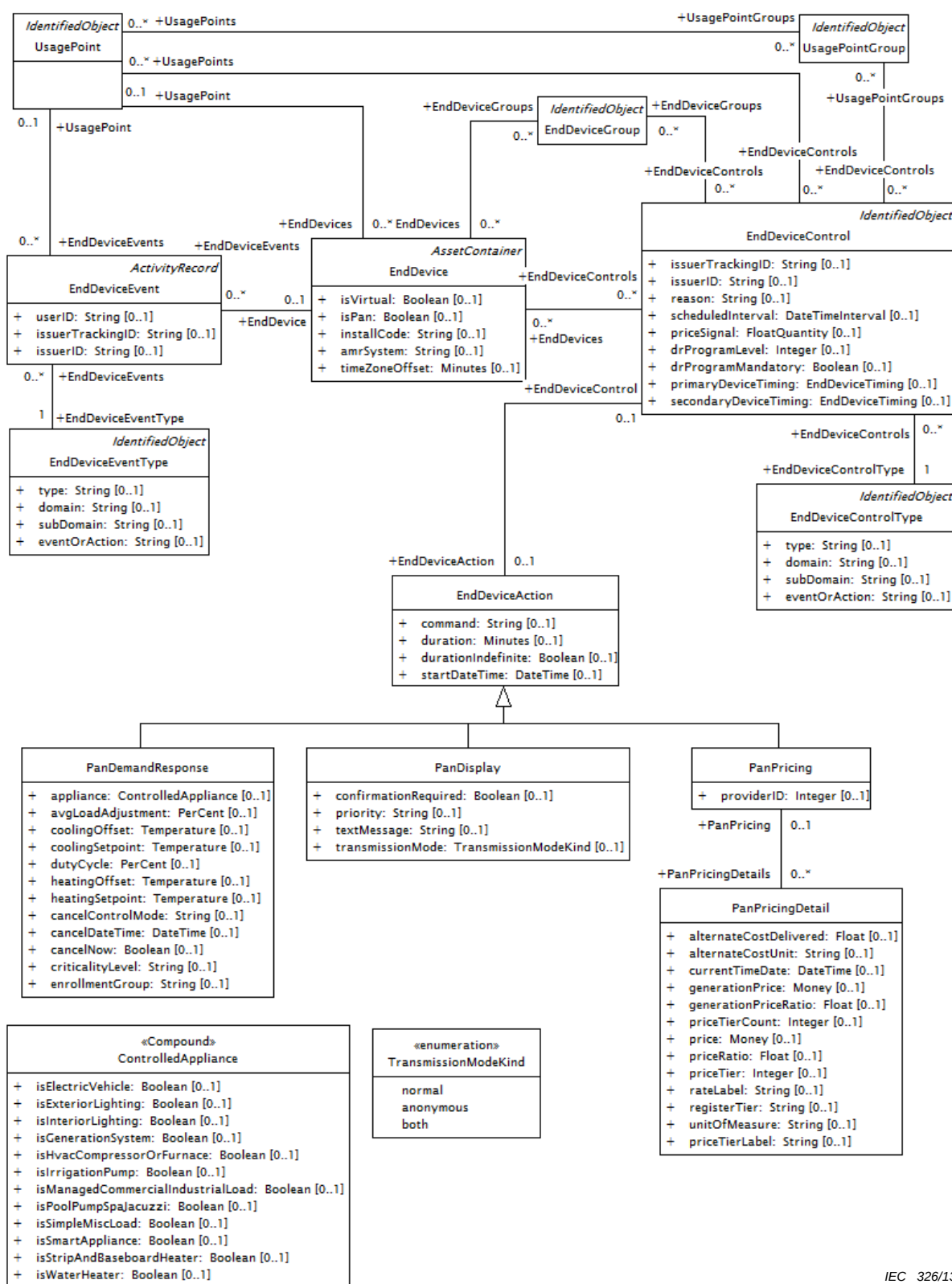
Figure 49 – Diagramme de classe Metering::MeteringEventsAndControls
