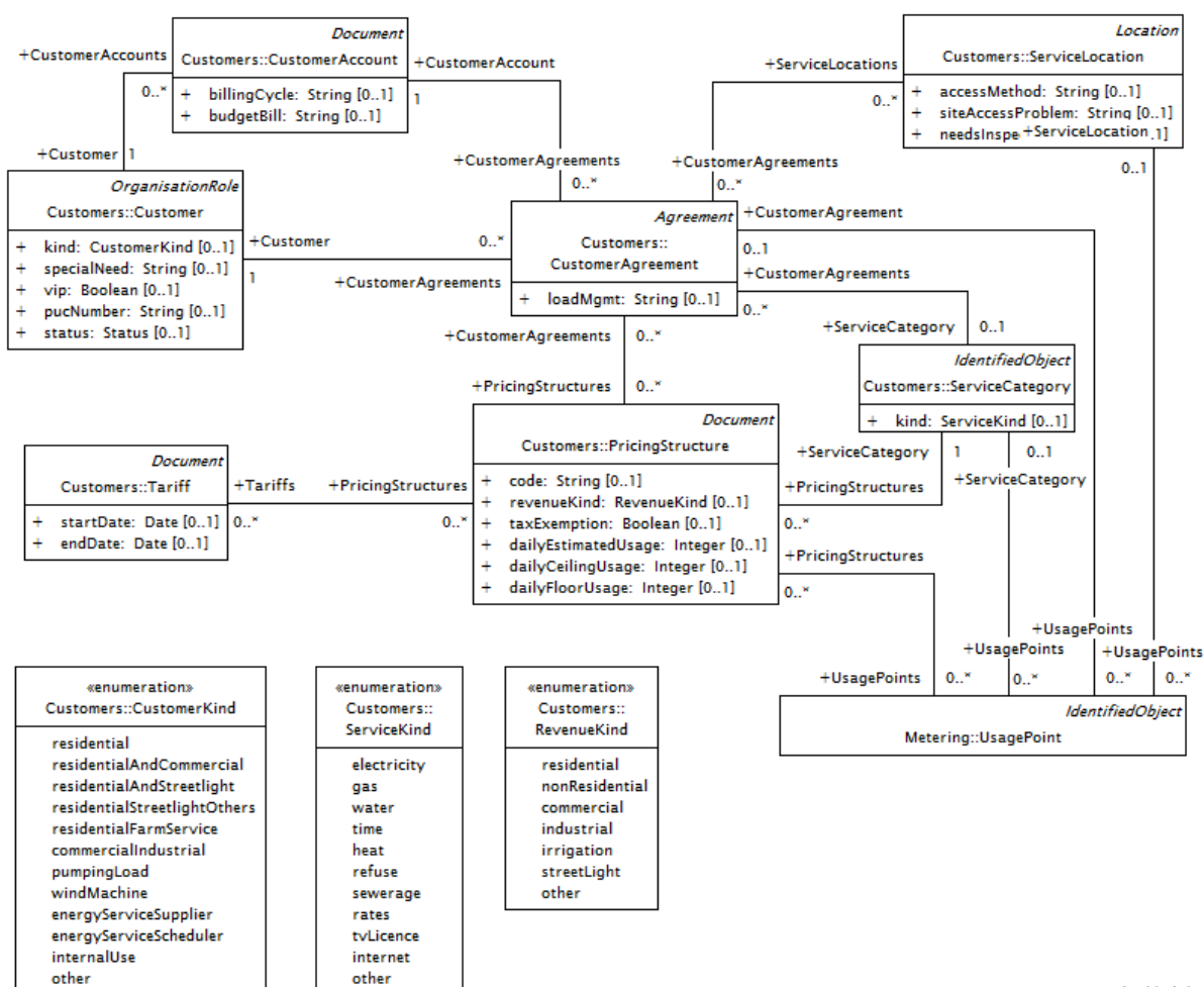
Figure 18 – Modèle Customers DCIM
