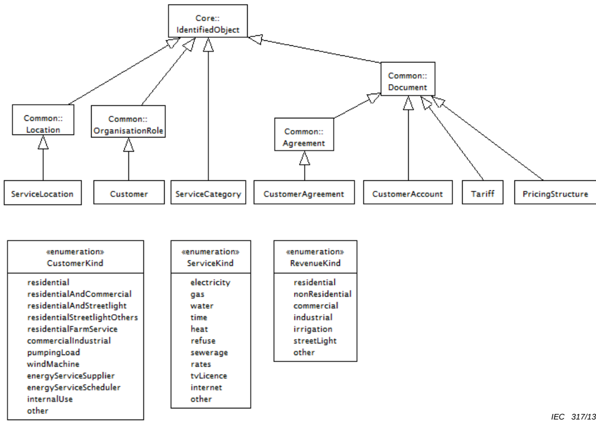
Figure 40 – Diagramme de classe Customers: :CustomersInheritance
