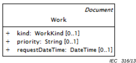
Figure 39 – Diagramme de classe Work::WorkOverview
