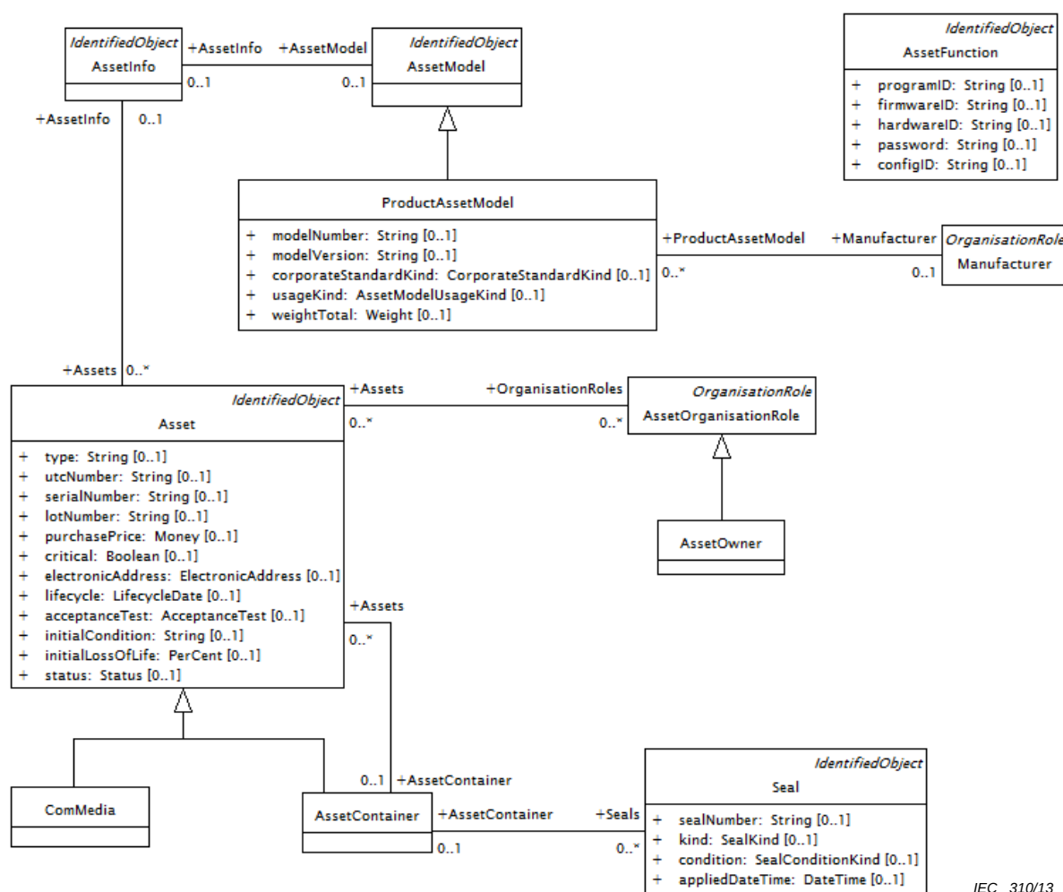
Figure 33 – Diagramme de classe Assets::AssetsOverview
