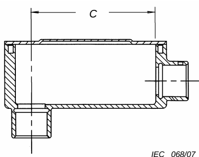
Figure 21 C – Angle pull (side view)
