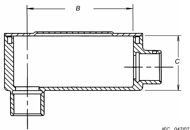
Figure 5b – Angled pull (side view)
