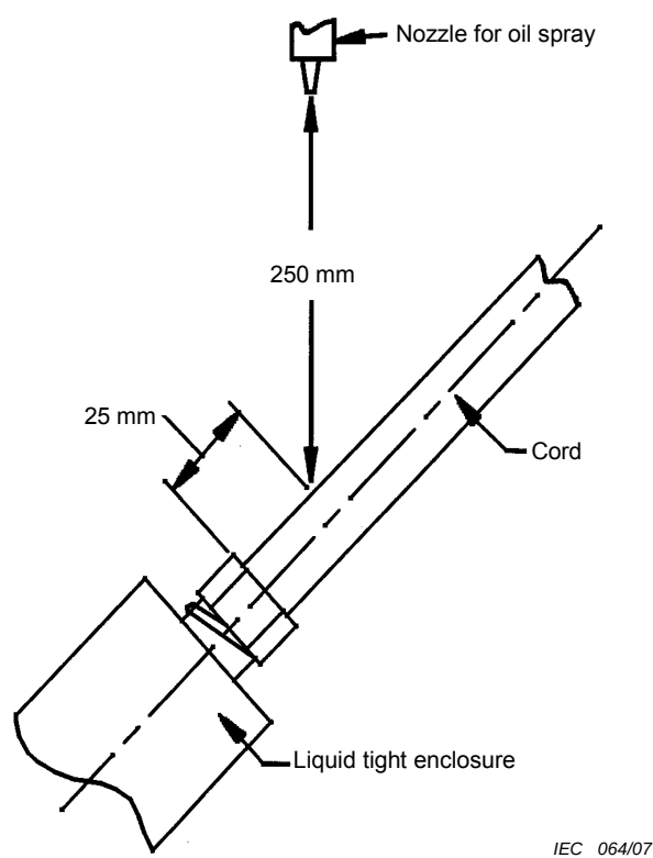
Figure 19 – Oil spray test fixture (see 9.22.4.2)
