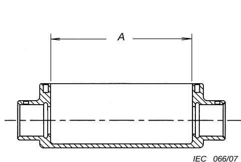
Figure 21 A – Straight pull (side view)
