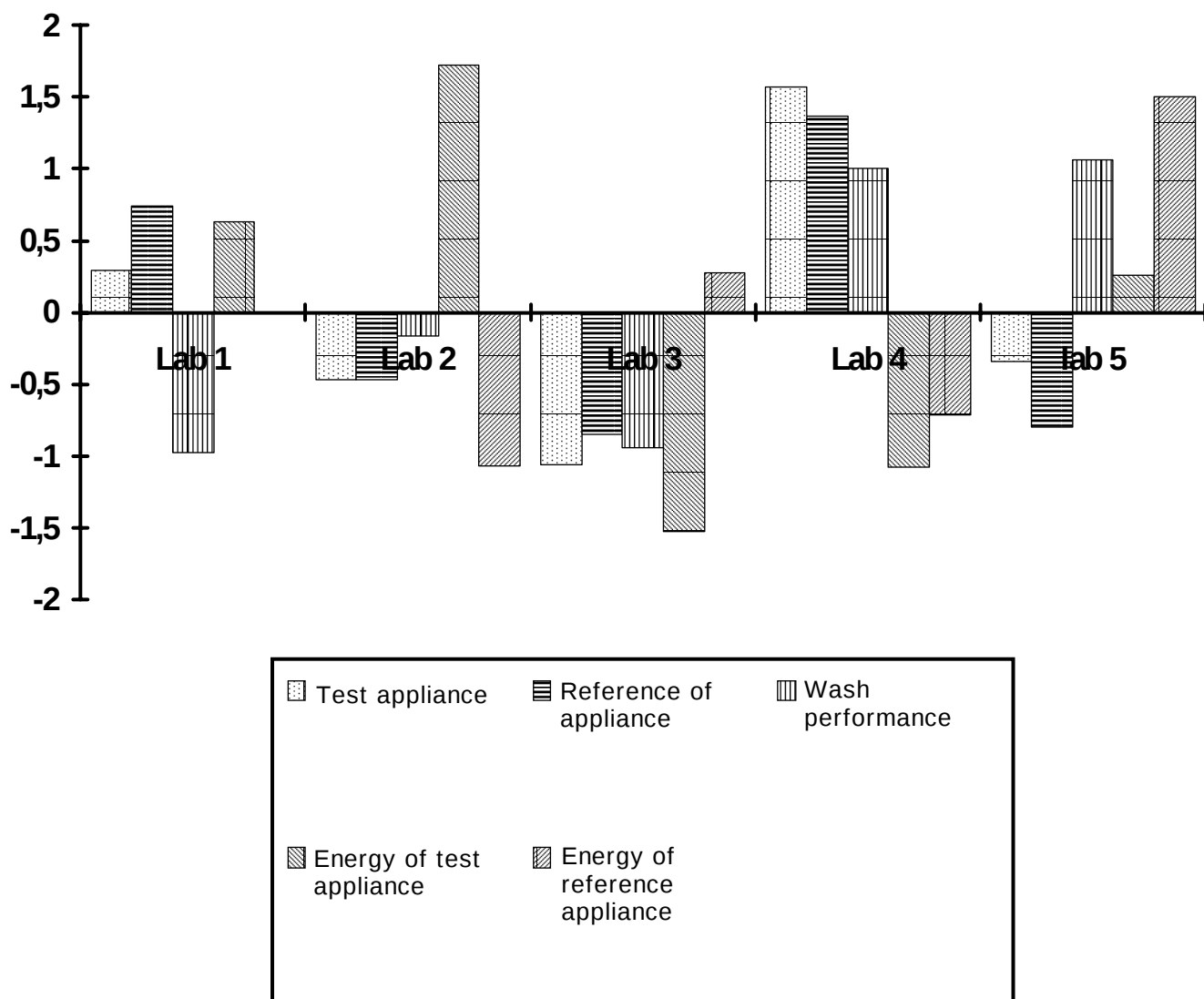
Figure A.1 – Mandel's h statistics
