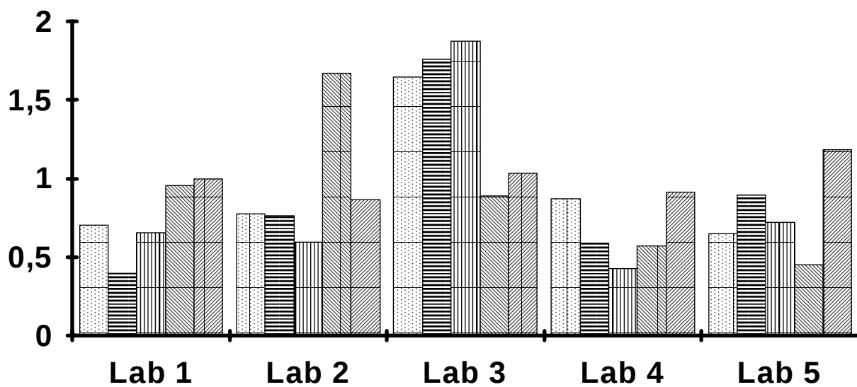
Figure A.1 – Mandel's h statistics
