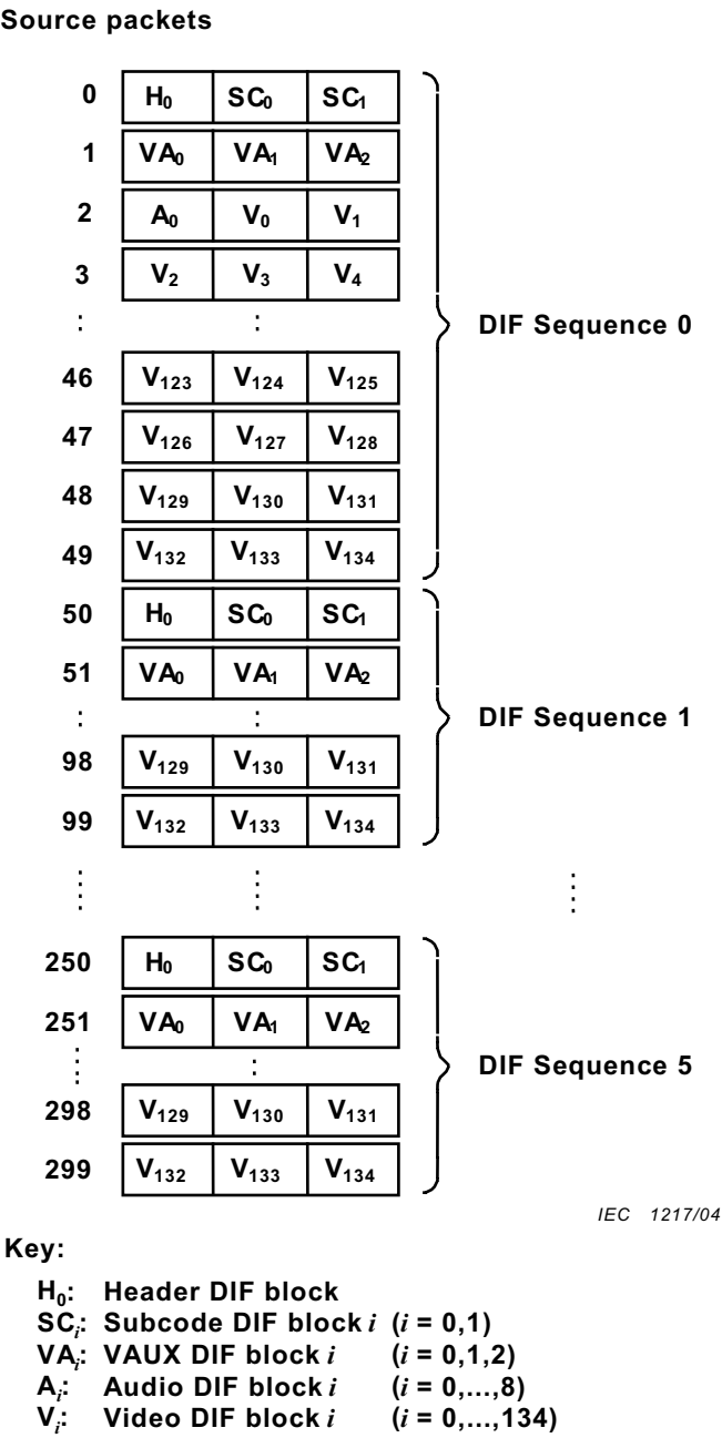
Figure 2 – Source packets of SDL-DVCR SDL625-50 system
