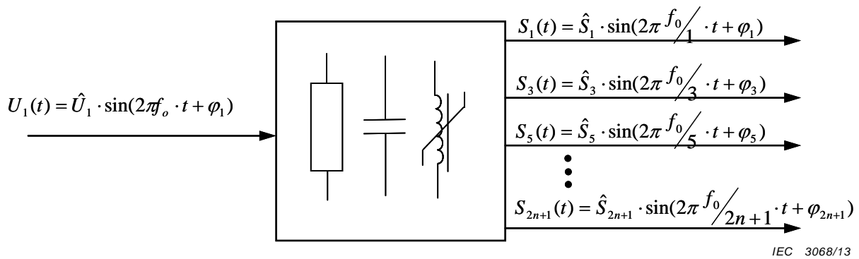
Figure A.3 – A non-linear oscillation system
