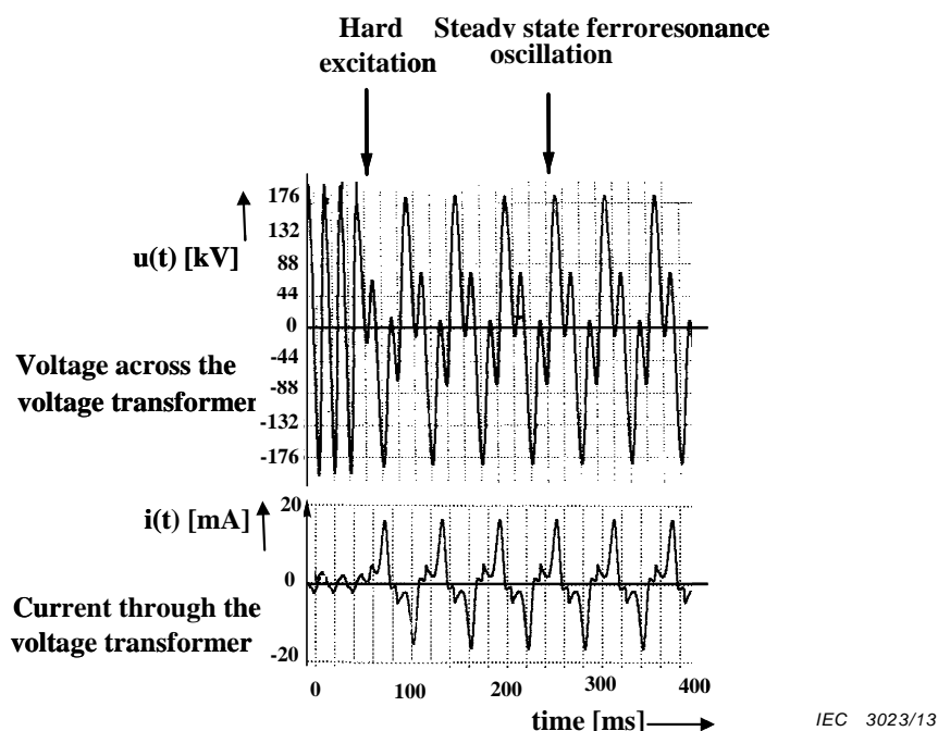
a) Single-phase steady state ferroresonance oscillations, type 2a according to Table 1
