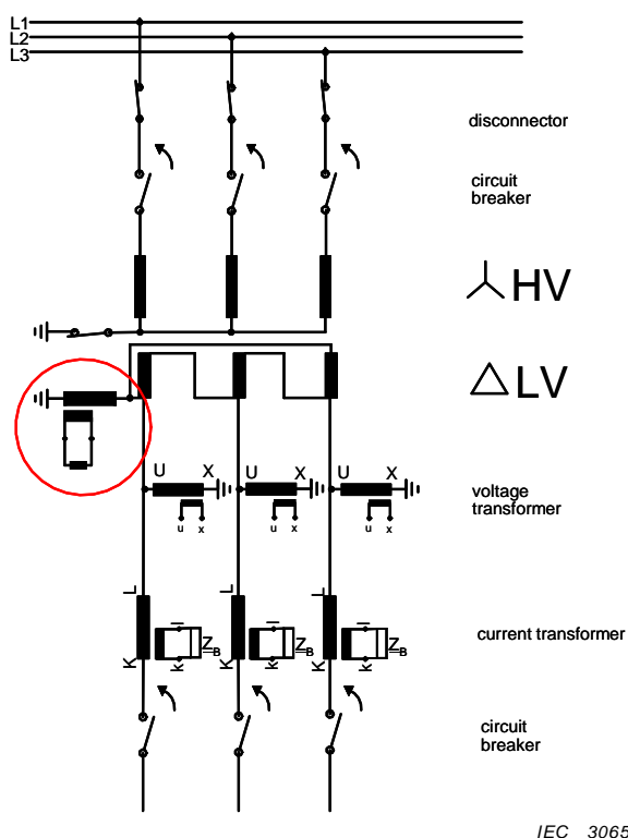
Figure 37 – Damping of ferroresonance oscillations with voltage transformer in the star point of the power transformer
