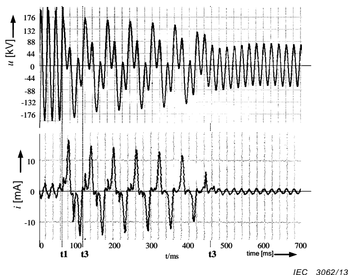
Figure 35 – Example of successful damping of single-phase ferroresonance oscillations of 16\frac{2}{3} Hz
