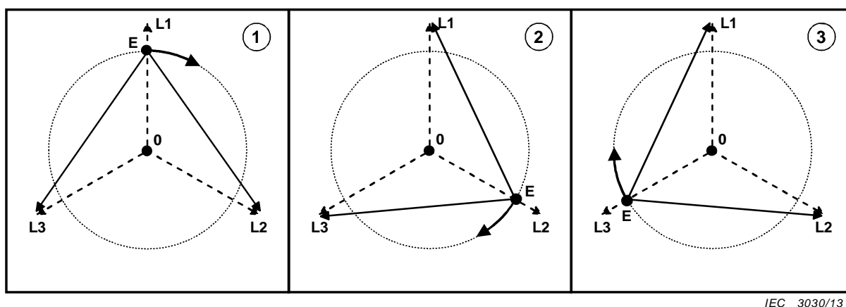
Figure 8 – Phasor diagram to explain the oscillation of the earth potential
