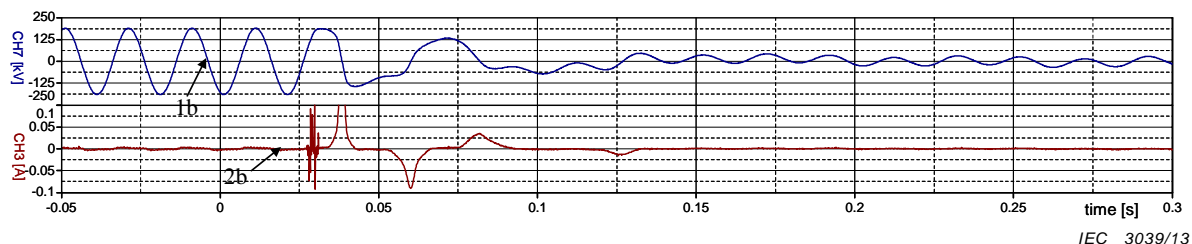
b) Non-steady state, decreasing ferroresonance oscillation, transient waveform (between 0,03 and 0,15 s); switching near zero crossing of voltage (between 0,15 s and 0,3 s the coupled a.c. voltage can be seen)
