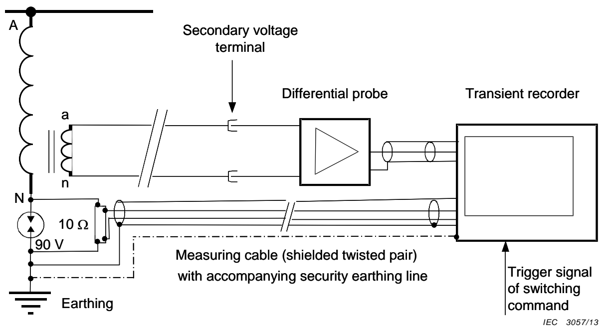
b) current measurement with shunt resistor
