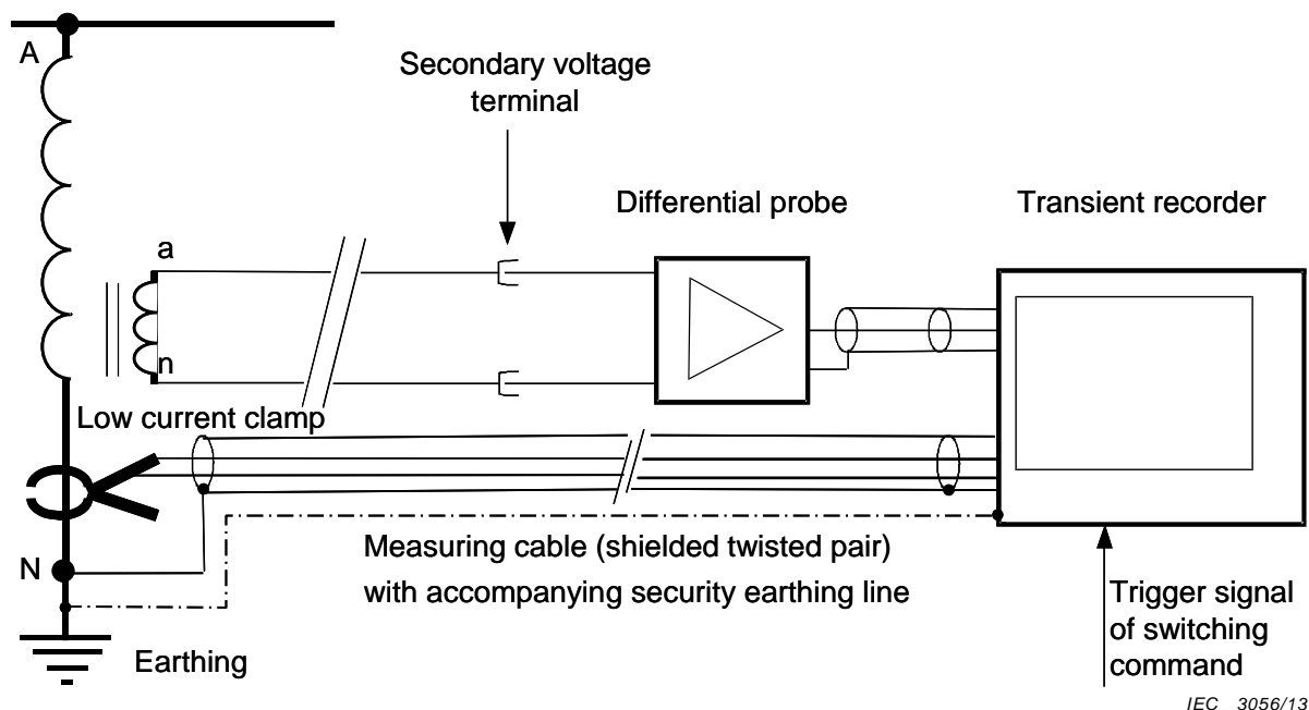
a) current measurement with current clamp
