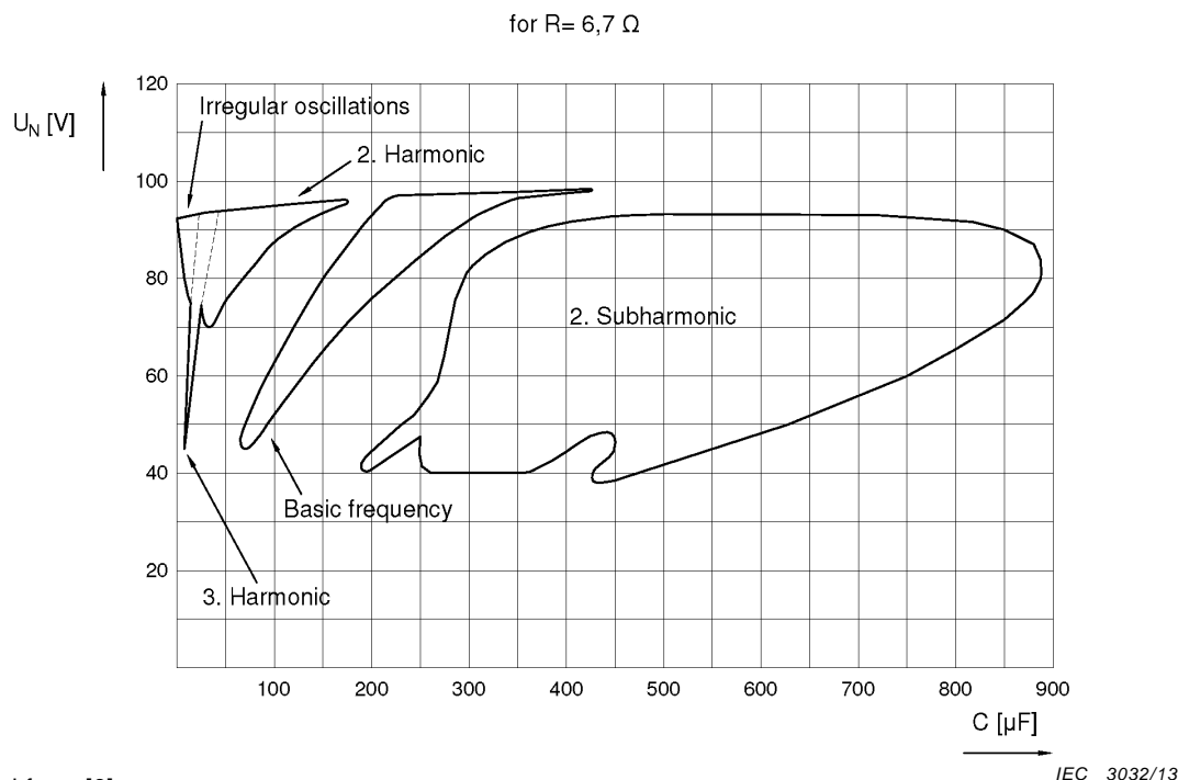
Figure 10 – Domains in the capacitance C and line voltage U where different harmonic and sub-harmonic ferroresonance oscillations are obtained for a given resistance R of 6,7 \, \Omega in Bergmann's test set
