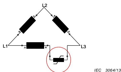
b) open delta connection of the secondary windings
