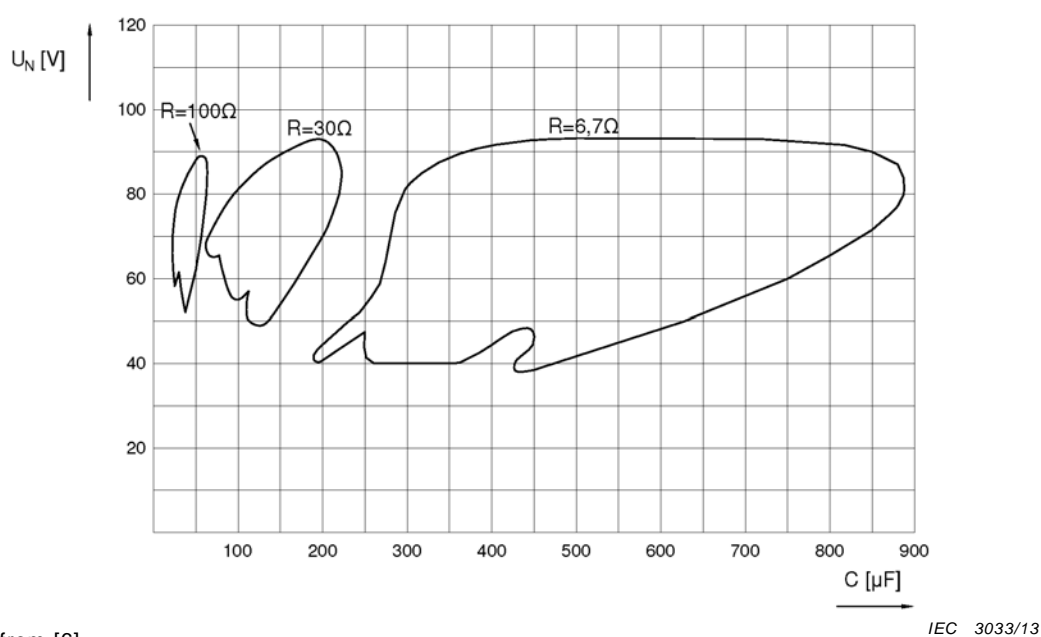
Figure 11 – Domains in the capacitance C and line voltage U where second sub-harmonic ferroresonance oscillations are obtained for a variation of the resistance R in Bergmann's test set
