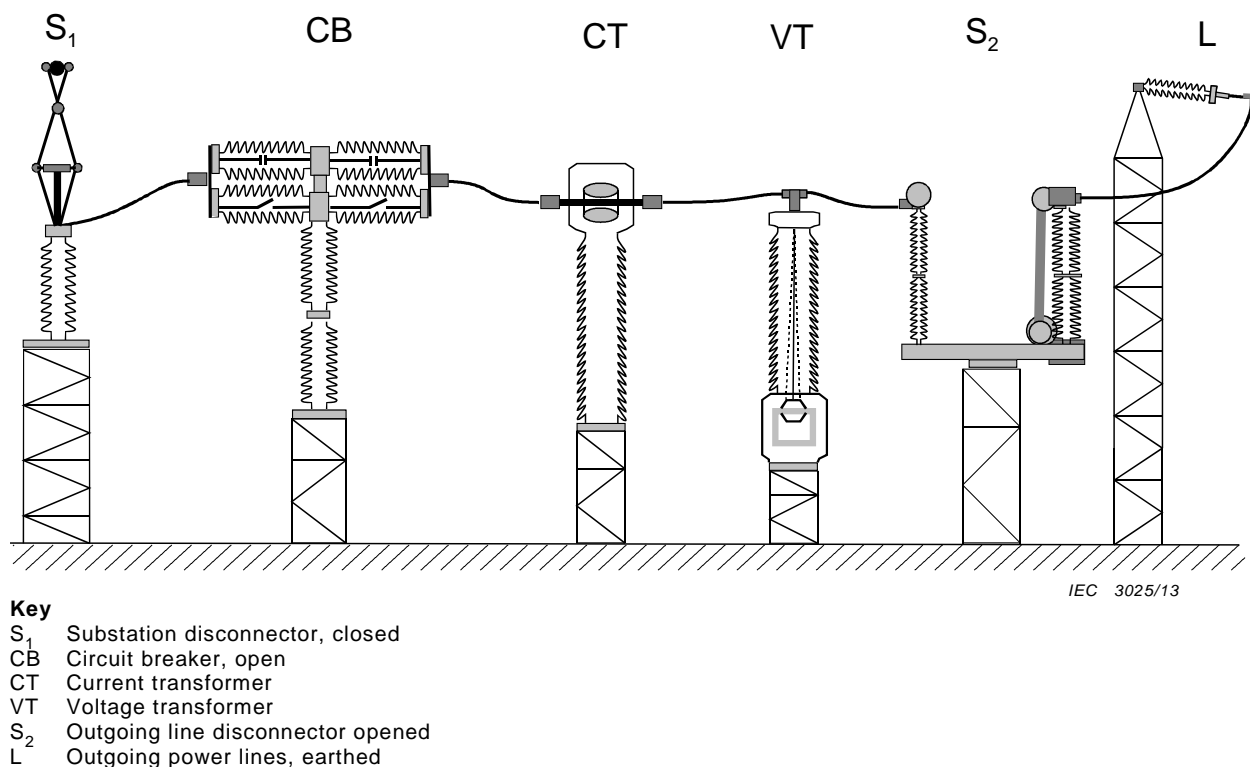
Figure 4 – Schematic diagram of a de-energised outgoing feeder bay with voltage transformers as an example in which single-phase ferroresonance oscillations can occur
