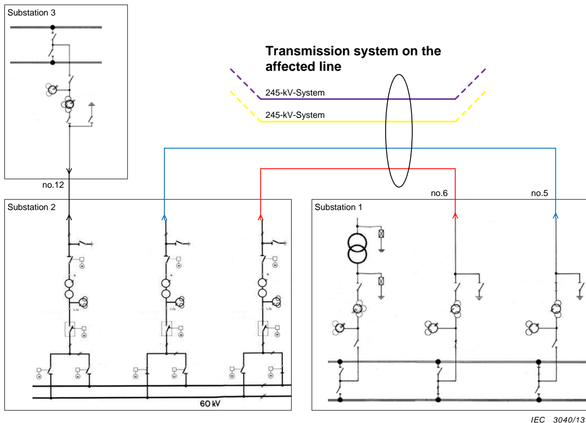
Figure 16 – Single-phase schematic of the network situation on the 60 kV voltage level in the area of substations 1, 2, and 3
