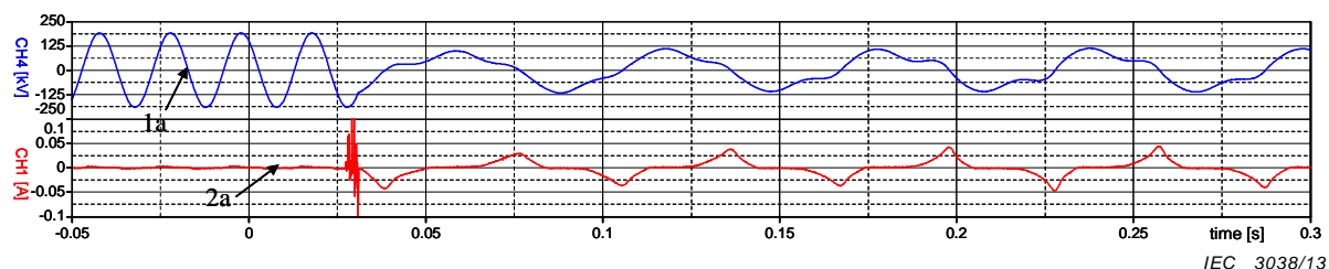
a) Steady state ferroresonance oscillations, frequency 16\frac{2}{3} Hz; switching near the voltage maximum
