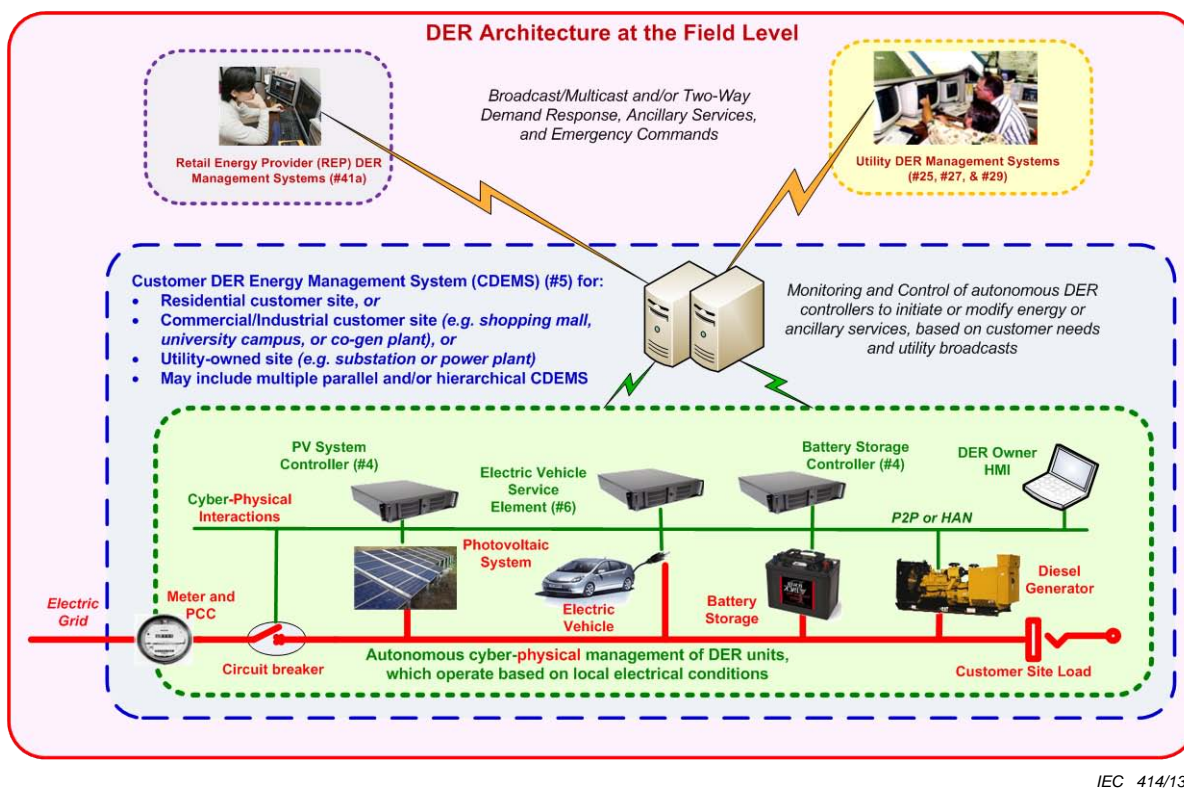
Figure 1 – DER management hierarchical interactions: autonomous, loosely-coupled, broadcast/multicast
