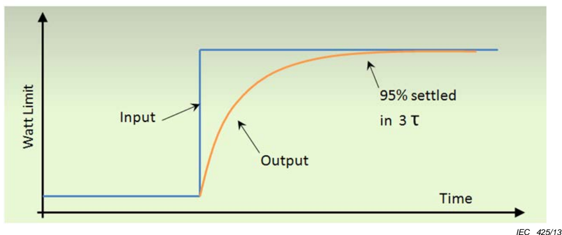
Figure 12 – Time domain response of first order low pass filter
