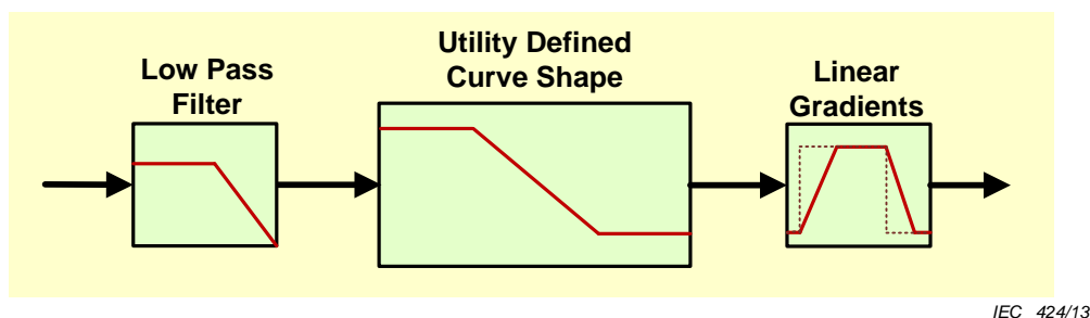
Figure 11 – Local function block diagram
