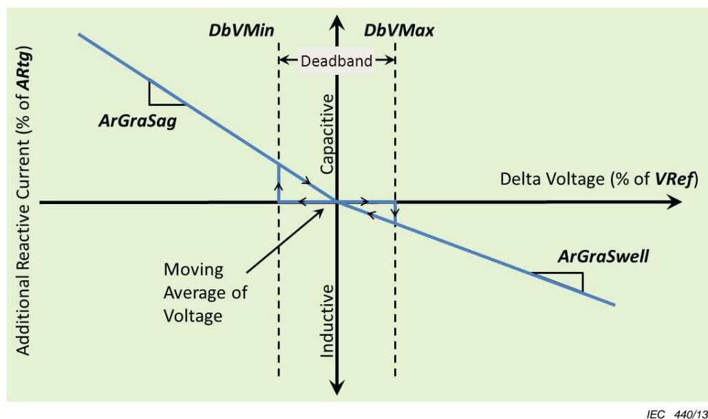
Figure 27 – Alternative gradient behaviour, selected by ArGraMod
