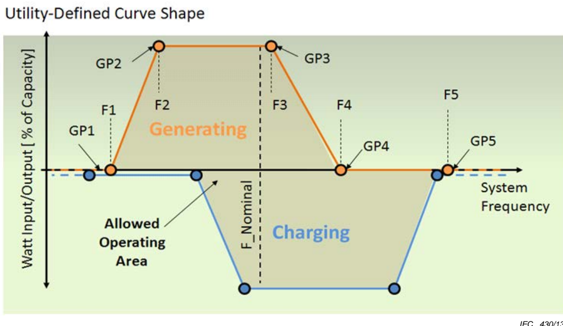
Figure 17 – Frequency-watt mode curves
