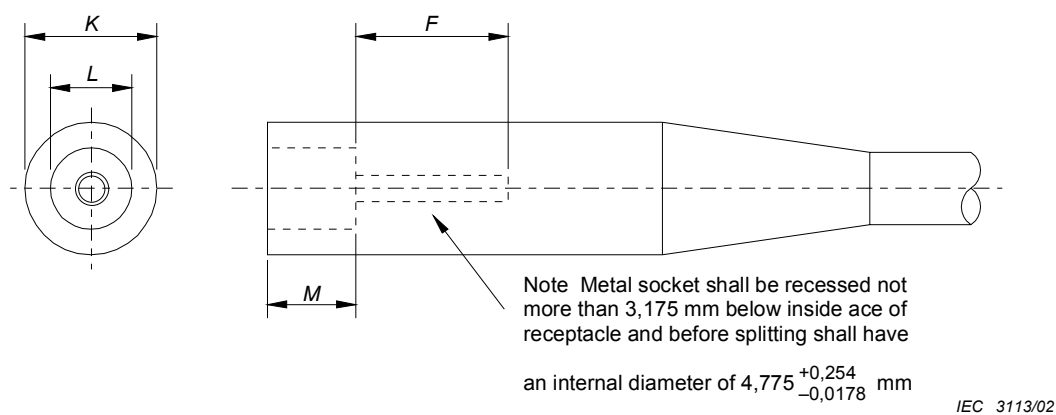
Figure A.2 – Style 9 primary receptacle
