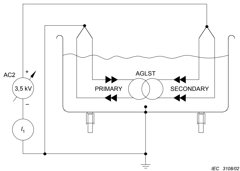
Figure 3 – Secondary a.c. leakage current test
