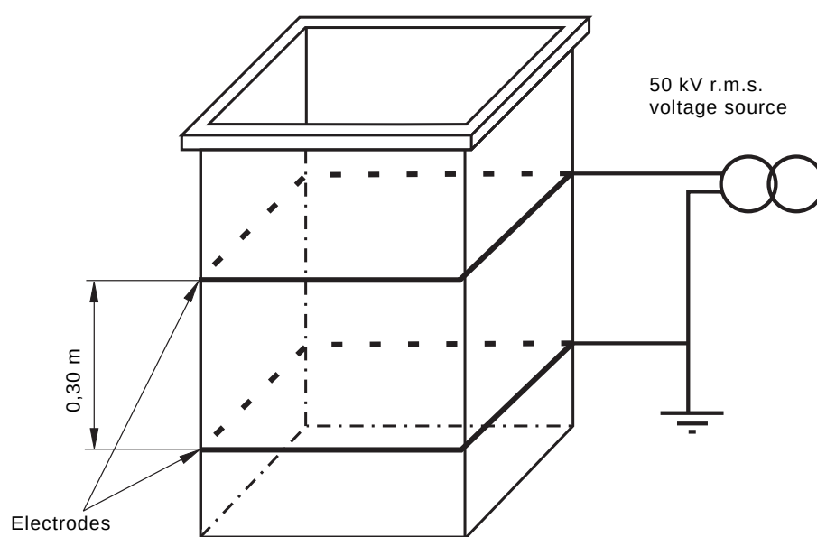
Figure 5 – Surface test on insulating platform or liner
