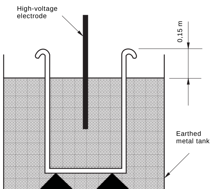
Figure 4 – Puncture test on insulating platform or liner
