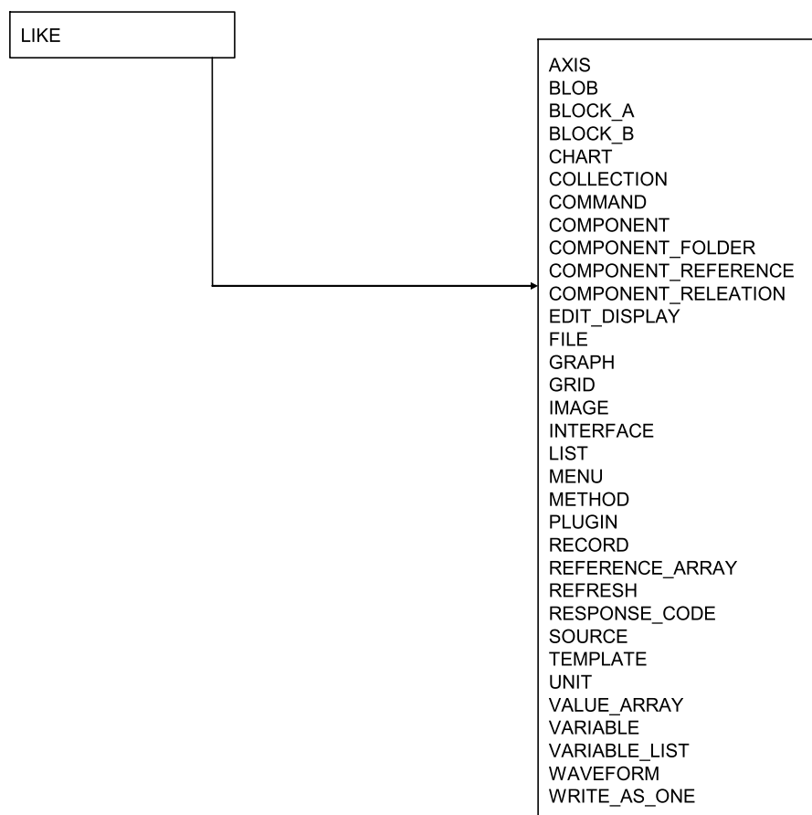
Figure 16 – LIKE
