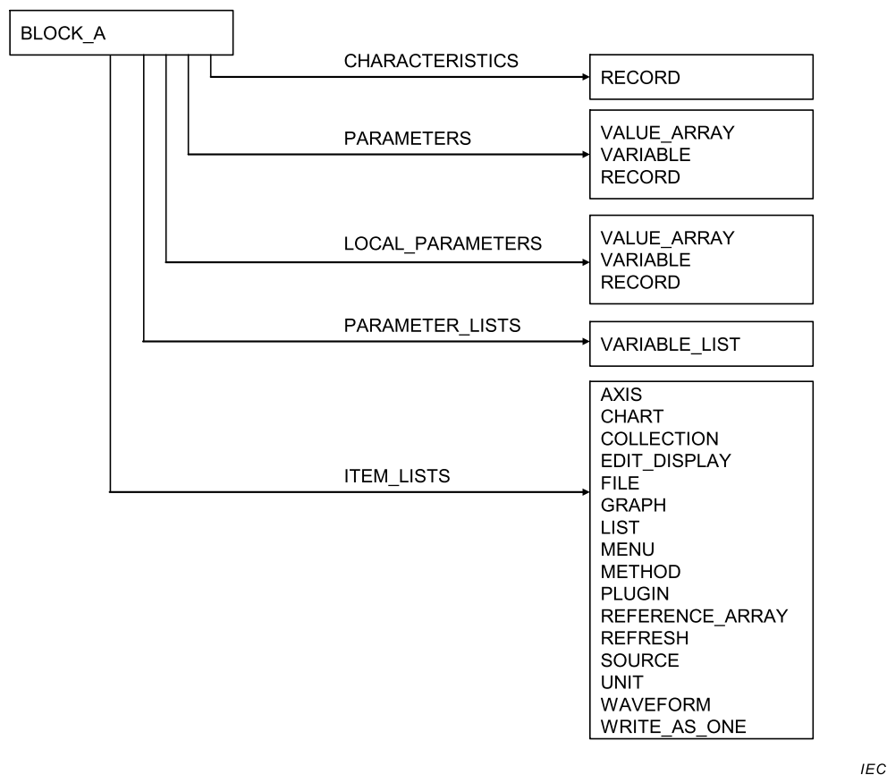
Figure 3 – BLOCK_A
