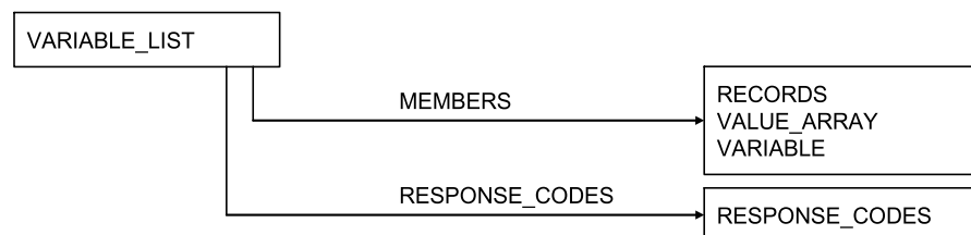
Figure 27 – VARIABLE_LIST
