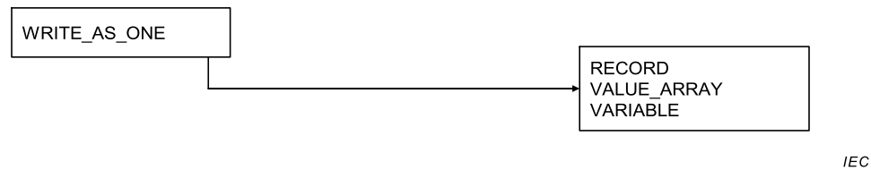
Figure 23 – WRITE_AS_ONE
