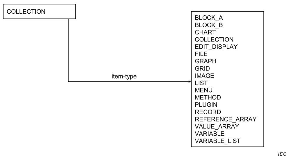
Figure 5 – COLLECTION
