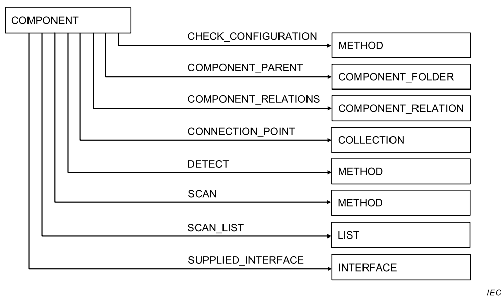
Figure 7 – COMPONENT
