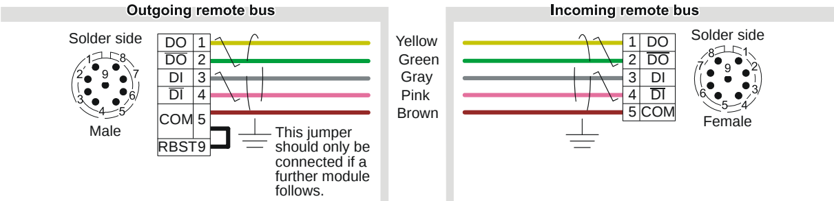
Figure A.4 – M23 circular connector pin assignment
