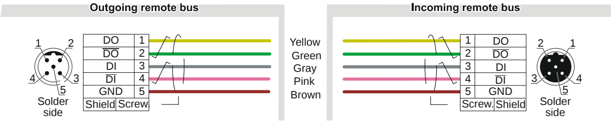
Figure A.5 – M12 circular connector pin assignment
