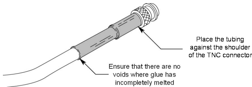
Figure A.43 – Sealed IP65/67 cable
