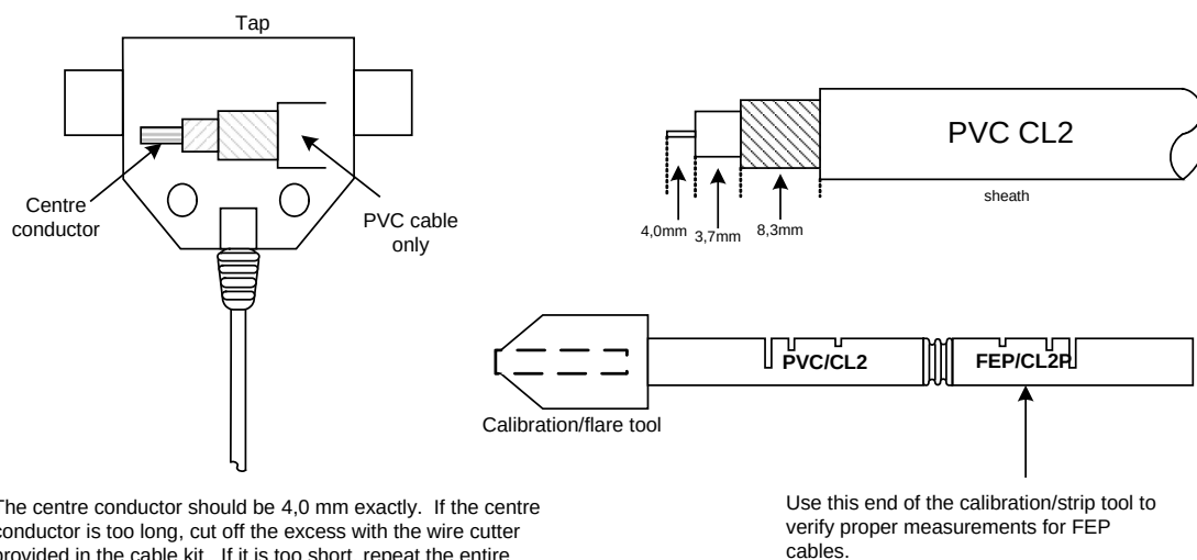
Figure A.35 – Strip guides
