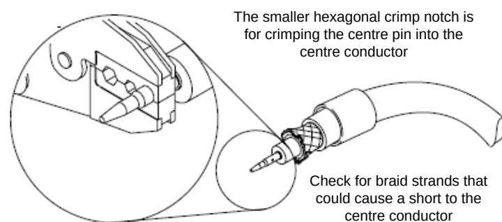
Figure A.39 – Crimping the centre pin
