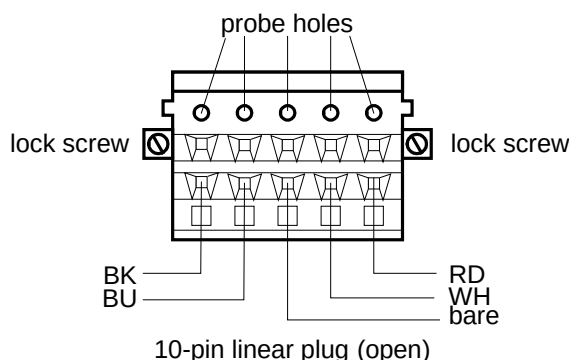
Figure C.10 – Open-style connector pin out 10 position
