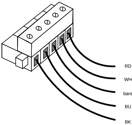
Figure C.30 – Open-style connector (female)
