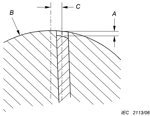
Figure 3 – Interface dimension of the end-face contact zone
