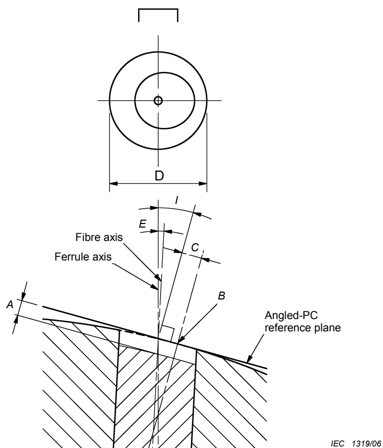
Figure 1 – Interface dimensions
