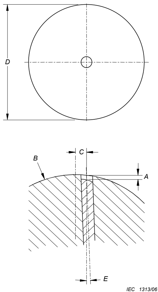
Figure 1 – Interface dimensions
