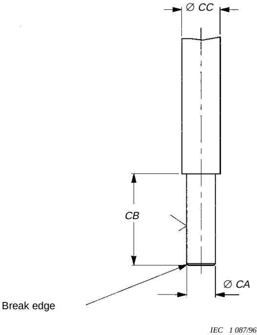
Figure 2b – Gauge pin for resilient alignment sleeve
