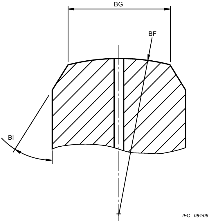
Figure 2 – Plug connector interface – Expanded view A (see Tables 1 and 2 for dimensions)
