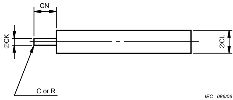
Figure 6 – Pin gauge for active device receptacle (see Table 7)
