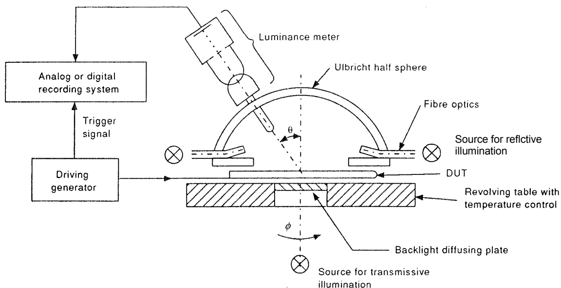
Figure B.2 – Example of system for measuring diffused light contrast ratio
