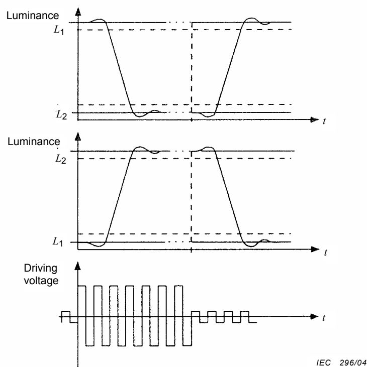
Figure B.4 – Typical examples of dynamic responses of two different LCDs
