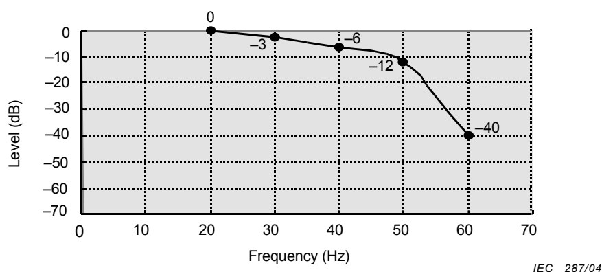
Figure 6 – Frequency characteristics of the integrator (response of human visual system)
