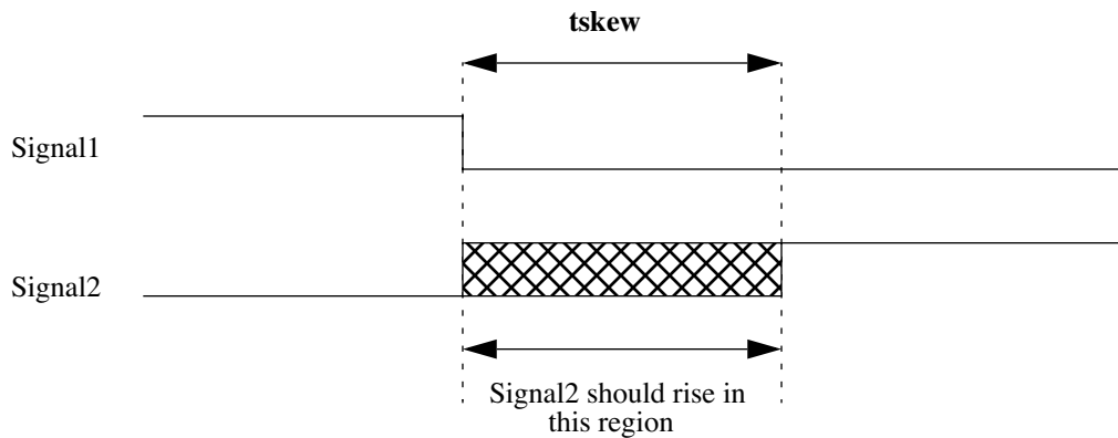
Figure 5—Out-of-phase skew check
