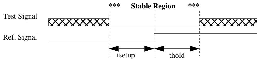
Figure 2—Setup/hold check for positive constraints
