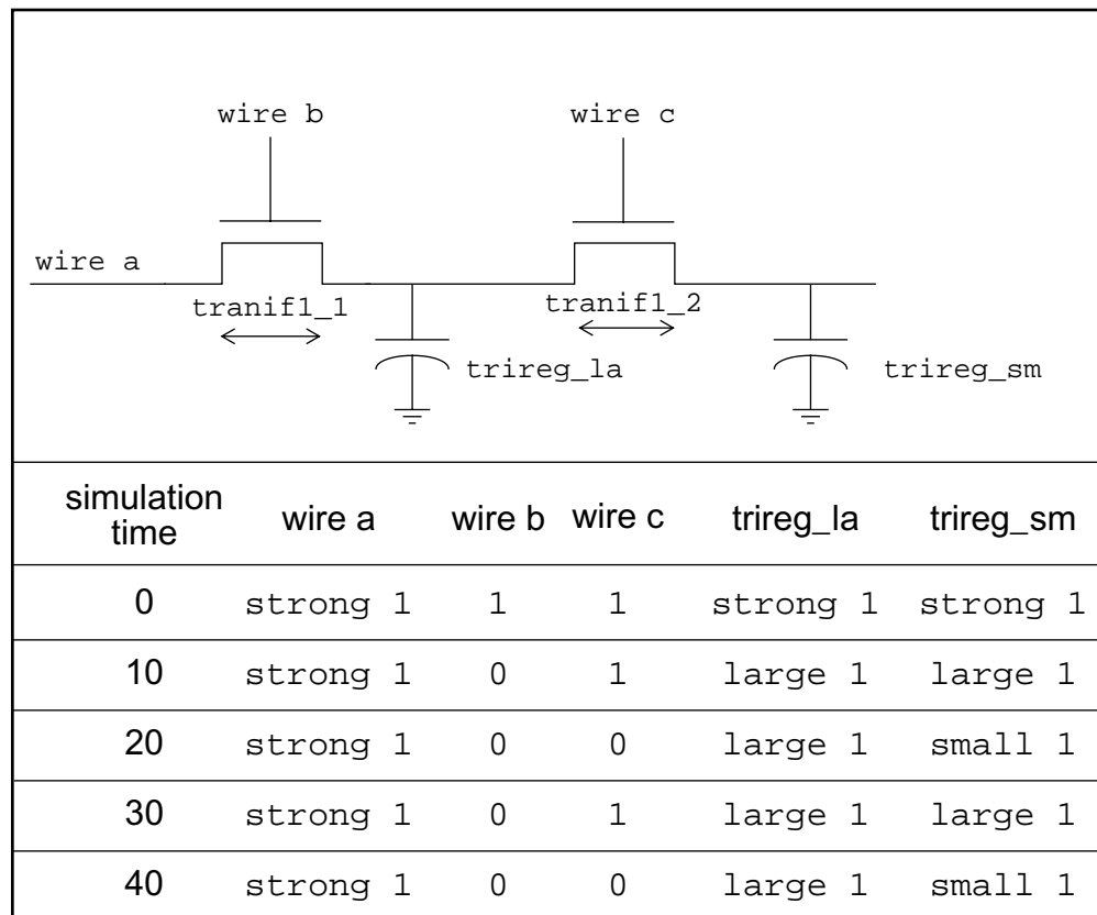
Figure 3—Simulation results of charge sharing
