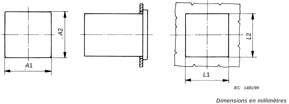
Figure 1 – Boîtier carré
