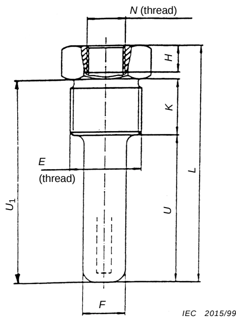
Figure 3 – Type B – External configuration
