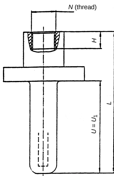
Figure 5 – Type C – External configuration
