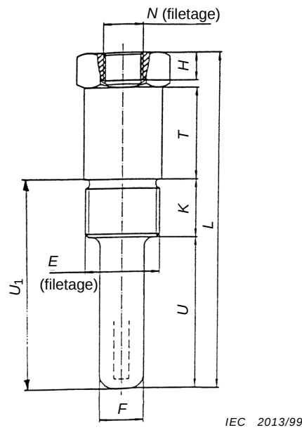
Figure 1 – Type A – Configuration extérieure
