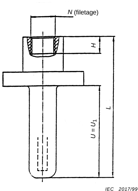
Figure 5 – Type C – Configuration extérieure
