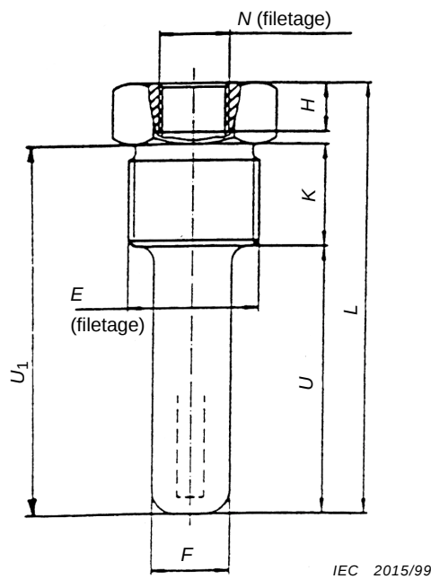
Figure 3 – Type B – Configuration extérieure
