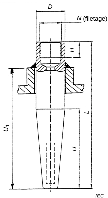
Figure 7 – Type D – Configuration extérieure
