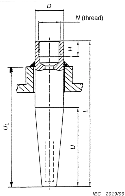
Figure 7 – Type D – External configuration
