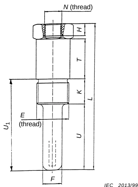
Figure 1 – Type A – External configuration
