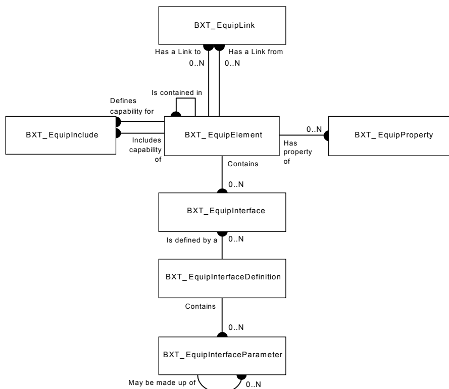
Figure 18 – Equipment information exchange tables
