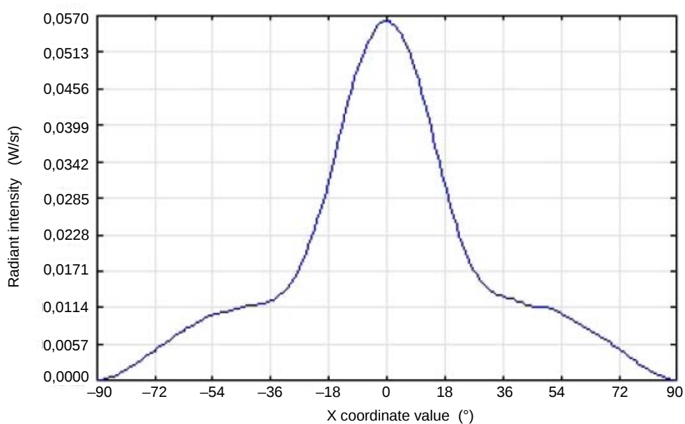
Figure 14 – Example of intensity distribution of emitting element
