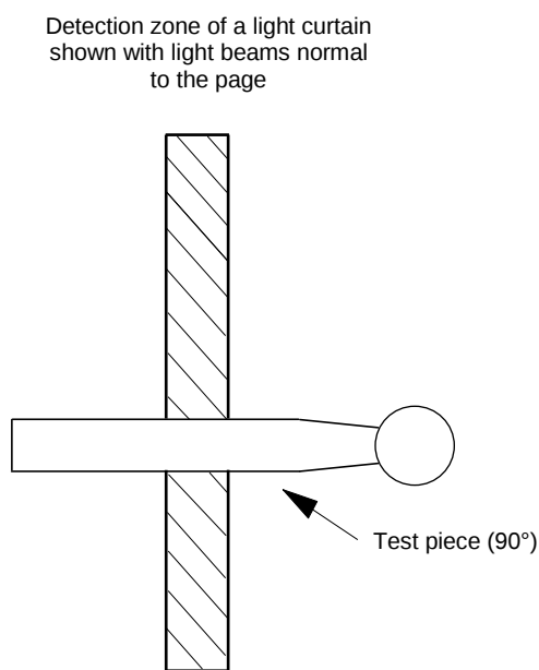
Figure 4 – Test piece at 90°
