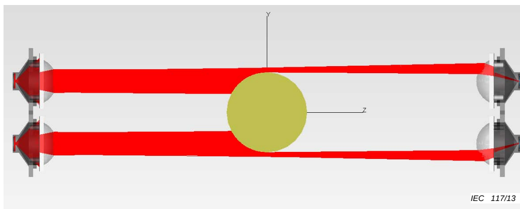
Figure 17 – Example of test piece inside model of optical subsystem with passing radiation on the receiver
