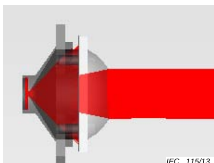
Figure 15 – Example of emitter model with beams internally blocked by aperture stop
