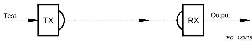
Figure AA.1 – Single beam sensing device
