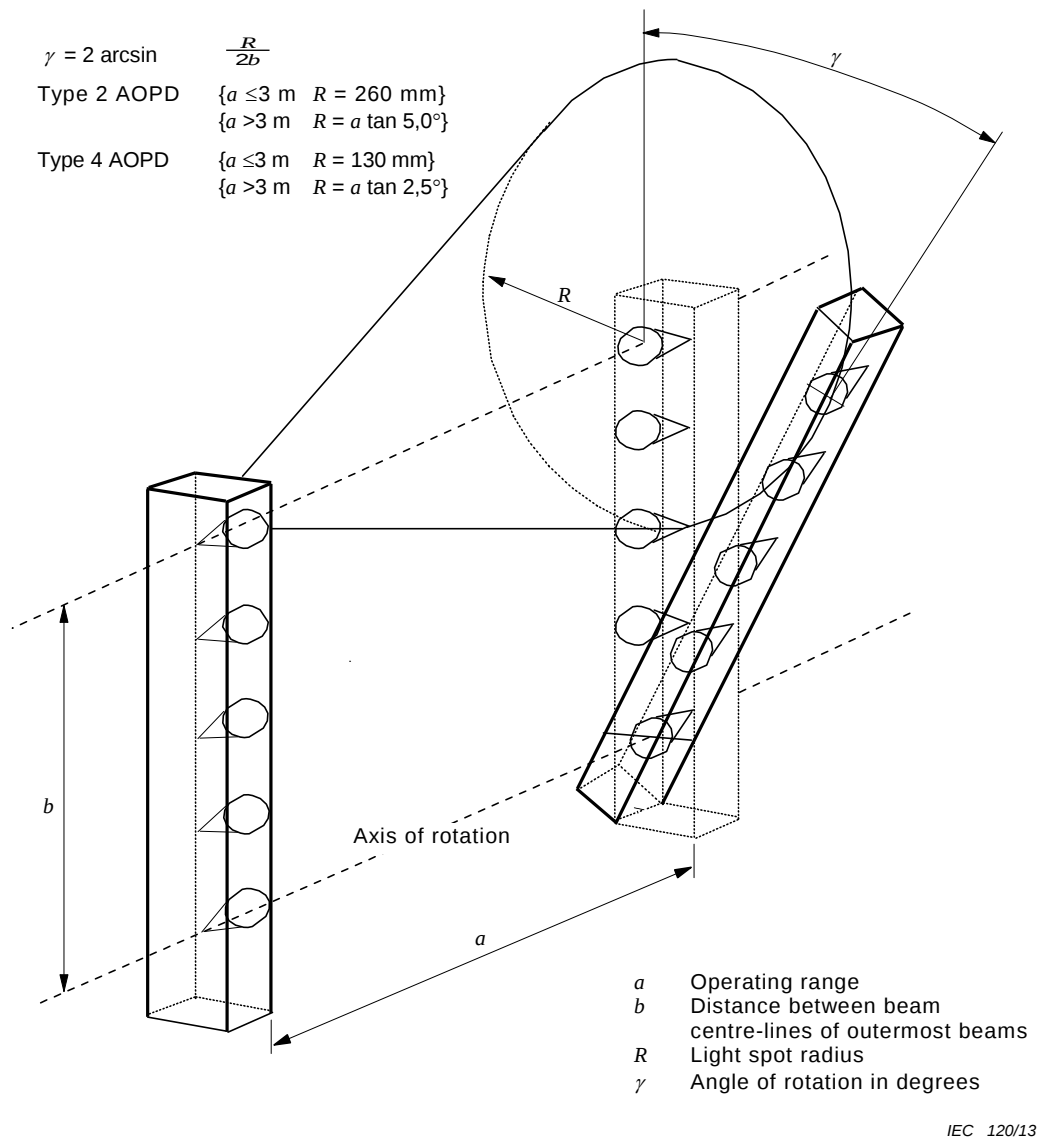
Figure 20 – AOPD misalignment test
