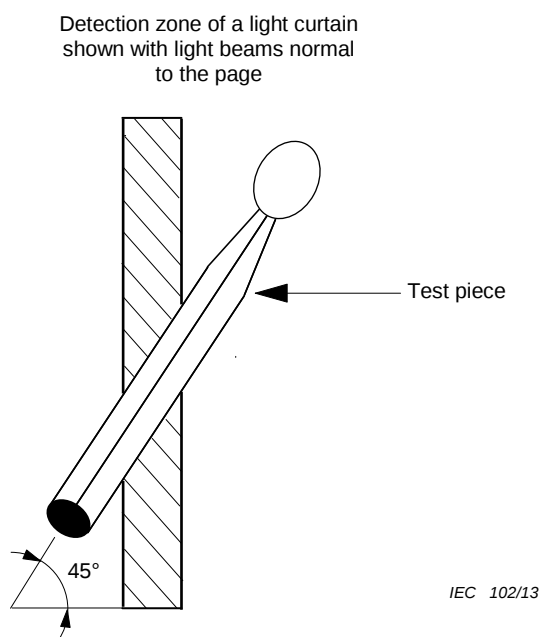
Figure 3 – Test piece at 45°
