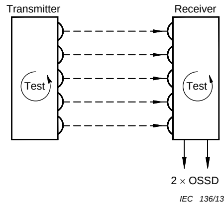
Figure AA.4 – Example of type 2 AOPD with internal test
