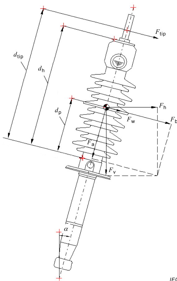
Figure D.2 – Forces affecting the bushing
