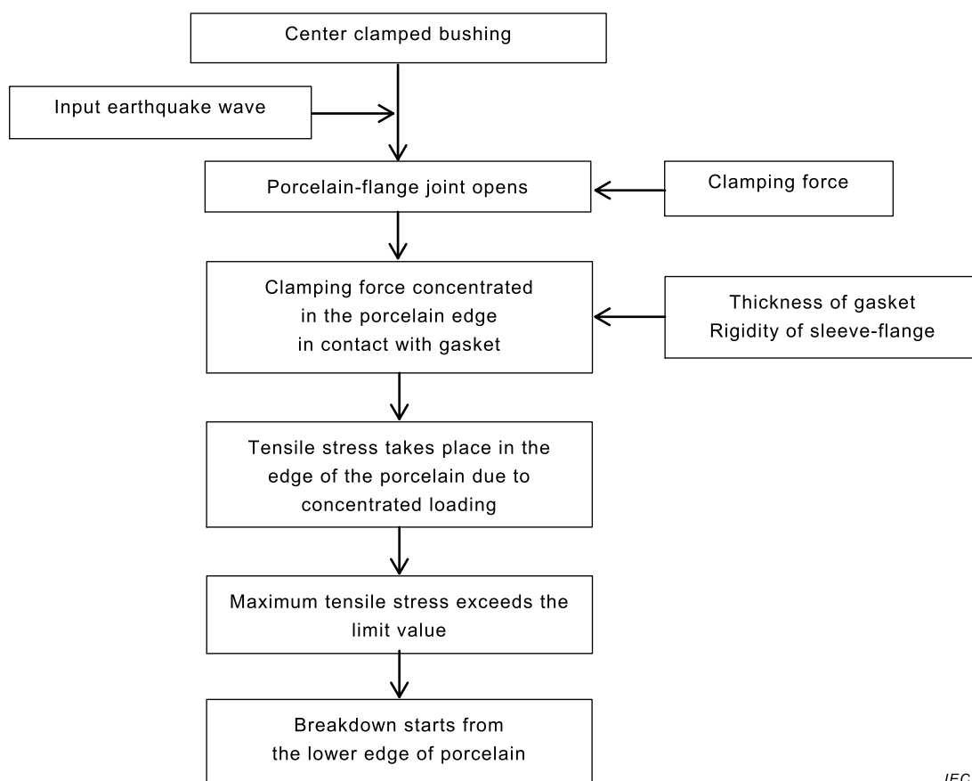
Figure E.2 – Failure process, flow chart [5] [6]
