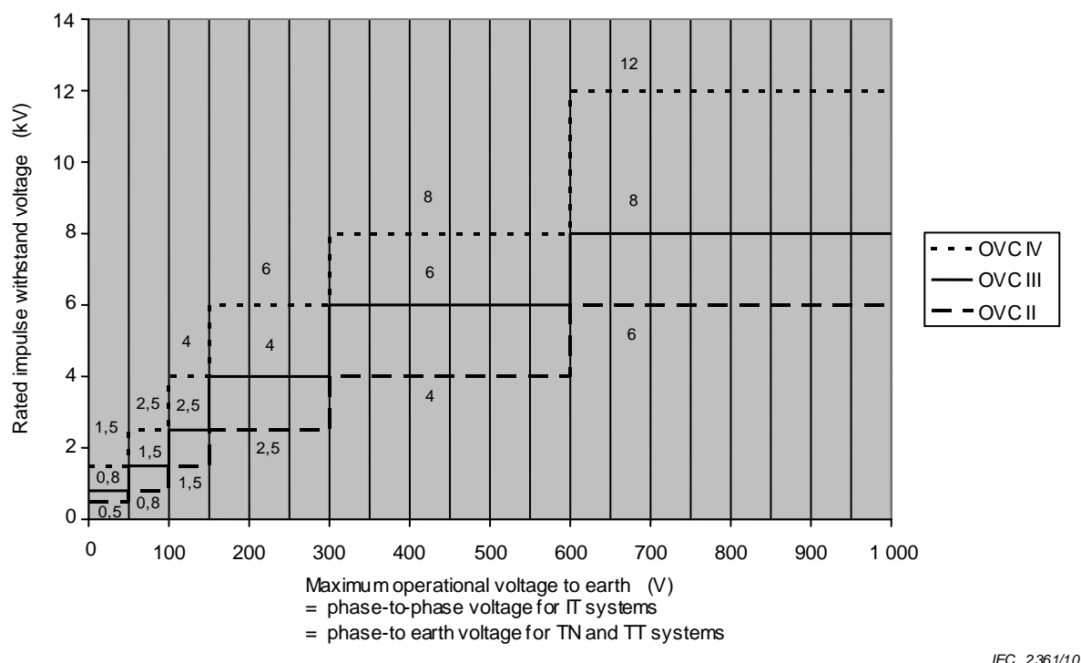
Figure 1 – Required rated impulse withstand voltage
