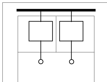
Form 3b: Terminals and external conductors separated from busbars IEC 1716/11
