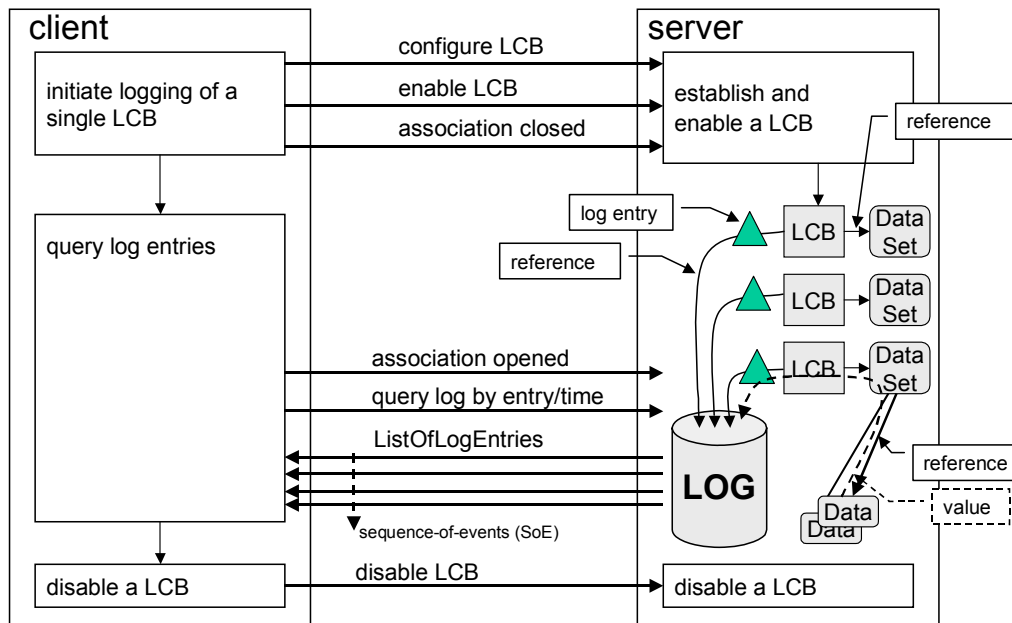
Figure 7 – Log control block – conceptual
