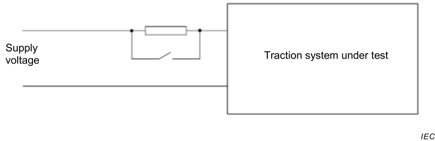
Figure 19 – Example of method to create a rapid voltage change
