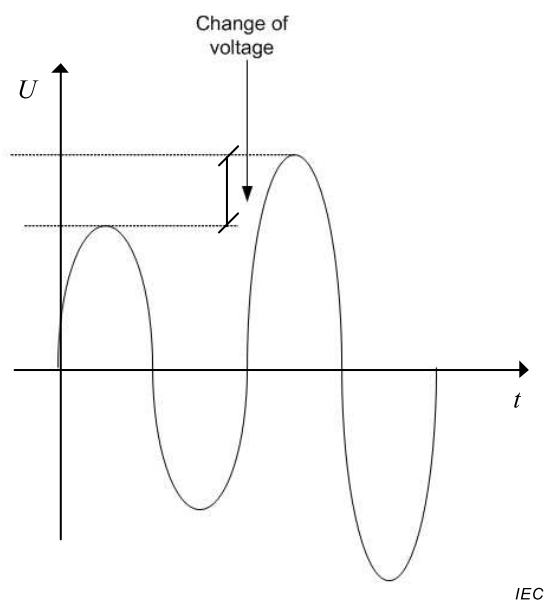
Figure 18 – Rapid voltage change with AC line voltage
