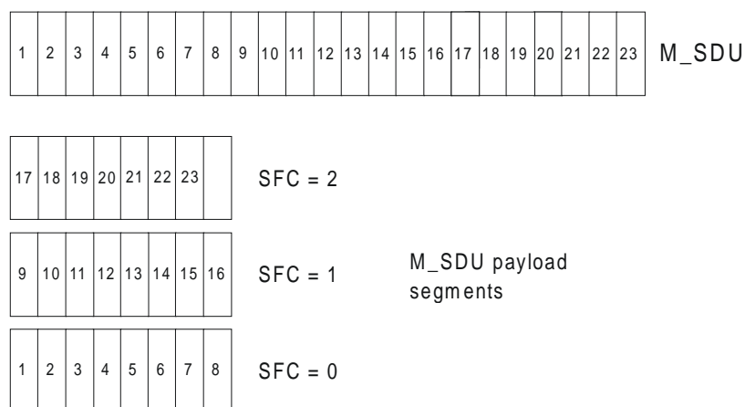
Figure 7 – Example segmentation of M_SDU
