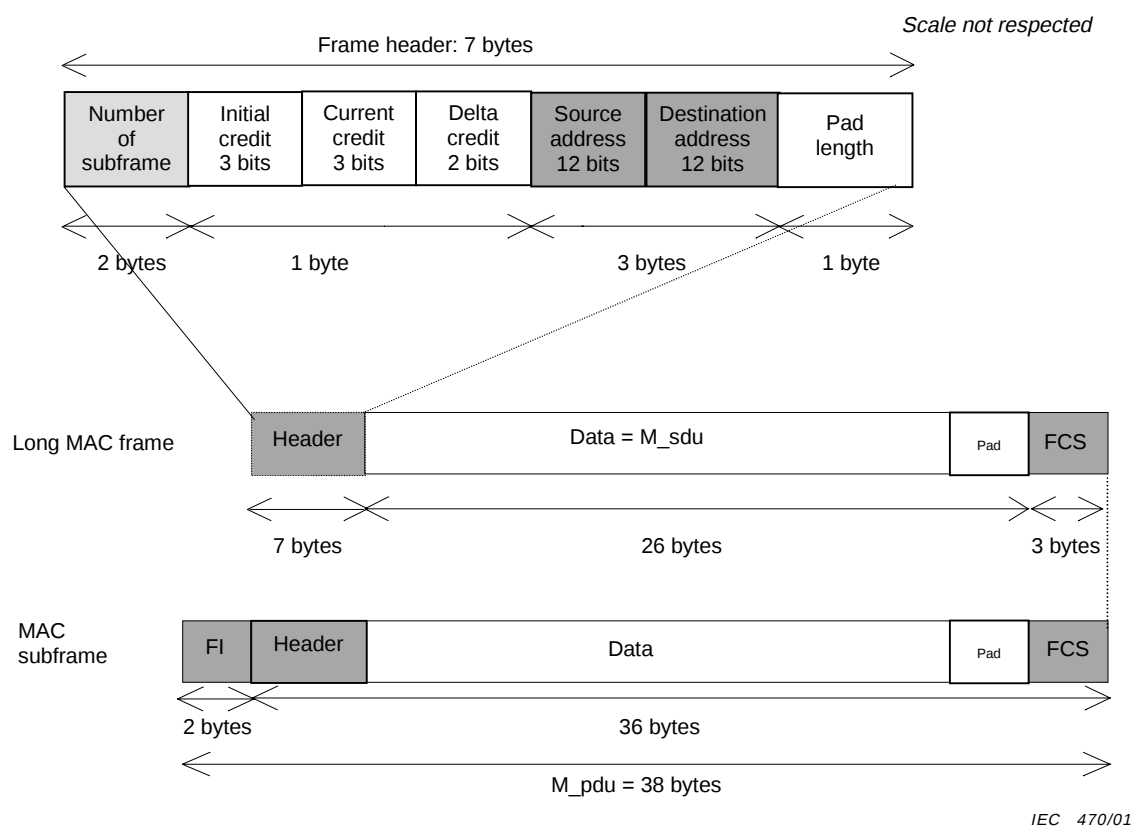
Figure 8 – Long MAC frame made of one subframe only
