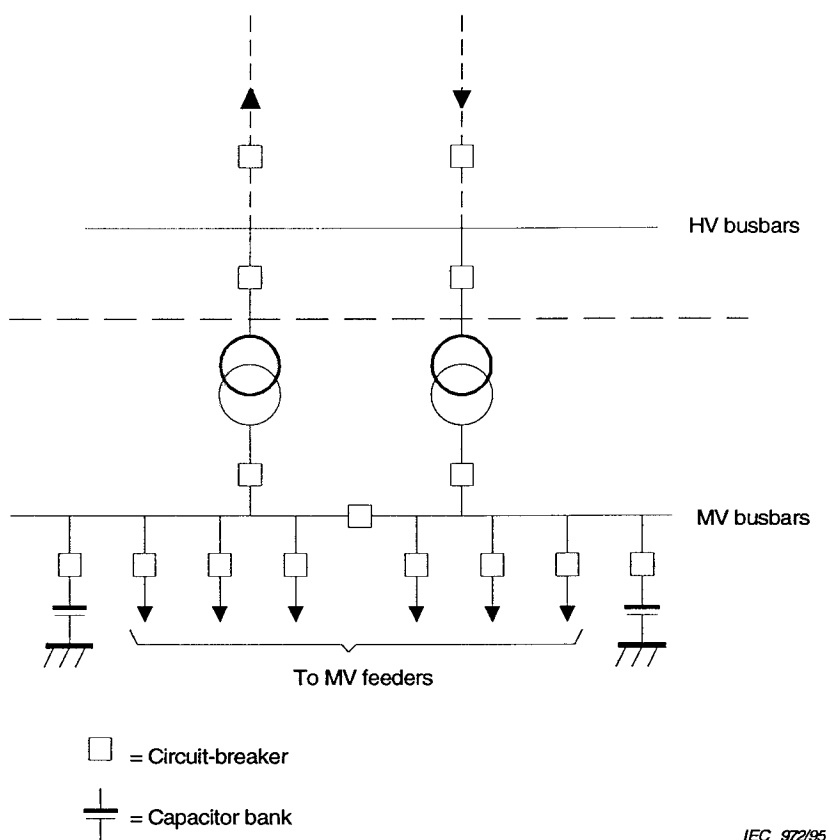
Figure 1 – Typical diagram of an HV/MV substation
