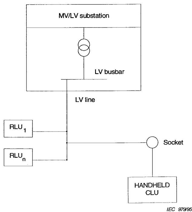
Figure 8 – Local reading via the mains
