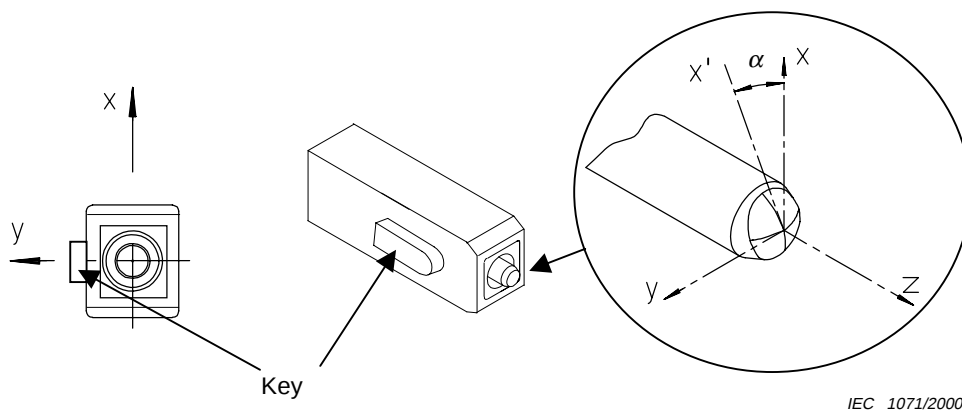
Figure 2 – Preferred orientation of the adjustment sector for some constructions – Example of angled connector scheme
