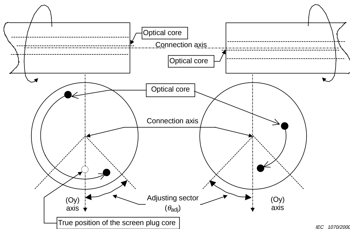
Figure 1 – Adjusting sector and reference plug true position
